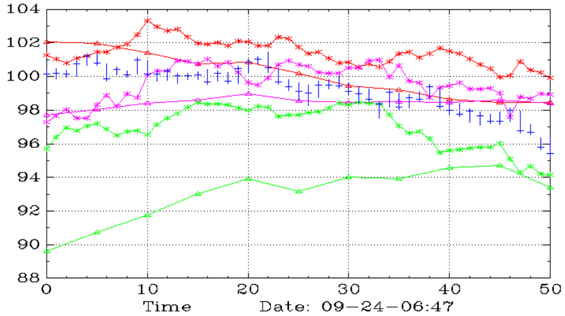
AGG (Monthly,Weekly)
