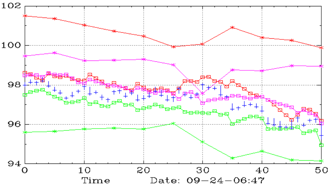
AGG (Weekly,Daily)
