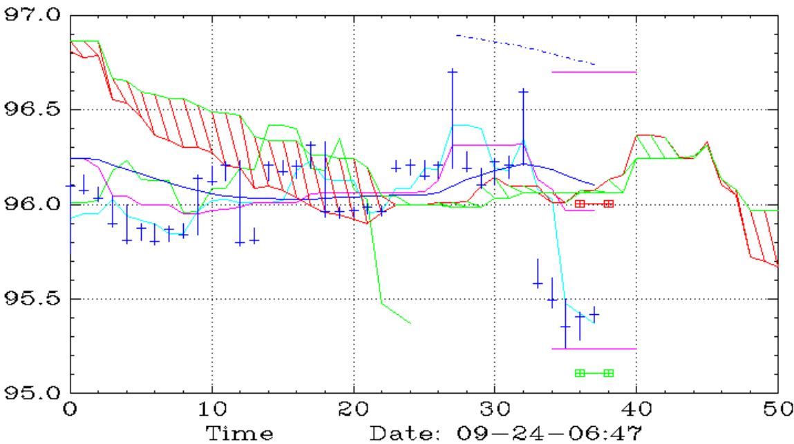
AGG (90,Ichimoku)
