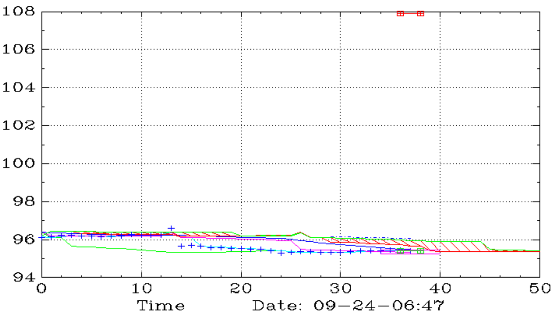
AGG (15,Ichimoku)
