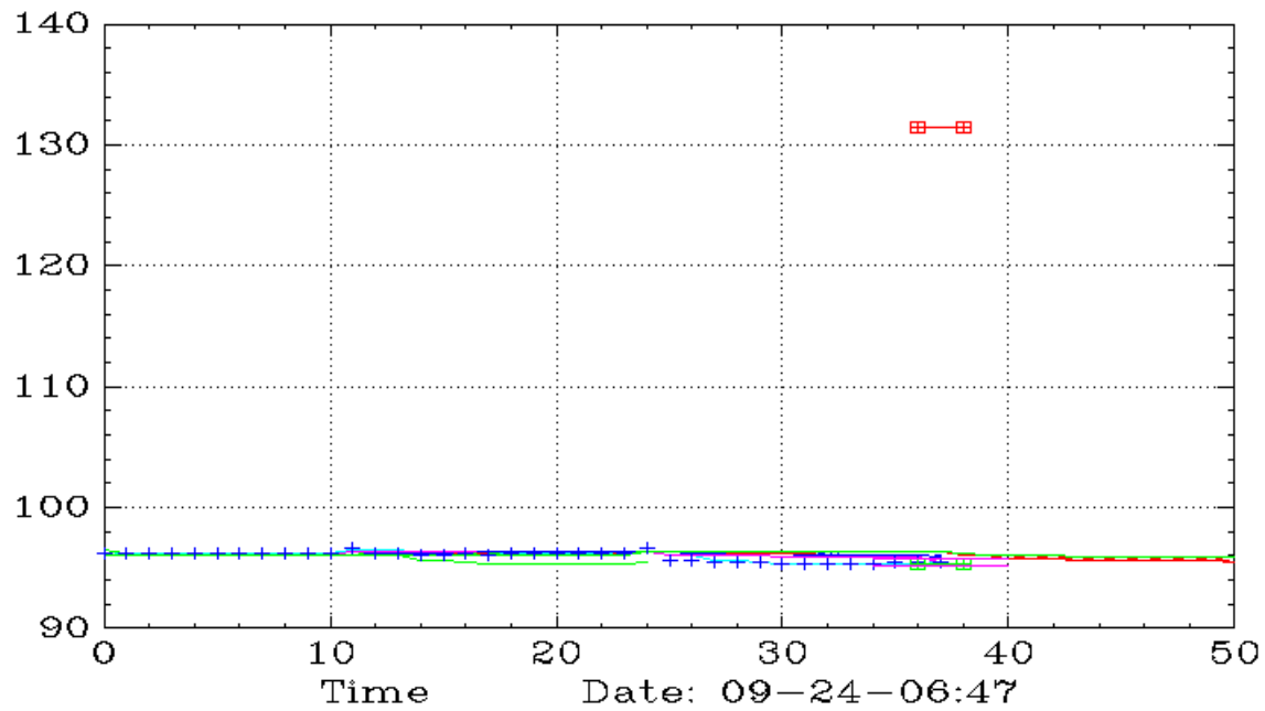
AGG (30,Ichimoku)
