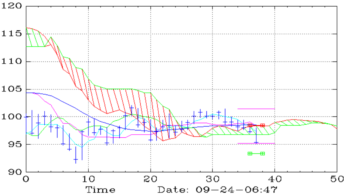
AGG (Monthly,Ichimoku)
