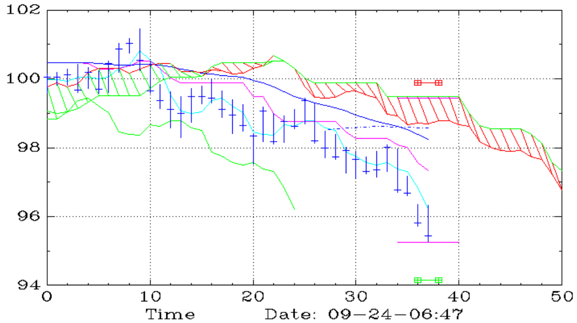
AGG (Weekly,Ichimoku)
