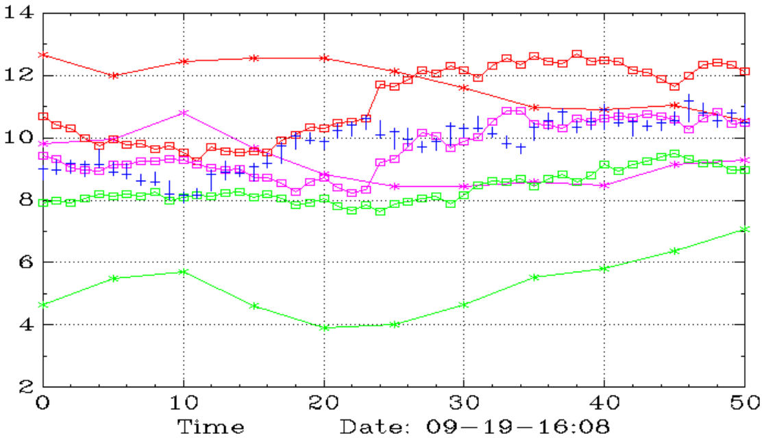
AI (Weekly,Daily)
