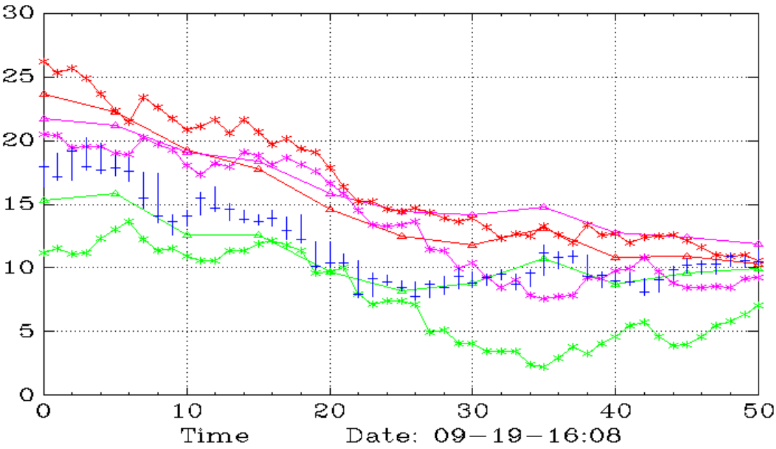
AI (Monthly,Weekly)
