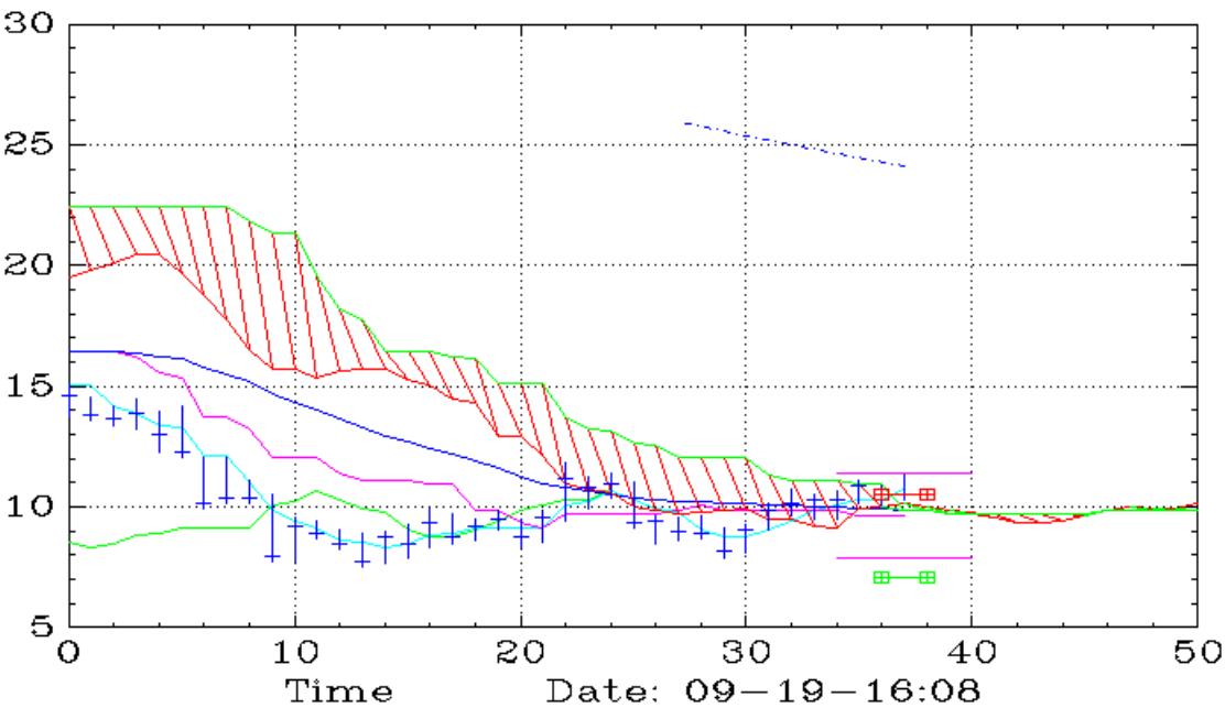
AI (Weekly,Ichimoku)
