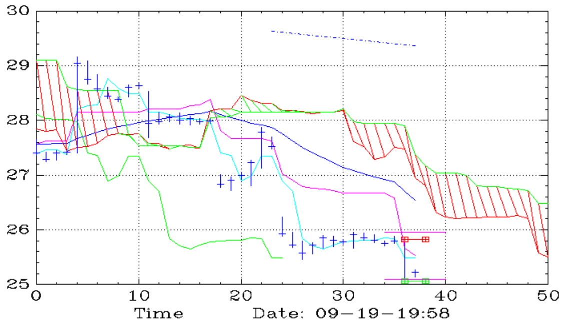
AMDD (60,Ichimoku)
