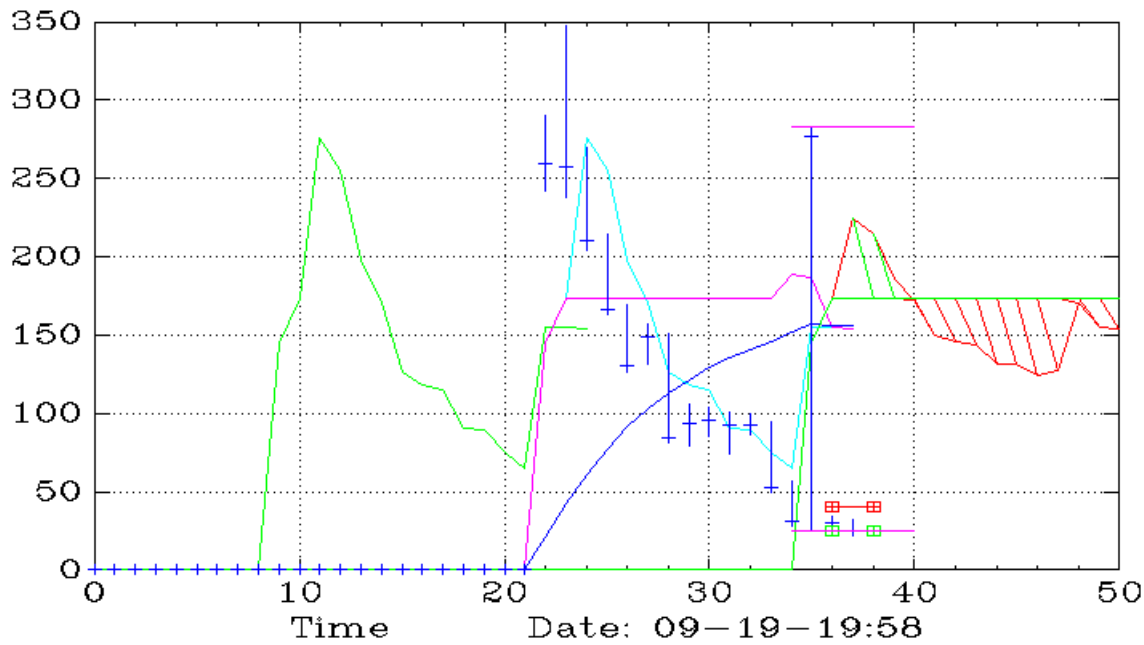
AMDD (Monthly,Ichimoku)
