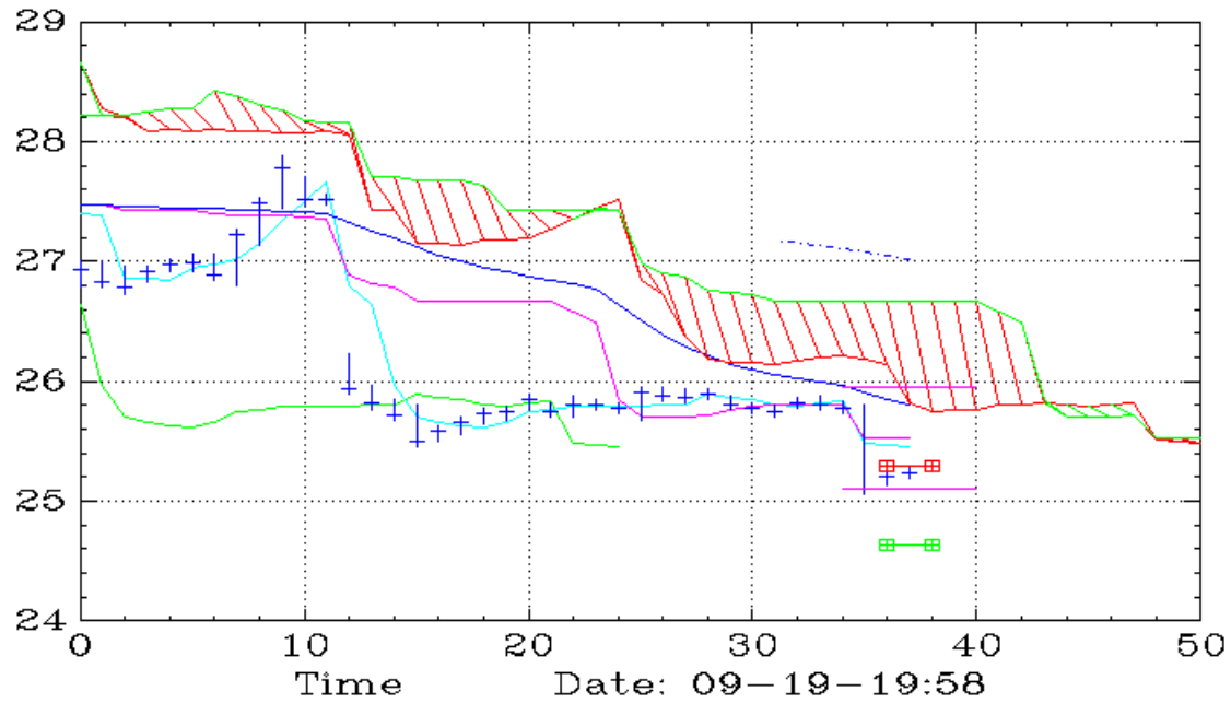
AMDD (30,Ichimoku)
