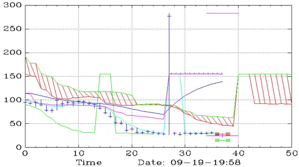
AMDD (Weekly,Ichimoku)
