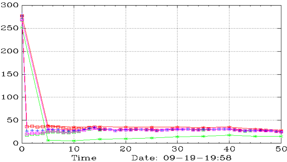
AMDD (Weekly,Daily)
