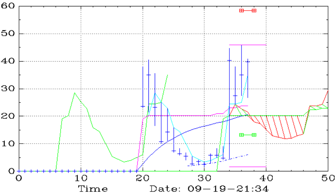
AXTU (Weekly,Ichimoku)
