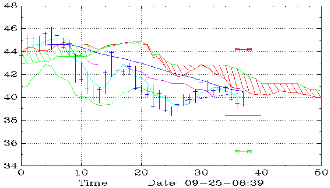
BKF (Weekly,Ichimoku)
