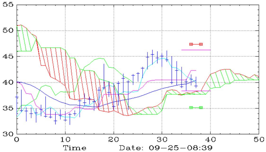
BKF (Monthly,Ichimoku)
