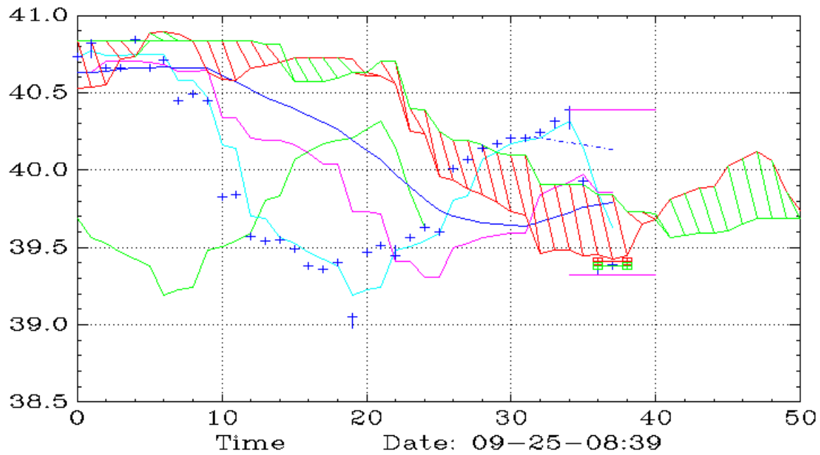
BKF (30,Ichimoku)
