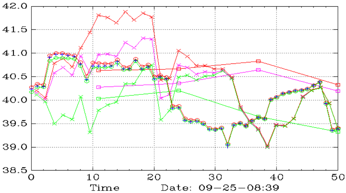
BKF (Daily,45,30)
