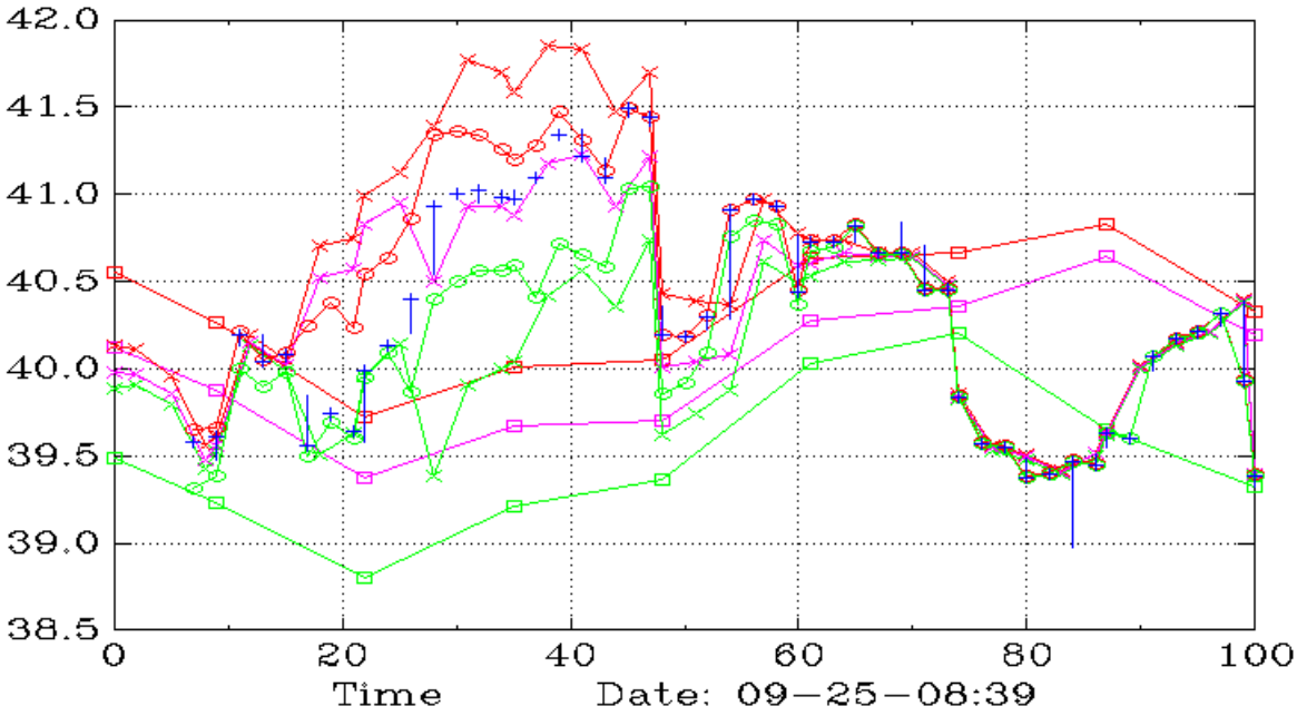
BKF (Daily,90,60)
