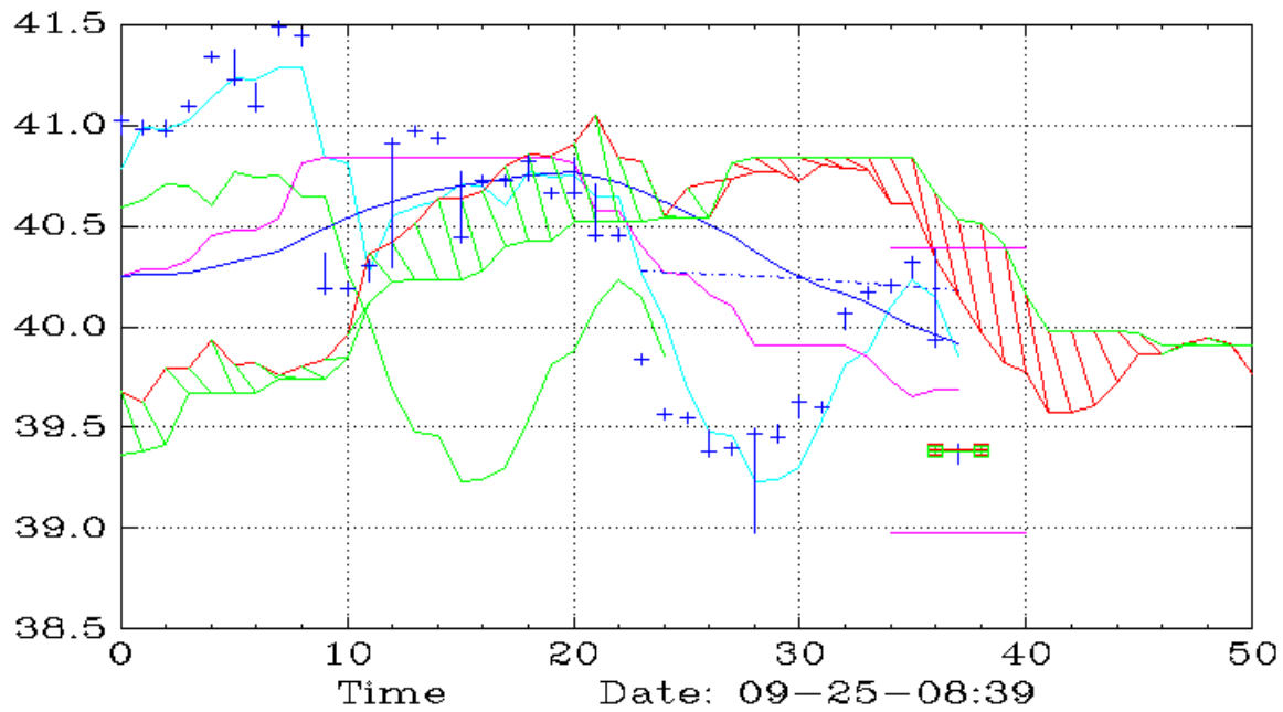
BKF (60,Ichimoku)
