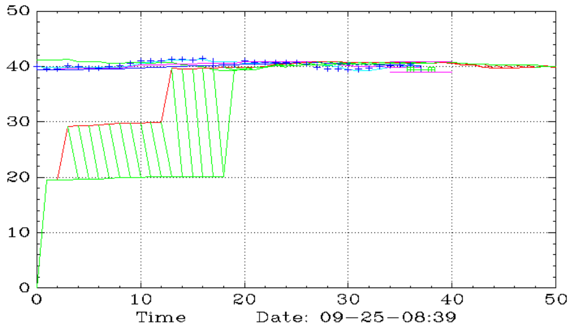
BKF (90,Ichimoku)
