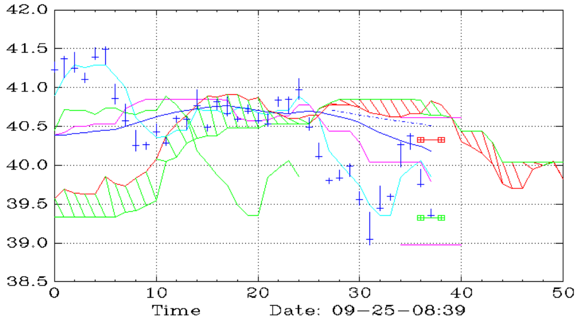
BKF (Daily,Ichimoku)
