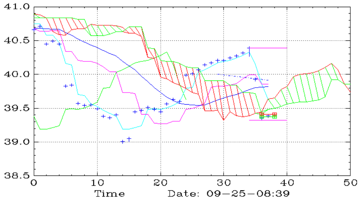
BKF (15,Ichimoku)
