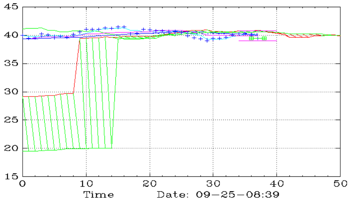
BKF (45,Ichimoku)
