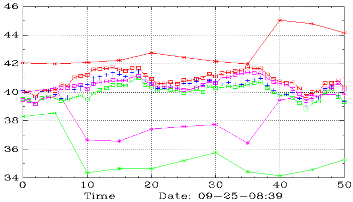
BKF (Weekly,Daily)
