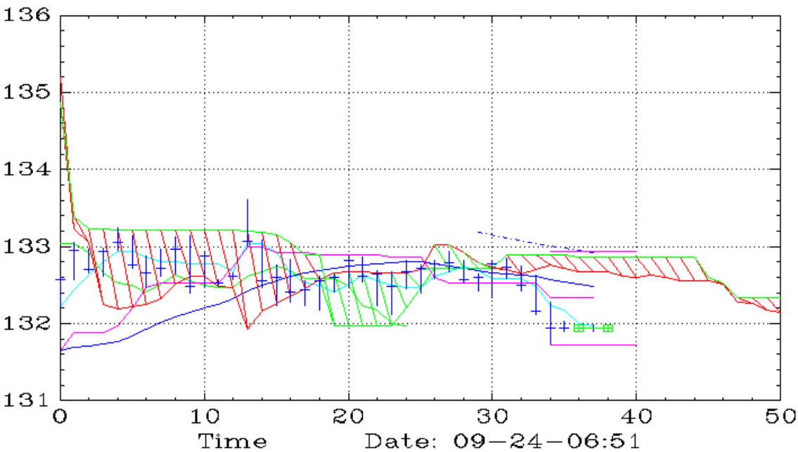
C (15,Ichimoku)
