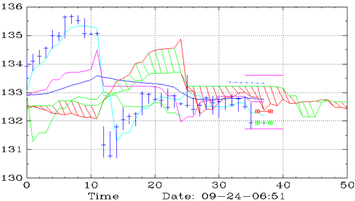
C (30,Ichimoku)
