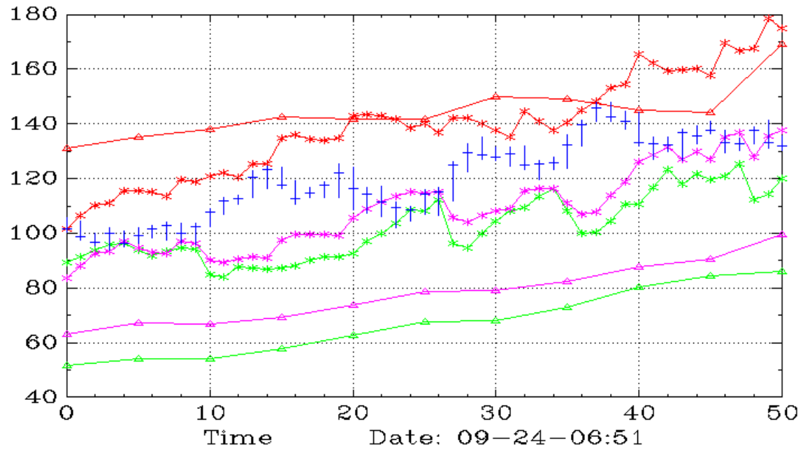
C (Monthly,Weekly)
