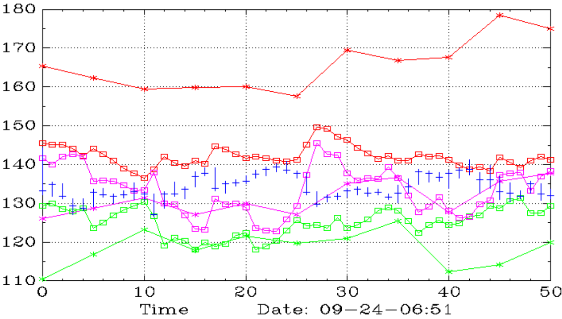
C (Weekly,Daily)
