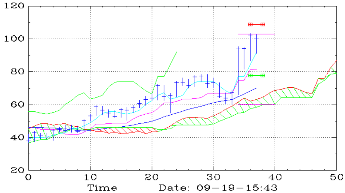
CIBR (Monthly,Ichimoku)
