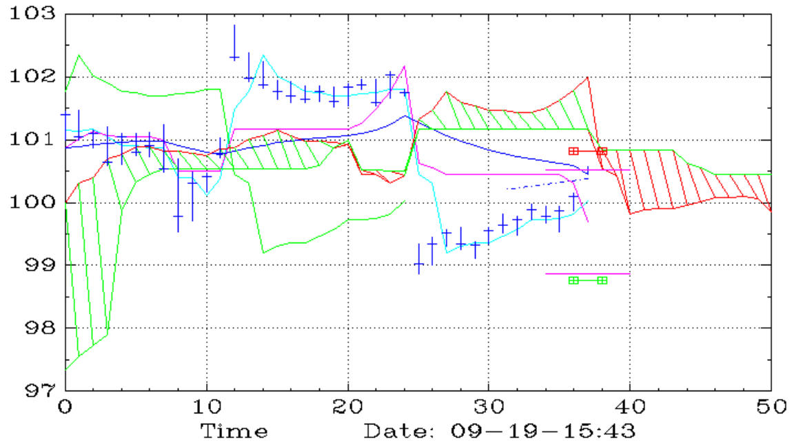
CIBR (30,Ichimoku)
