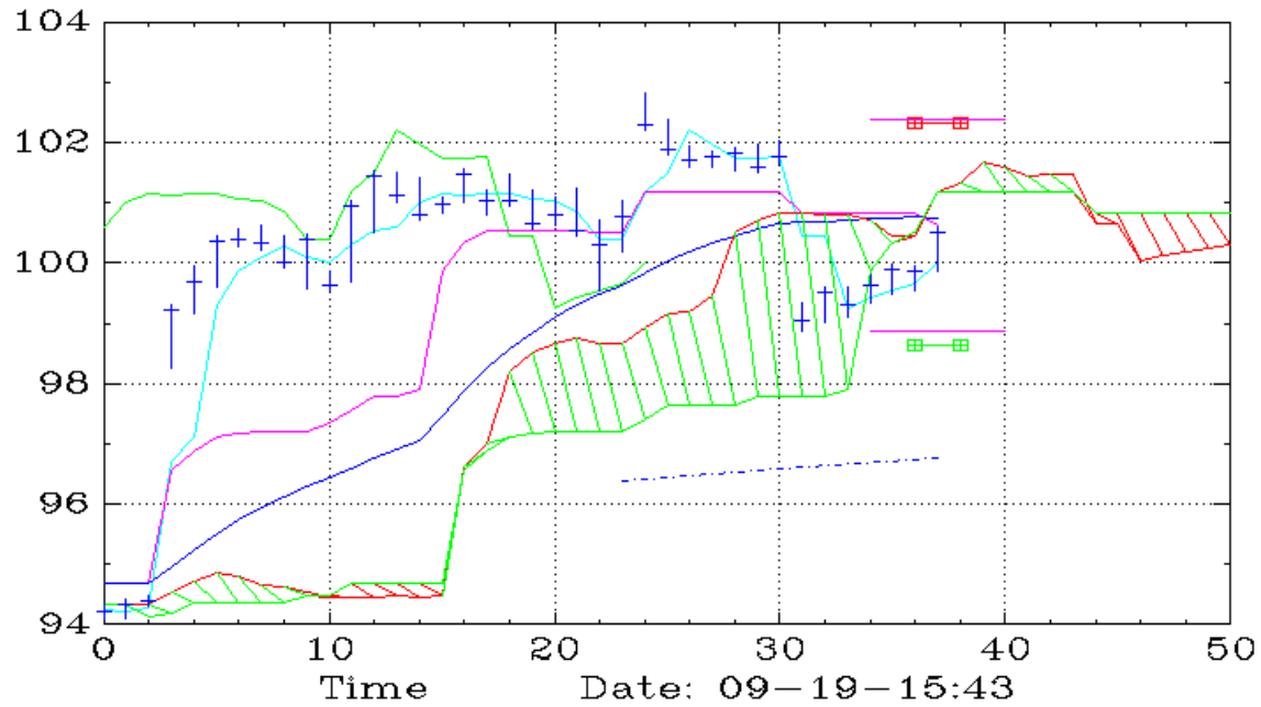
CIBR (60,Ichimoku)
