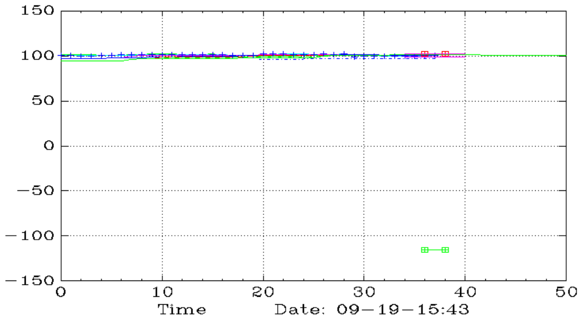
CIBR (45,Ichimoku)
