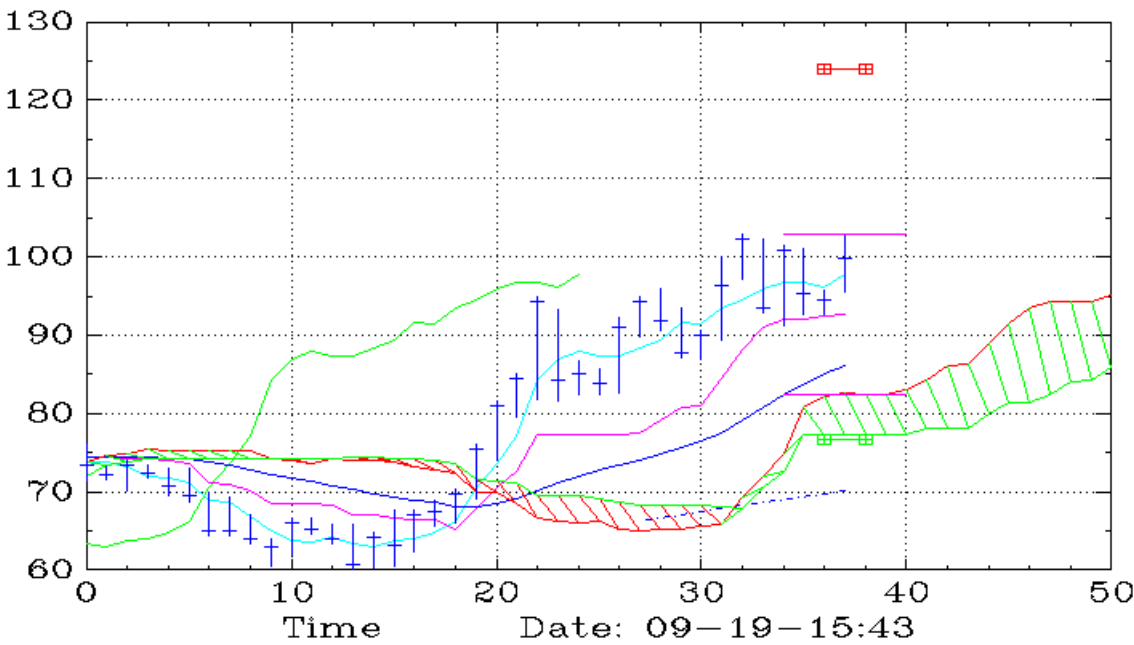
CIBR (Weekly,Ichimoku)
