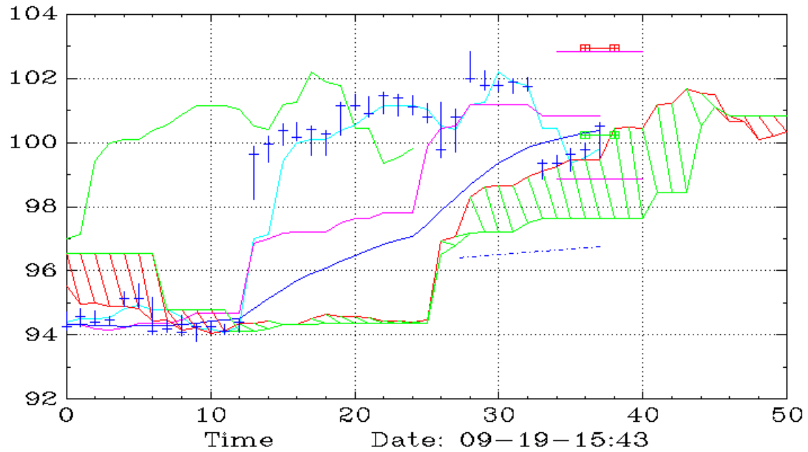
CIBR (90,Ichimoku)
