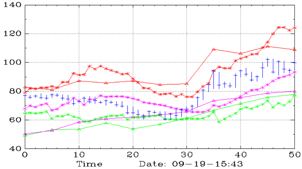
CIBR (Monthly,Weekly)
