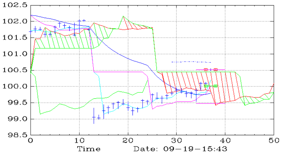
CIBR (15,Ichimoku)
