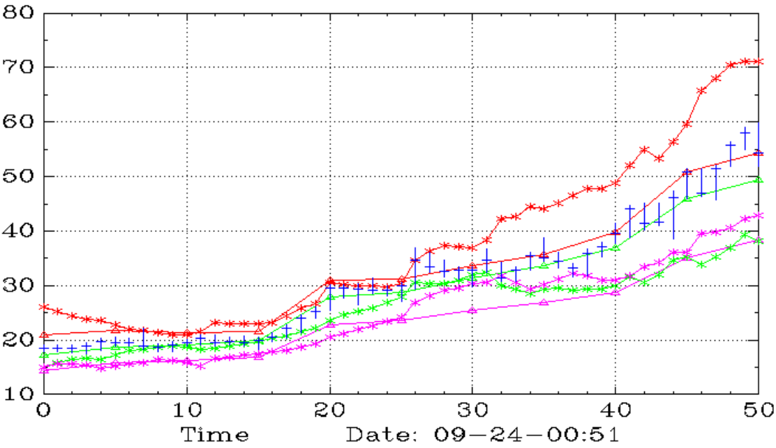
CLMT (Monthly,Weekly)
