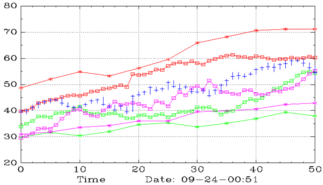
CLMT (Weekly,Daily)
