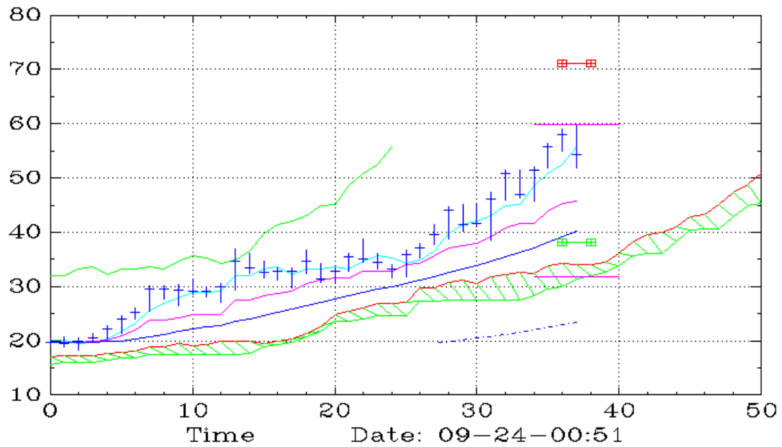
CLMT (Weekly,Ichimoku)
