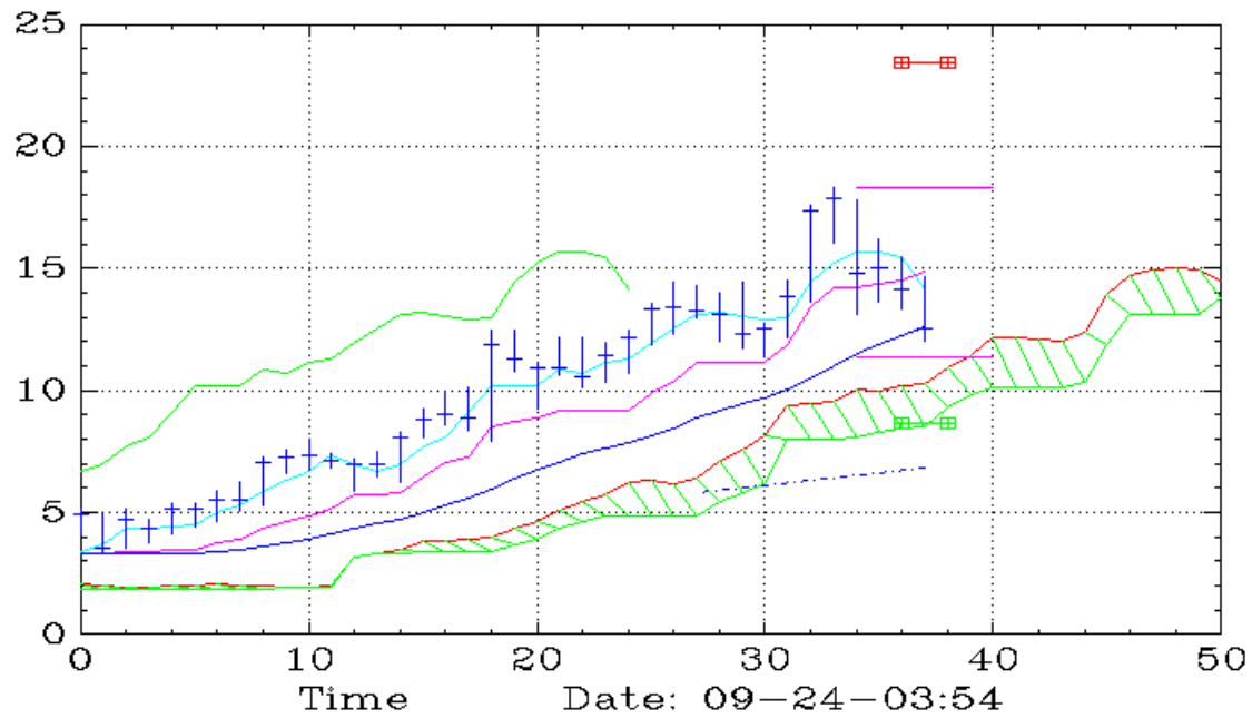
CLYM (Weekly,Ichimoku)
