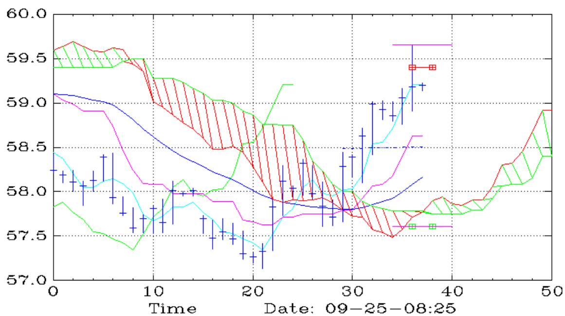
COCO (15,Ichimoku)
