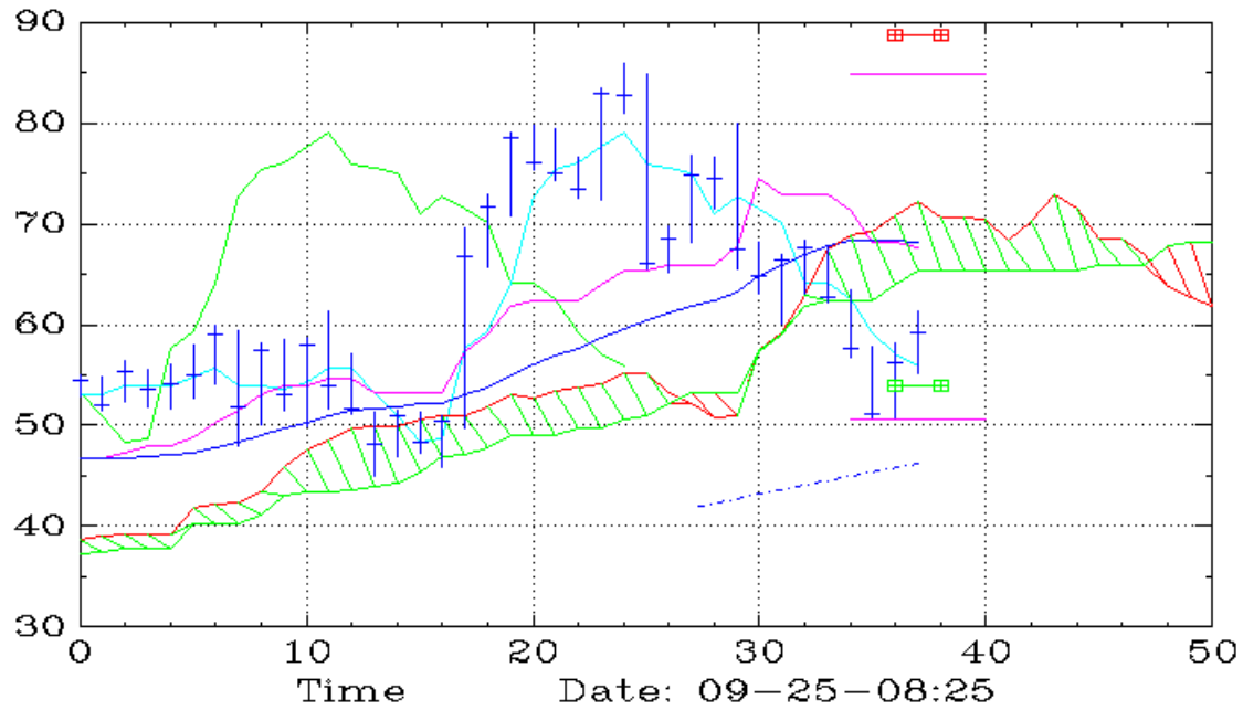
COCO (Weekly,Ichimoku)
