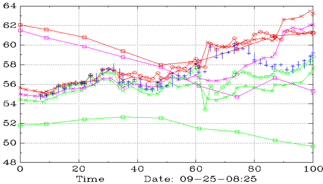
COCO (Daily,90,60)
