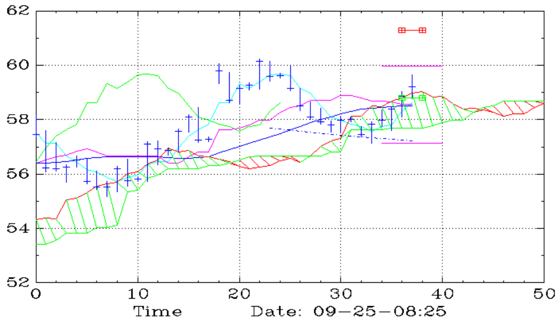
COCO (60,Ichimoku)
