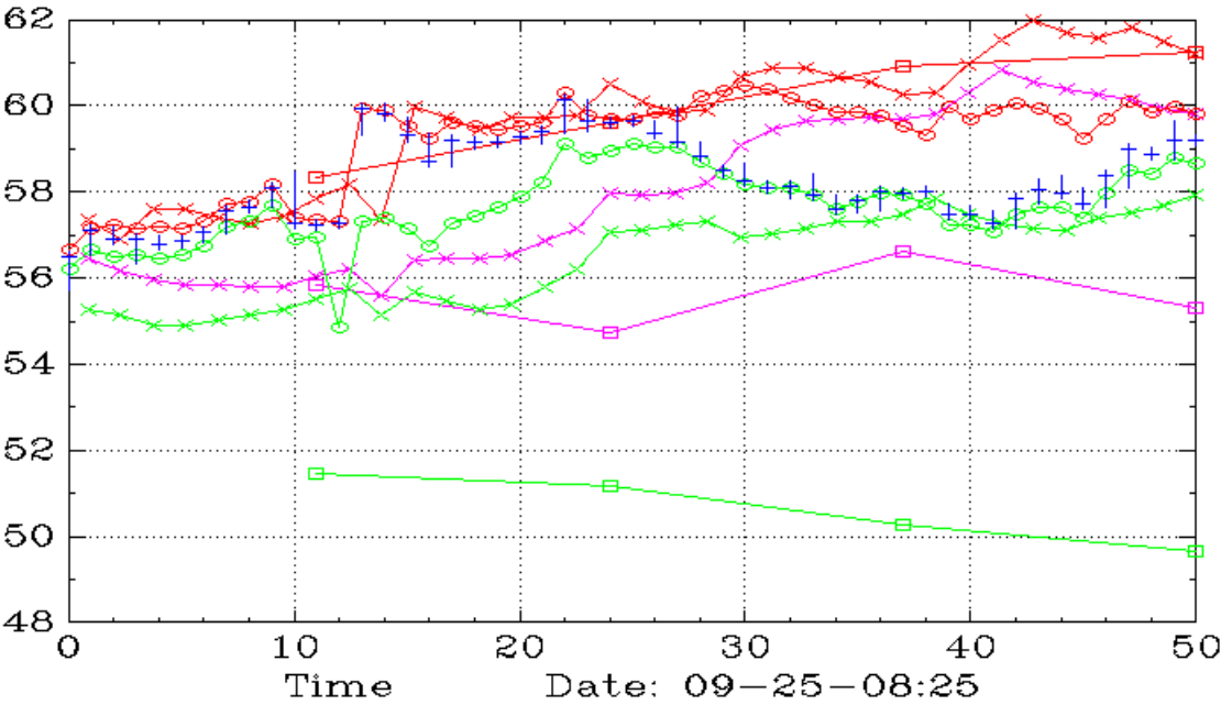
COCO (Daily,45,30)
