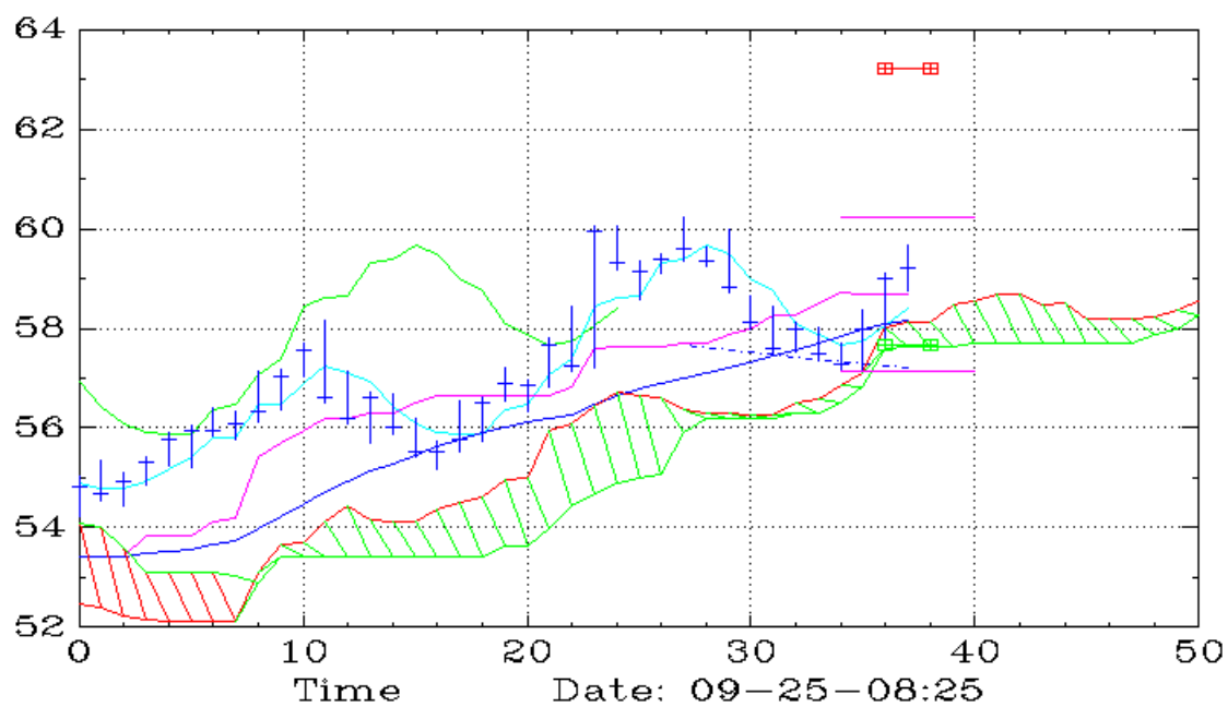
COCO (90,Ichimoku)
