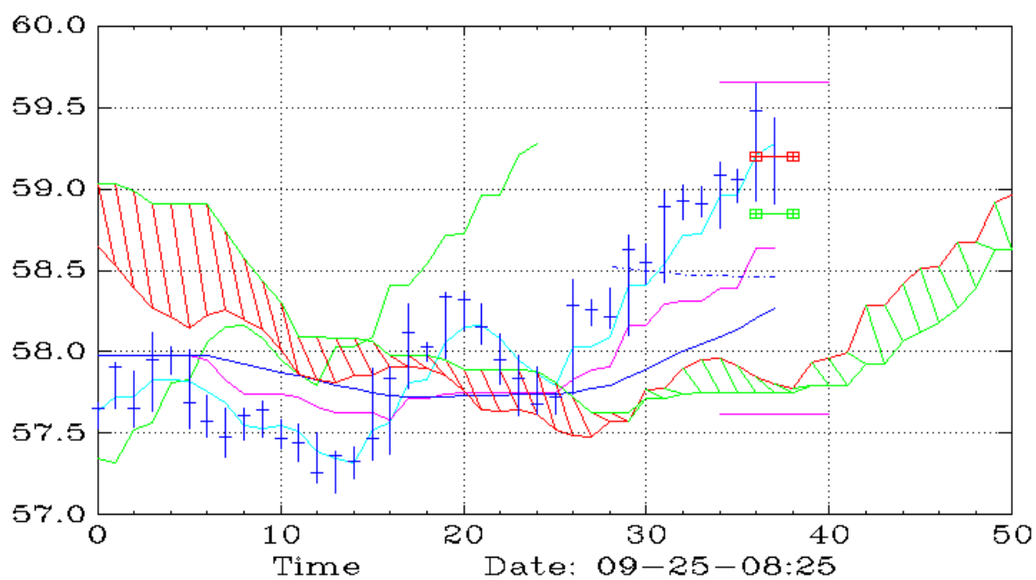
COCO (10,Ichimoku)
