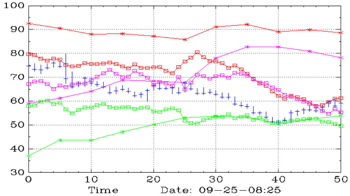
COCO (Weekly,Daily)
