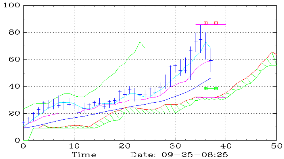
COCO (Monthly,Ichimoku)
