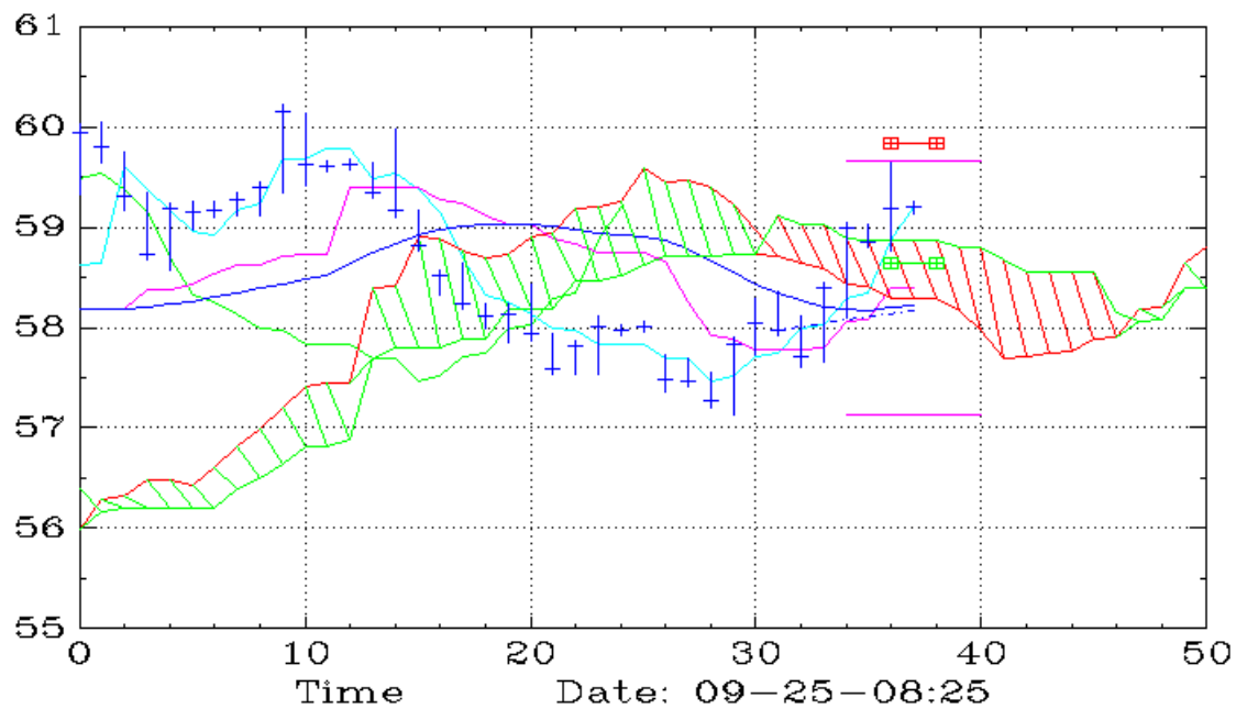
COCO (30,Ichimoku)
