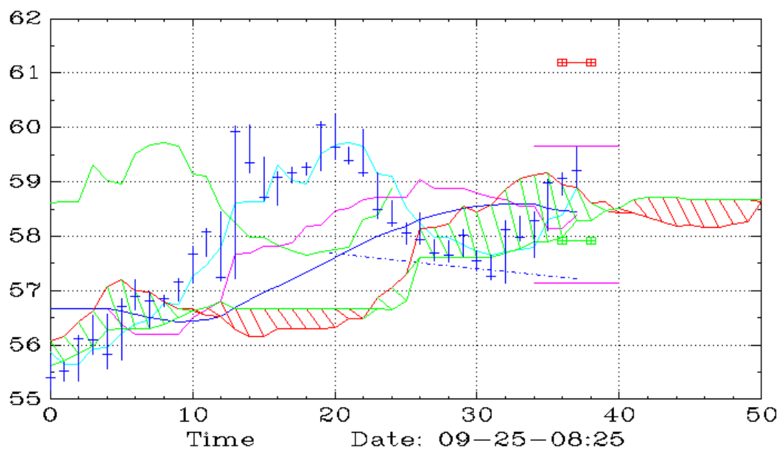
COCO (45,Ichimoku)
