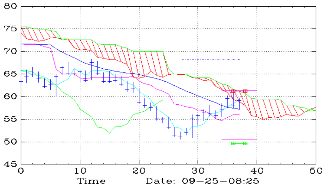
COCO (Daily,Ichimoku)
