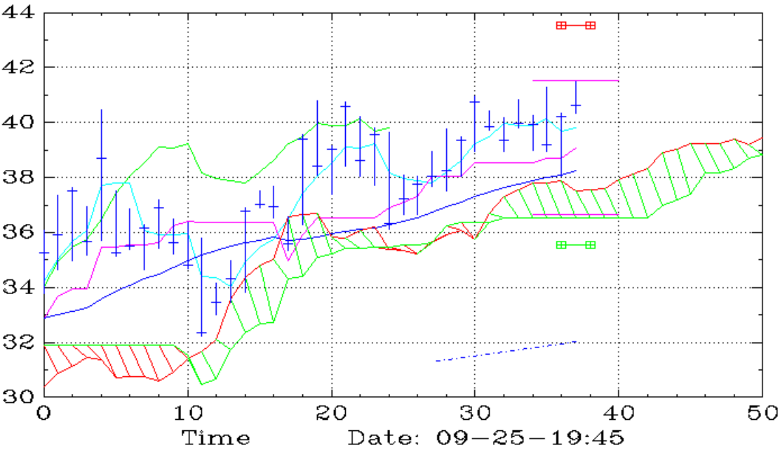
CPER (Weekly,Ichimoku)
