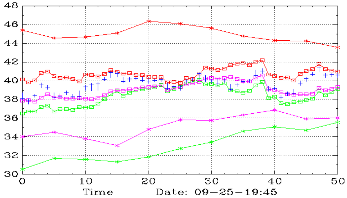
CPER (Weekly,Daily)
