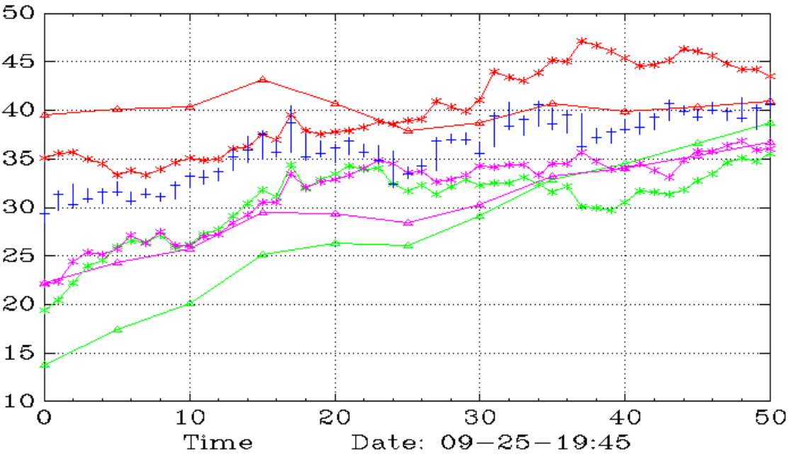
CPER (Monthly,Weekly)
