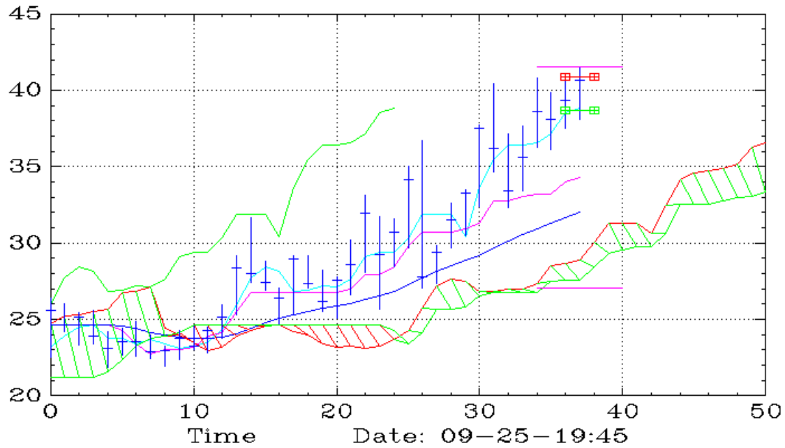
CPER (Monthly,Ichimoku)
