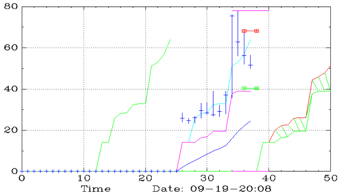
CSCL (Monthly,Ichimoku)
