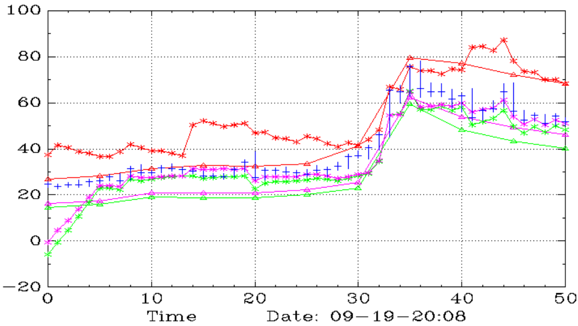
CSCL (Monthly,Weekly)
