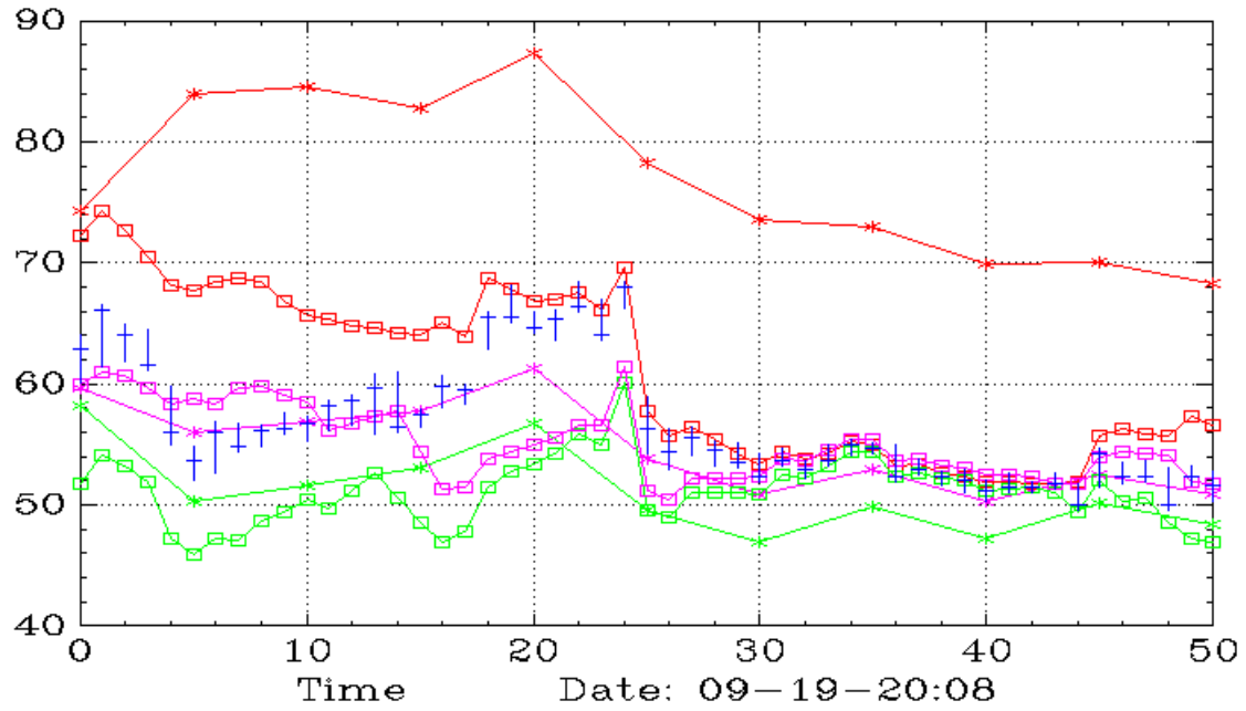
CSCL (Weekly,Daily)
