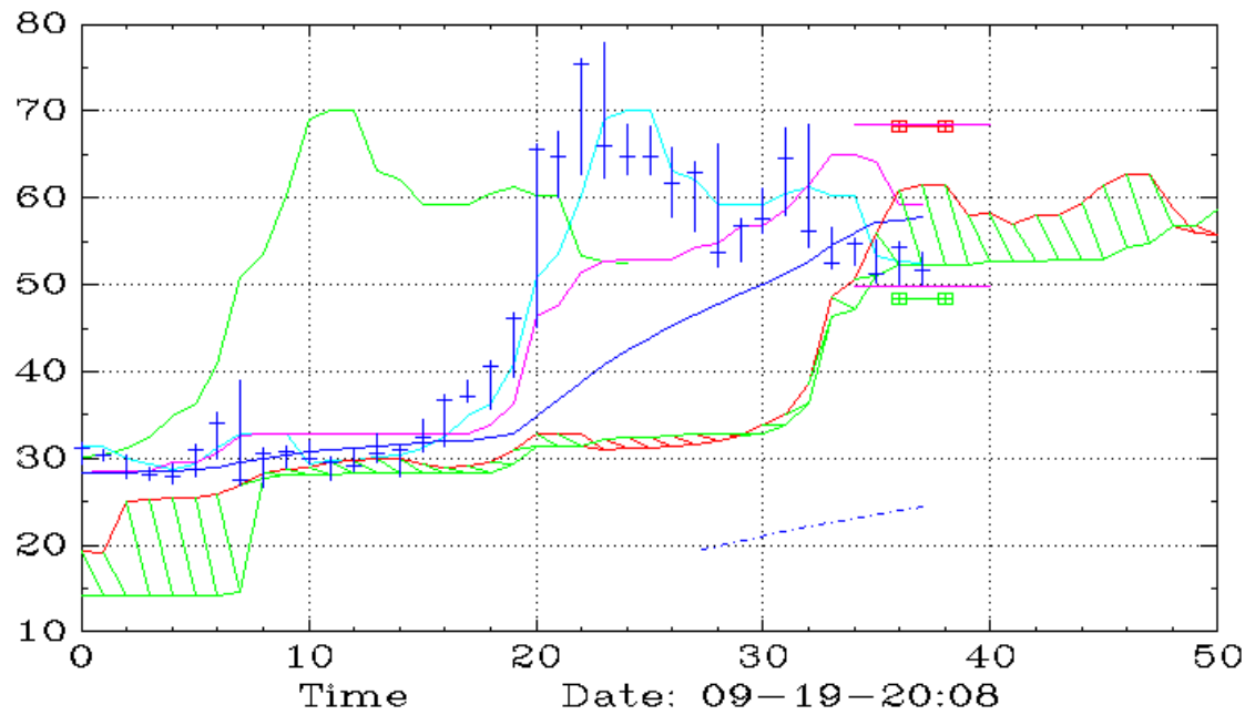
CSCL (Weekly,Ichimoku)
