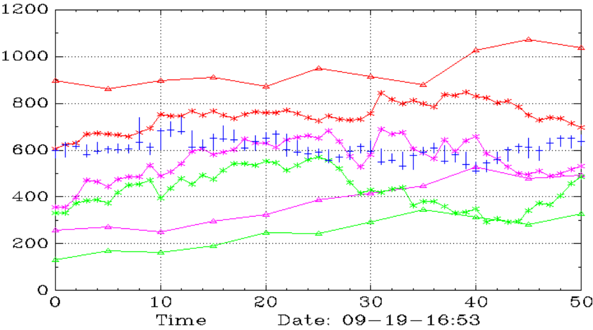
DDS (Monthly,Weekly)
