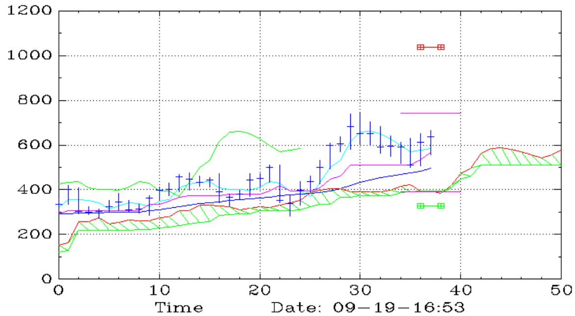
DDS (Monthly,Ichimoku)
