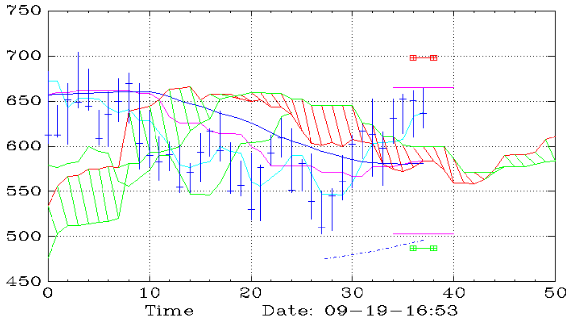
DDS (Weekly,Ichimoku)
