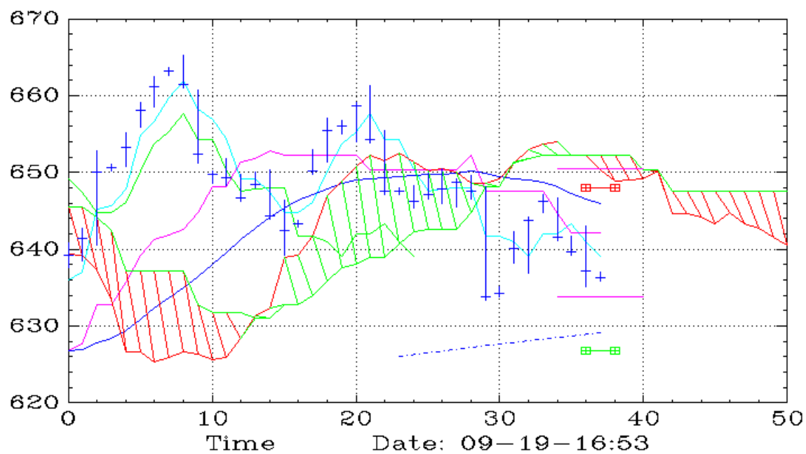
DDS (60,Ichimoku)
