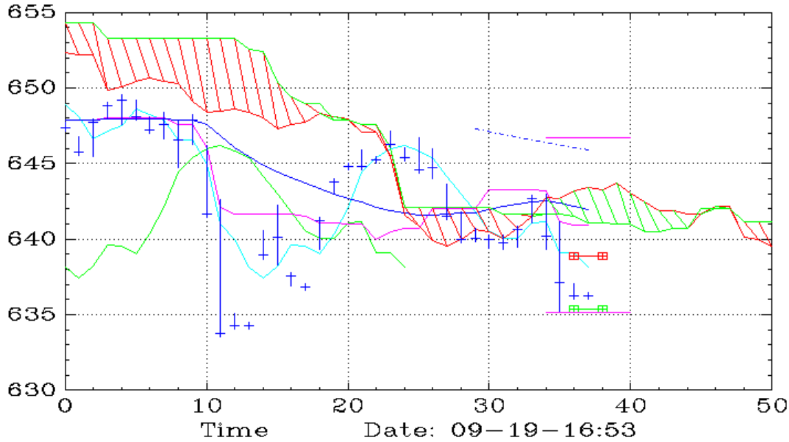
DDS (15,Ichimoku)
