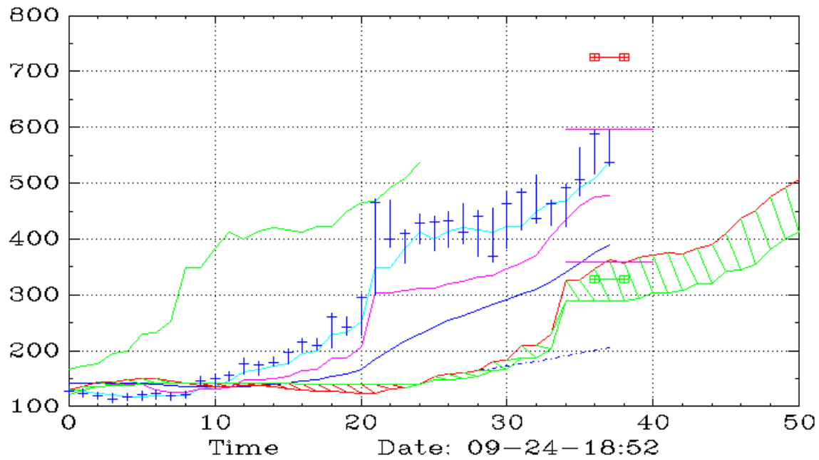
DELL (Weekly,Ichimoku)
