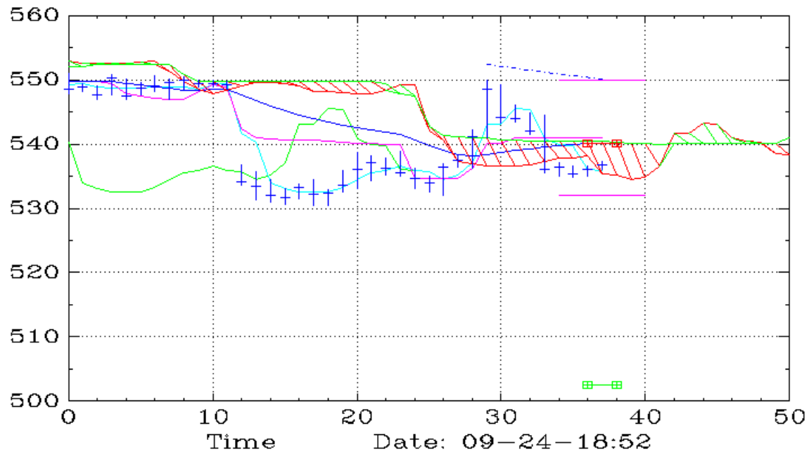
DELL (15,Ichimoku)
