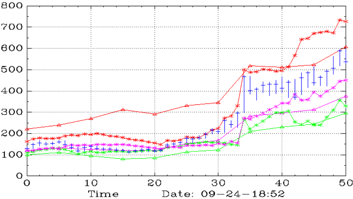
DELL (Monthly,Weekly)
