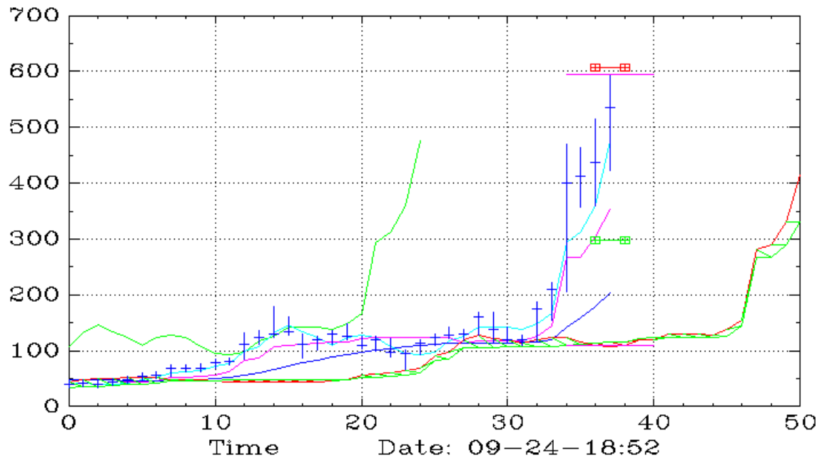
DELL (Monthly,Ichimoku)
