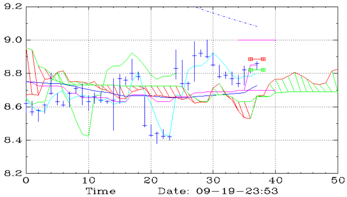
ERY (90,Ichimoku)
