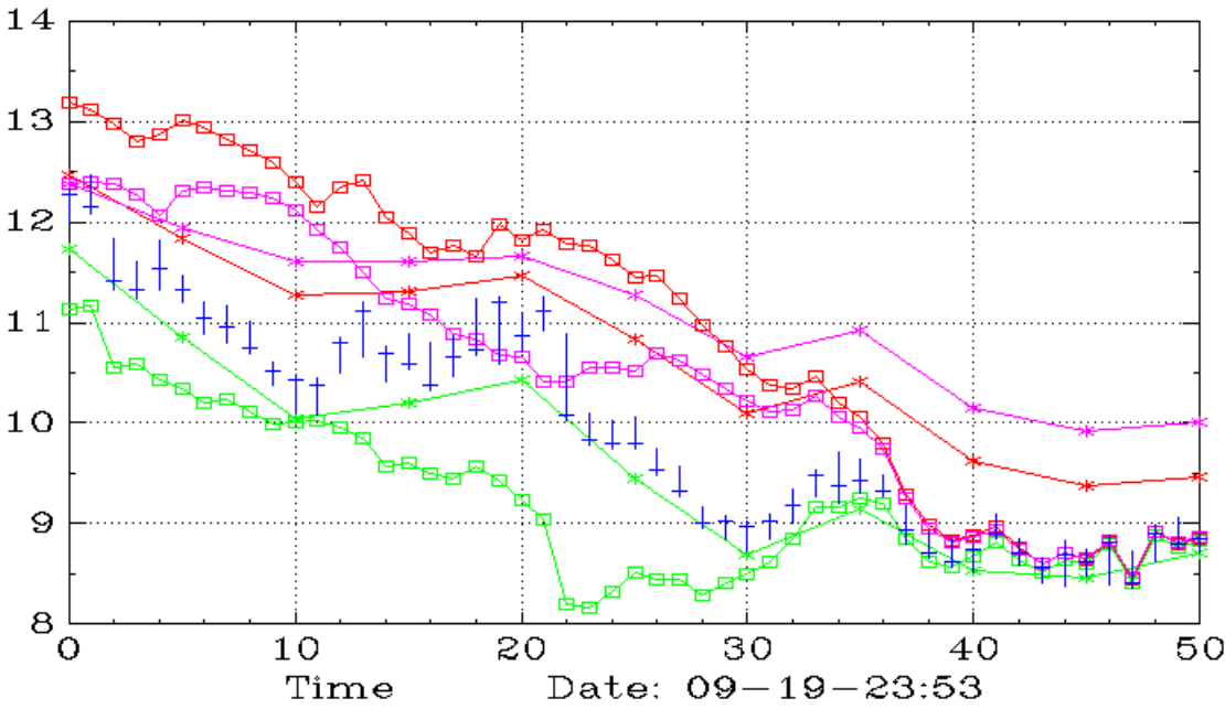
ERY (Weekly,Daily)
