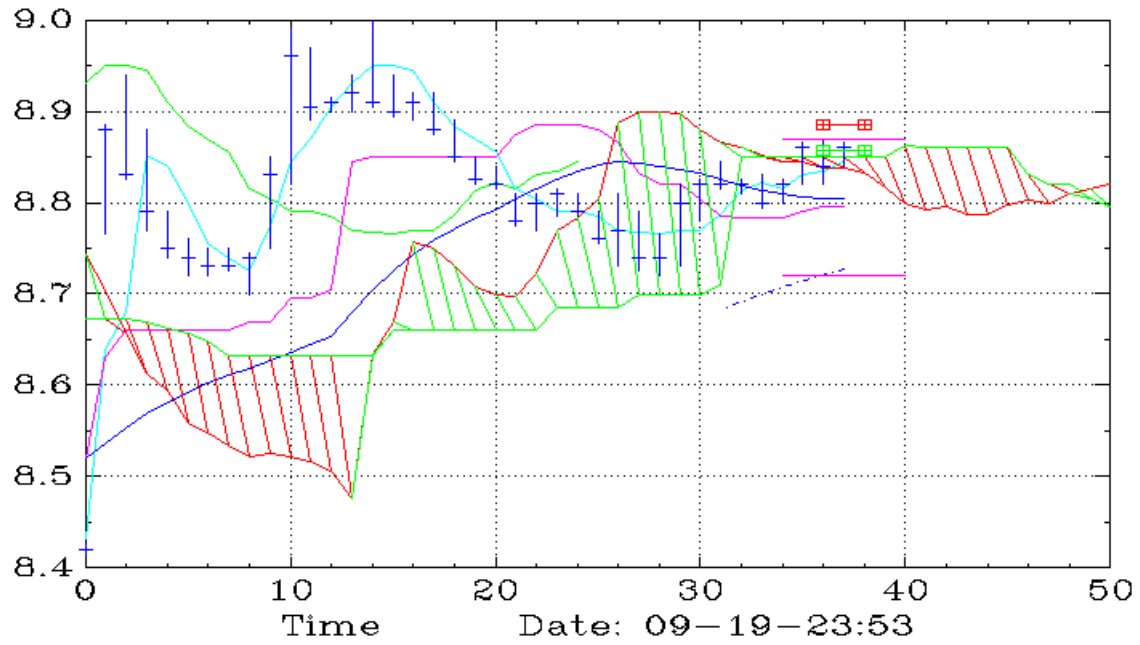
ERY (30,Ichimoku)
