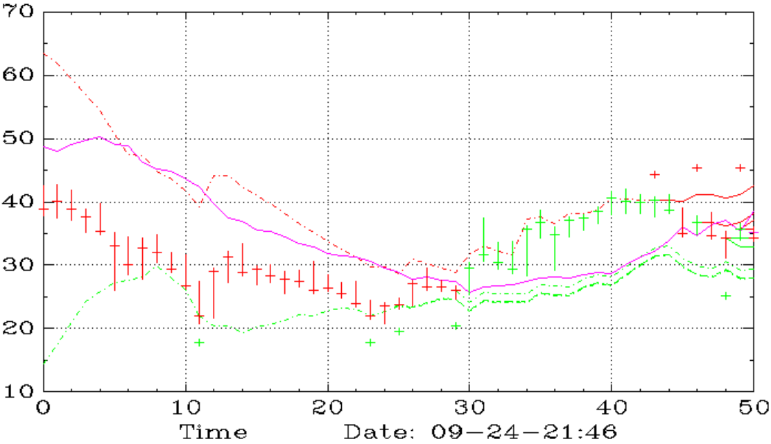
FXI (Monthly,SAR)
