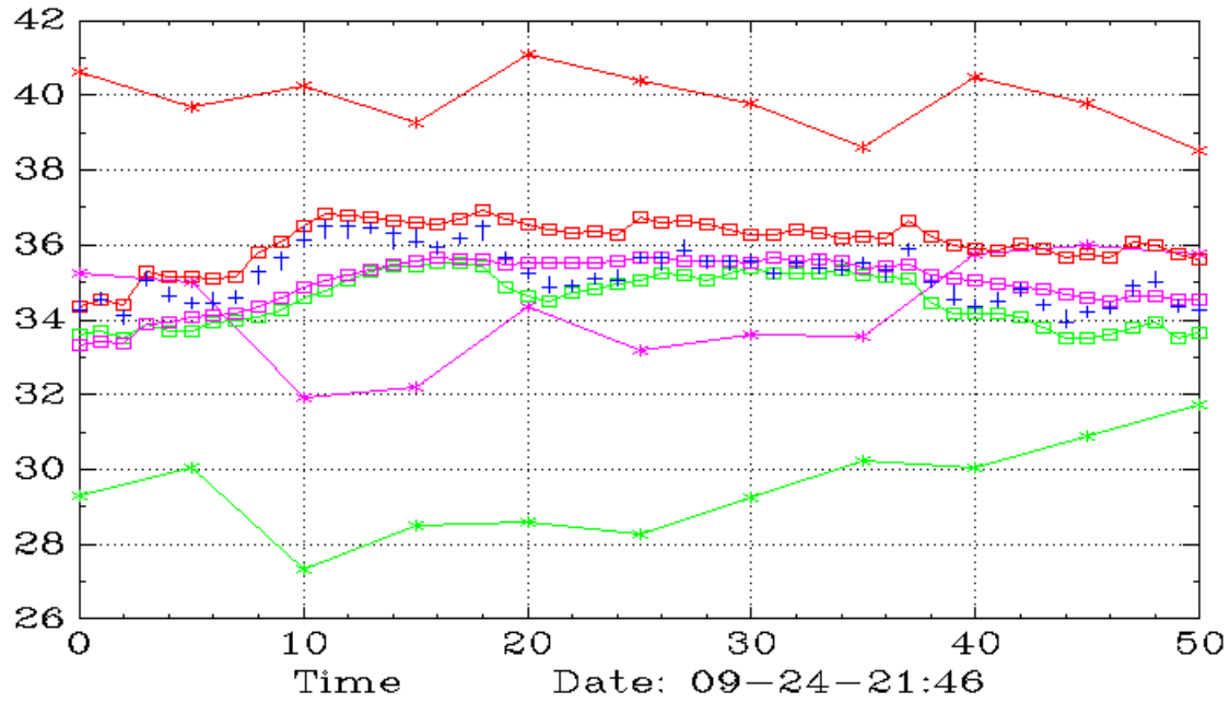
FXI (Weekly,Daily)
