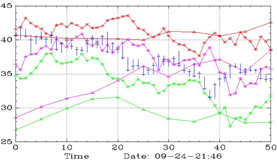
FXI (Monthly,Weekly)
