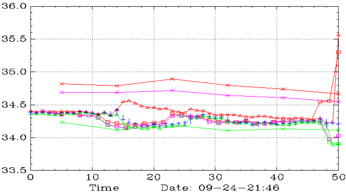
FXI (90,15,10)
