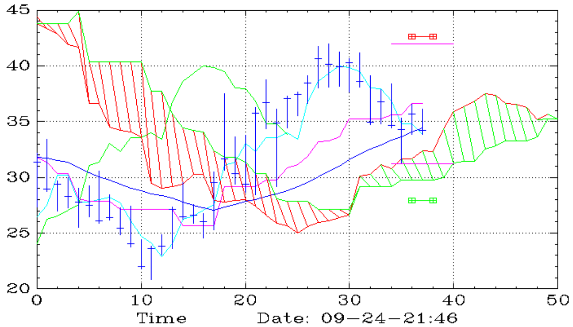
FXI (Monthly,Ichimoku)
