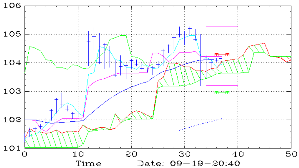
GGLL (15,Ichimoku)
