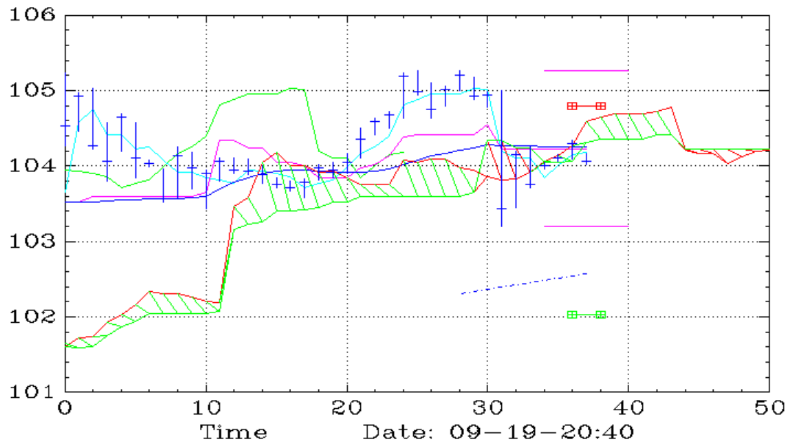
GGLL (10,Ichimoku)
