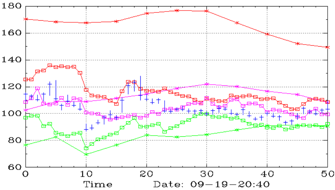
GGLL (Weekly,Daily)
