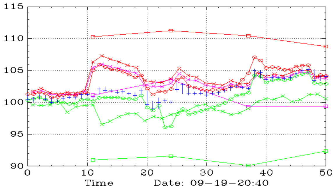
GGLL (Daily,45,30)
