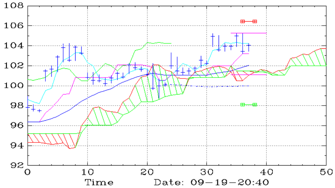
GGLL (60,Ichimoku)
