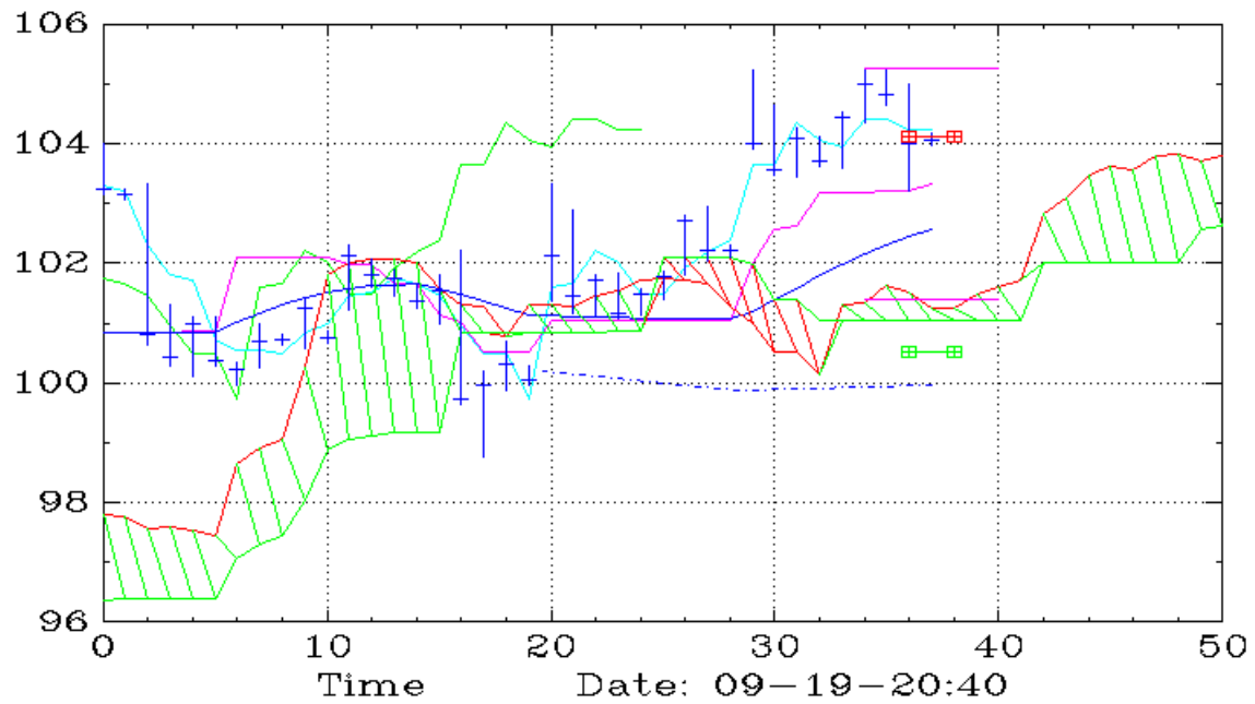
GGLL (45,Ichimoku)
