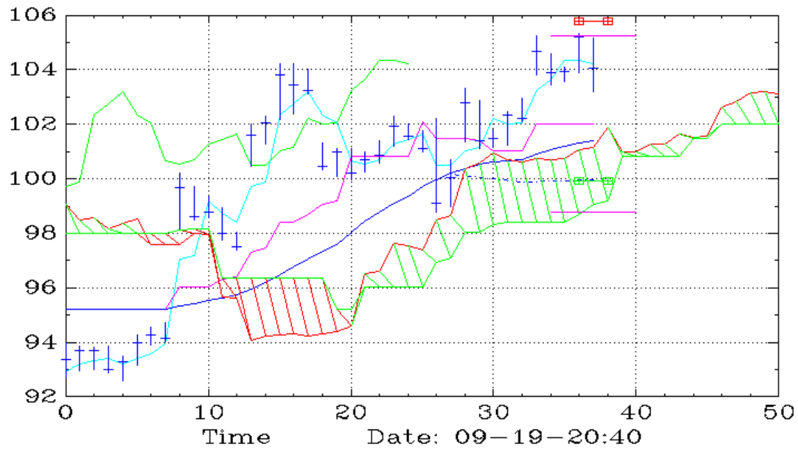
GGLL (90,Ichimoku)
