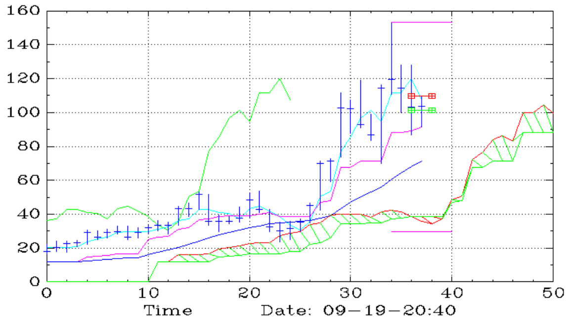
GGLL (Monthly,Ichimoku)
