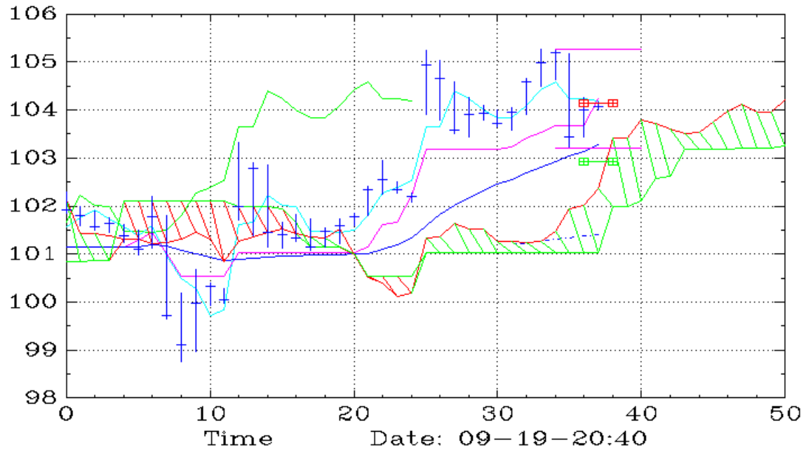
GGLL (30,Ichimoku)
