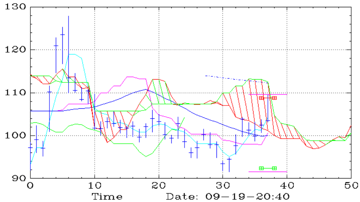
GGLL (Daily,Ichimoku)
