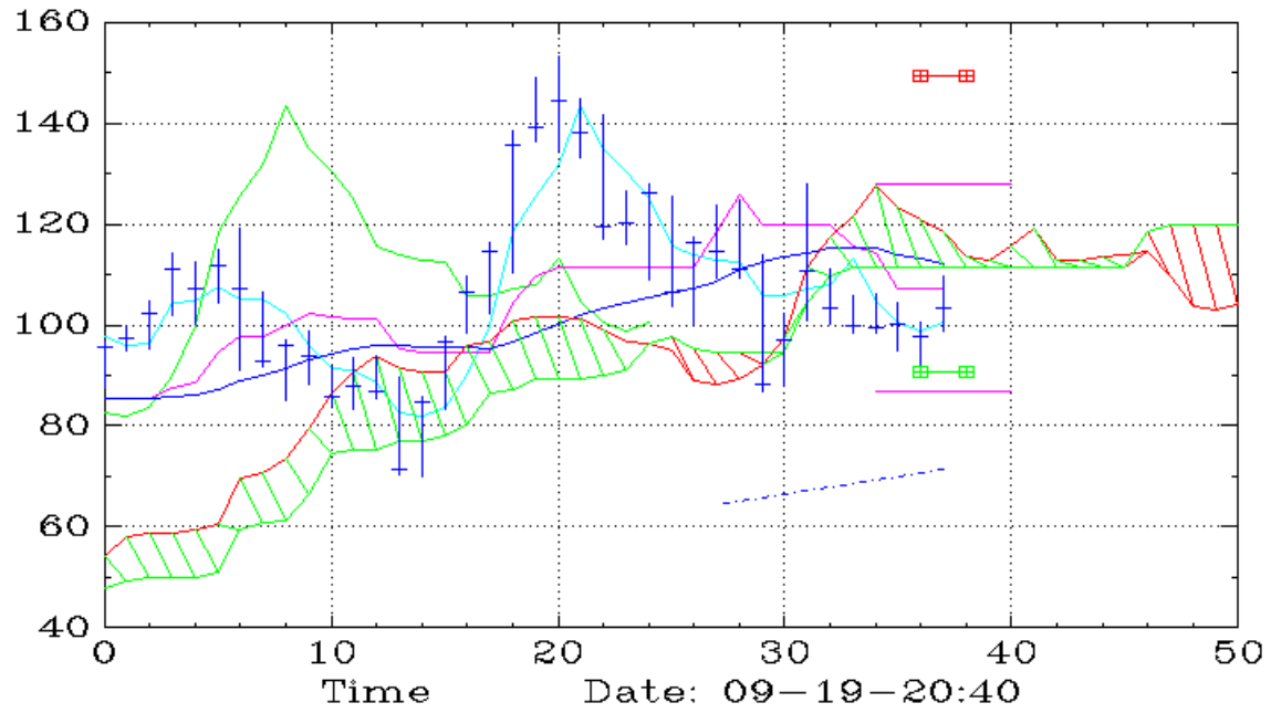
GGLL (Weekly,Ichimoku)
