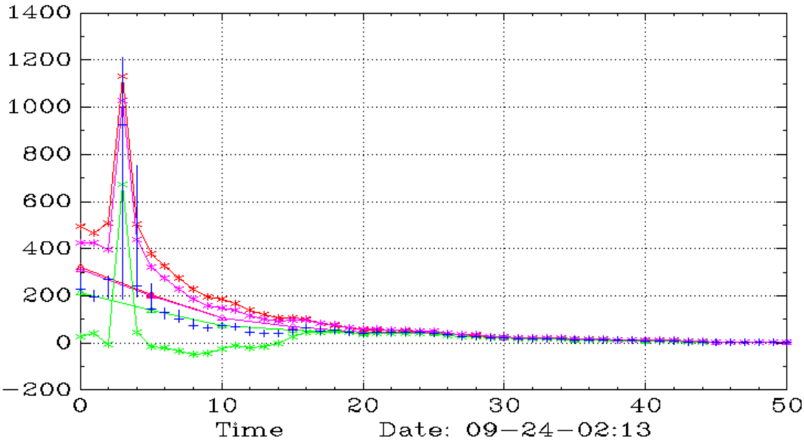
GNPX (Monthly,Weekly)
