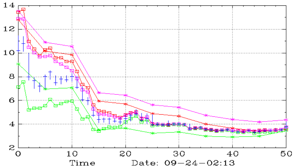
GNPX (Weekly,Daily)
