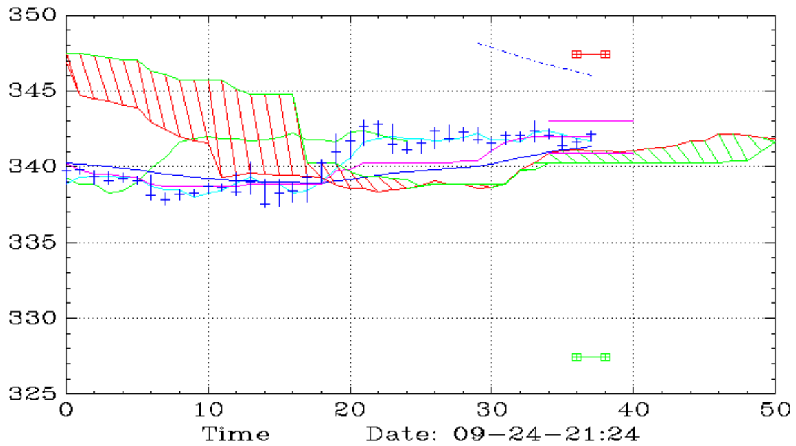
GOOGL (15,Ichimoku)
