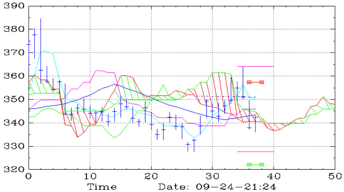
GOOGL (Daily,Ichimoku)
