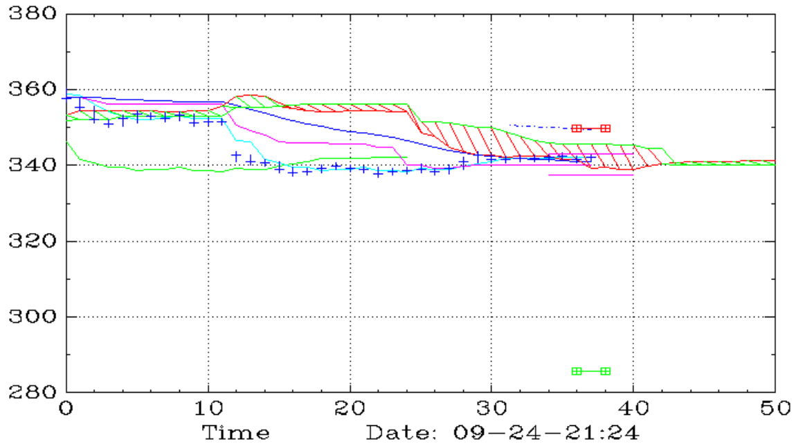
GOOGL (30,Ichimoku)
