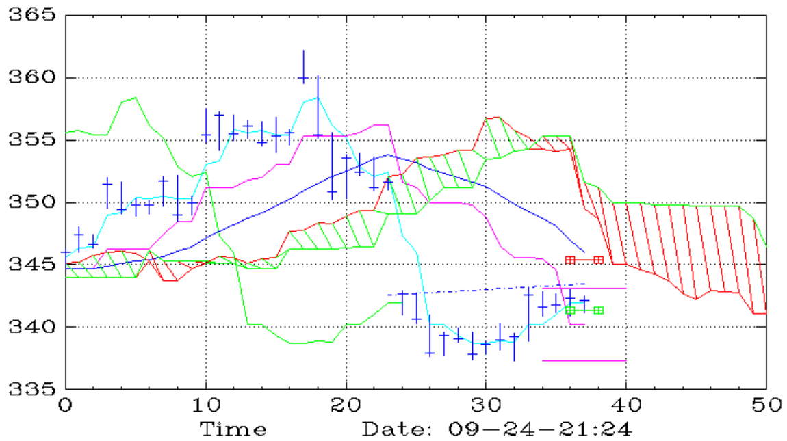
GOOGL (60,Ichimoku)
