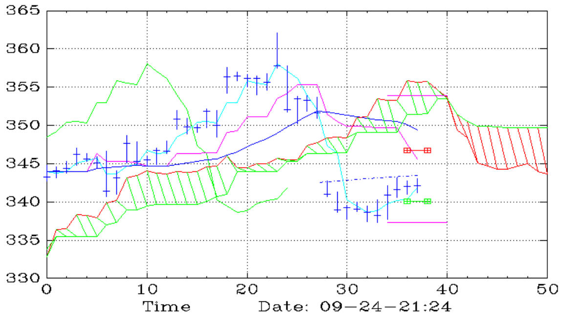
GOOGL (90,Ichimoku)
