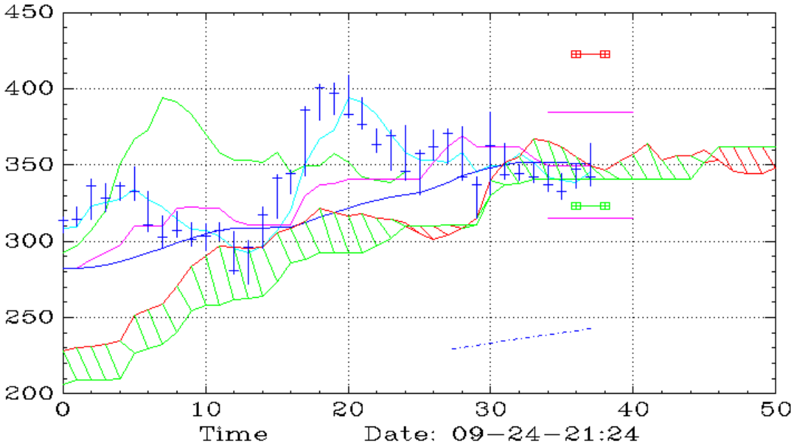
GOOGL (Weekly,Ichimoku)
