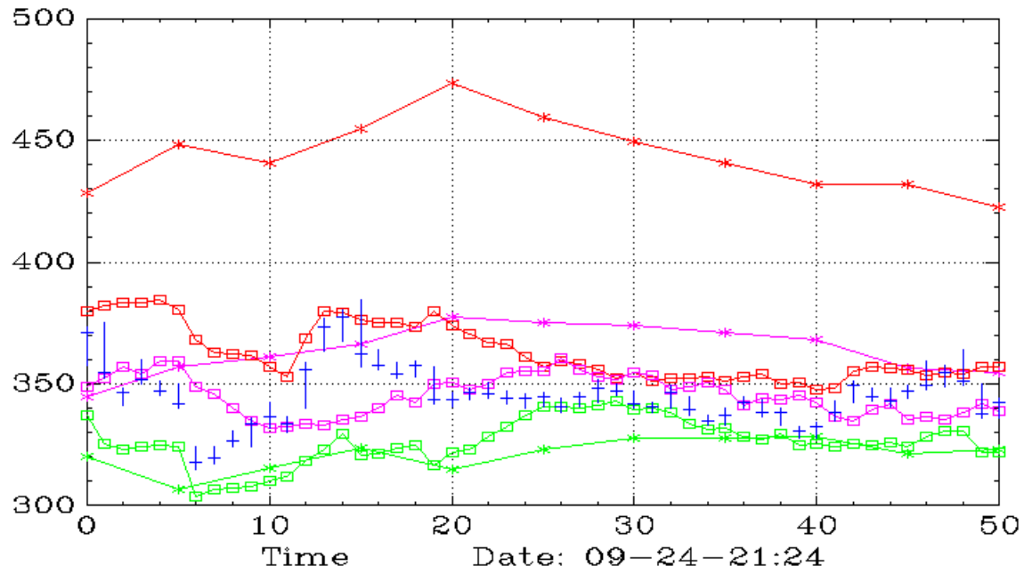
GOOGL (Weekly,Daily)
