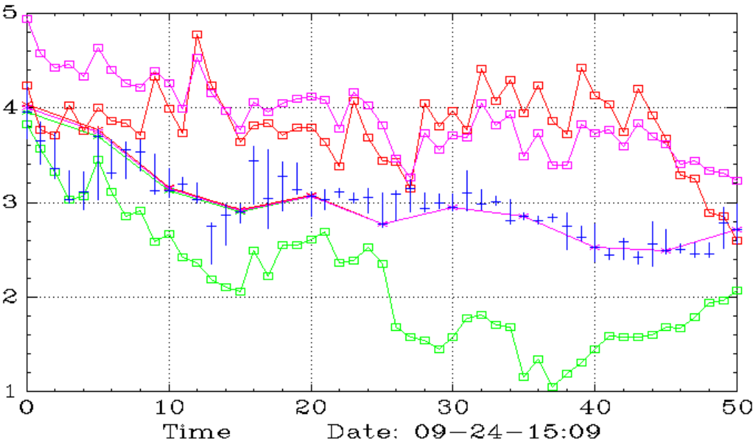
HKIT (Weekly,Daily)
