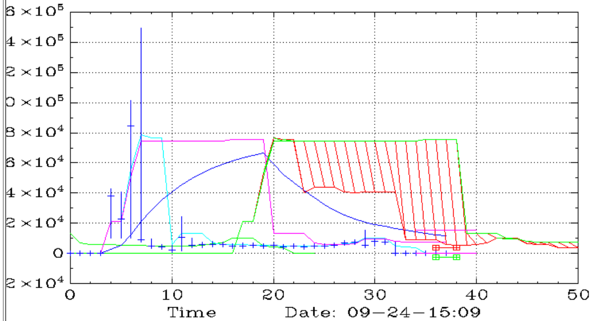
HKIT (Monthly,Ichimoku)
