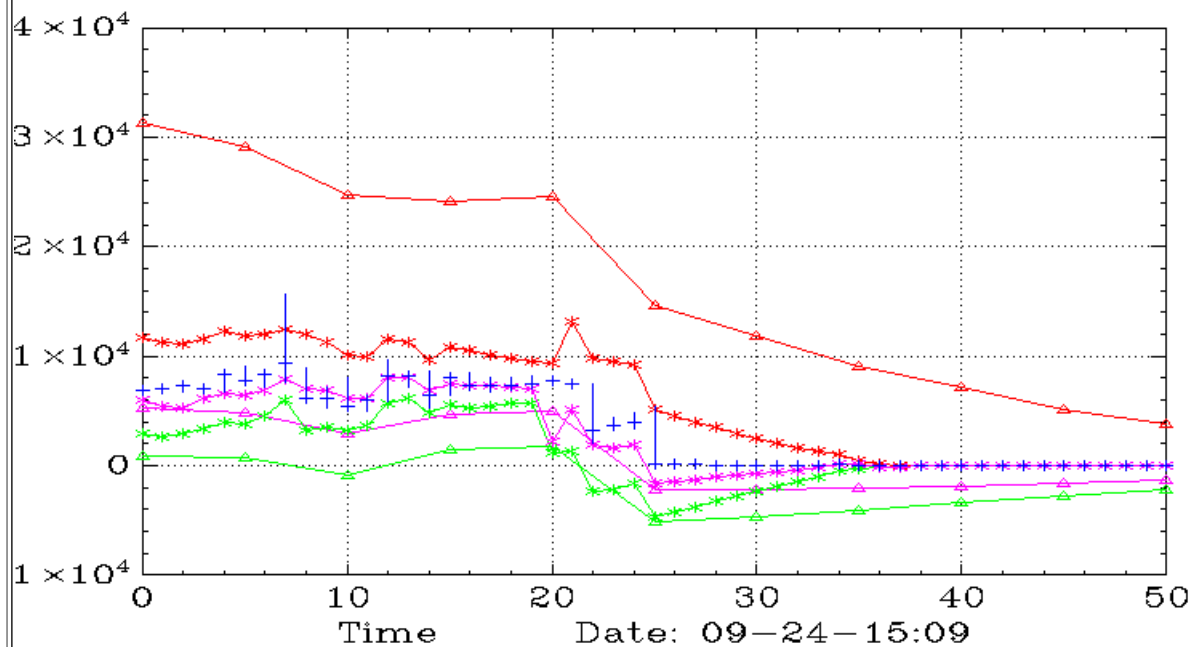
HKIT (Monthly,Weekly)
