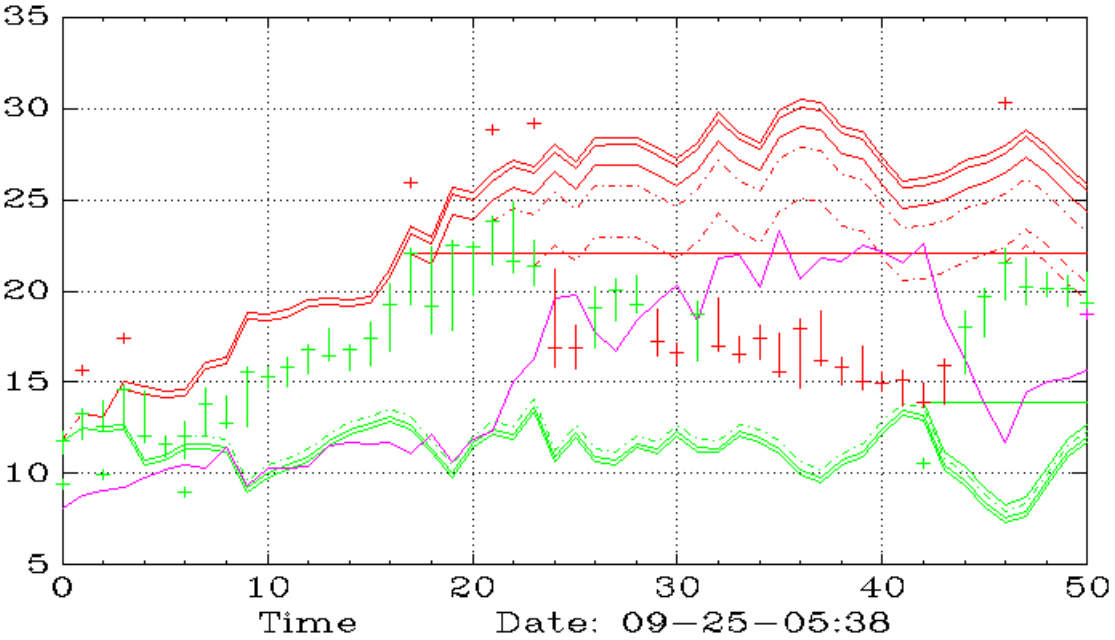
IAG (Weekly,SAR)
