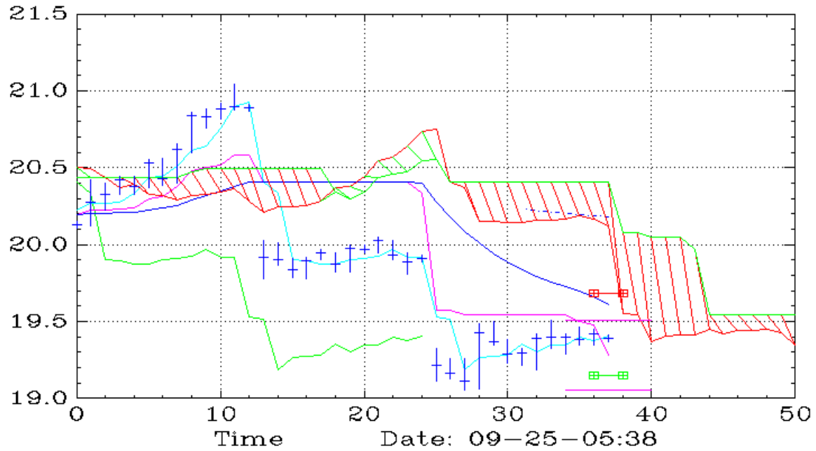
IAG (30,Ichimoku)
