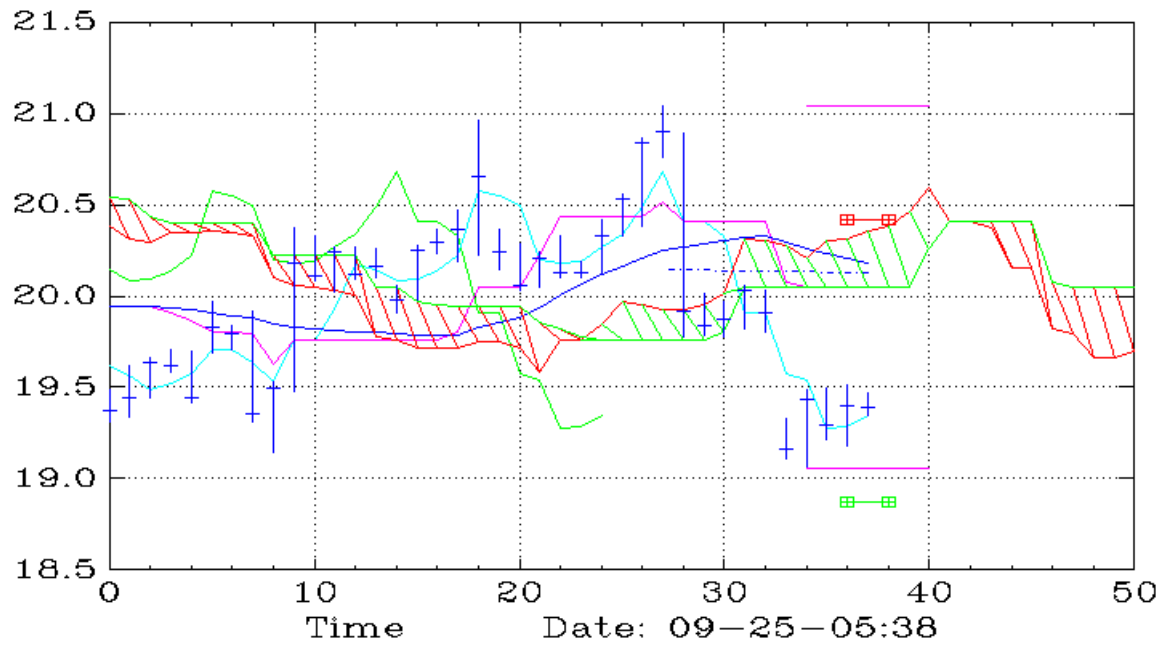
IAG (90,Ichimoku)
