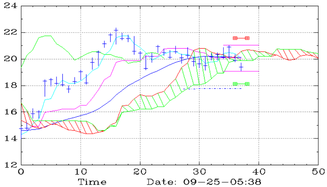
IAG (Daily,Ichimoku)
