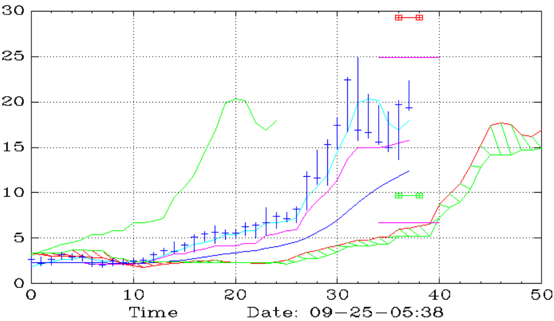
IAG (Monthly,Ichimoku)
