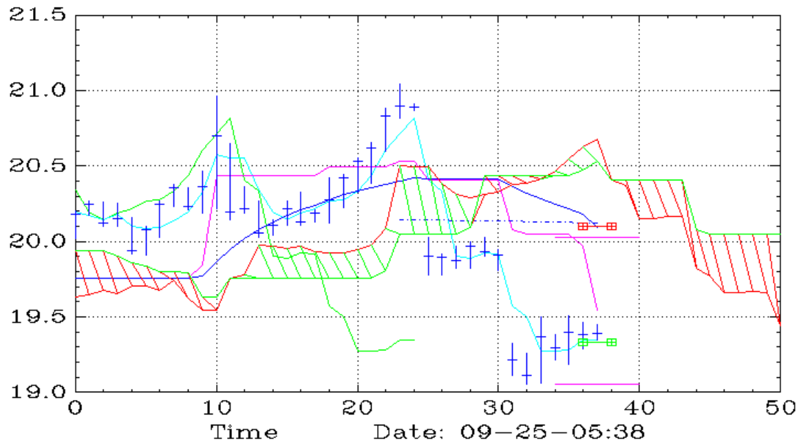
IAG (60,Ichimoku)
