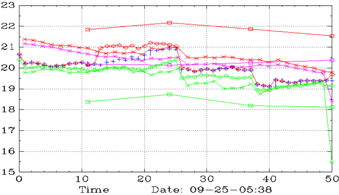
IAG (Daily,45,30)
