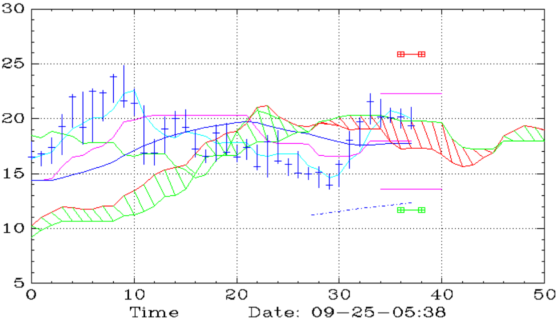
IAG (Weekly,Ichimoku)
