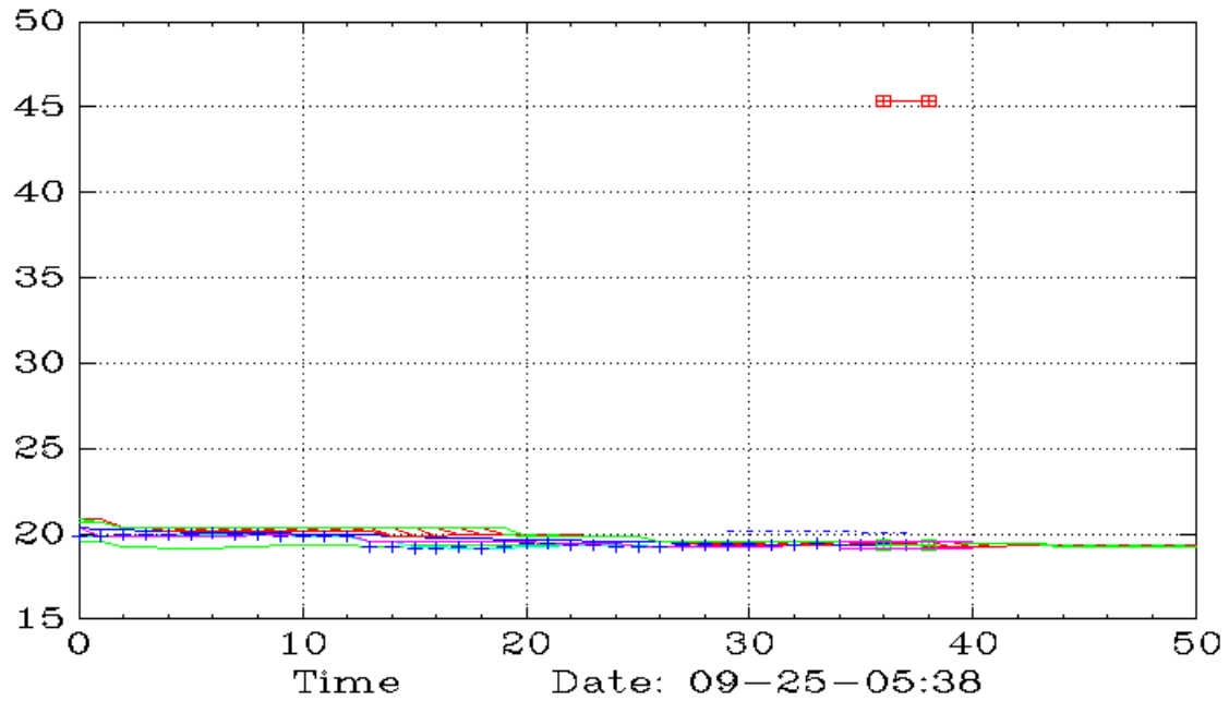
IAG (15,Ichimoku)
