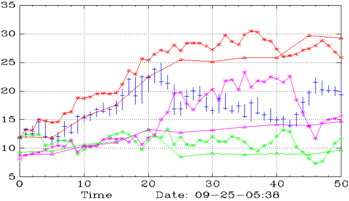
IAG (Monthly,Weekly)
