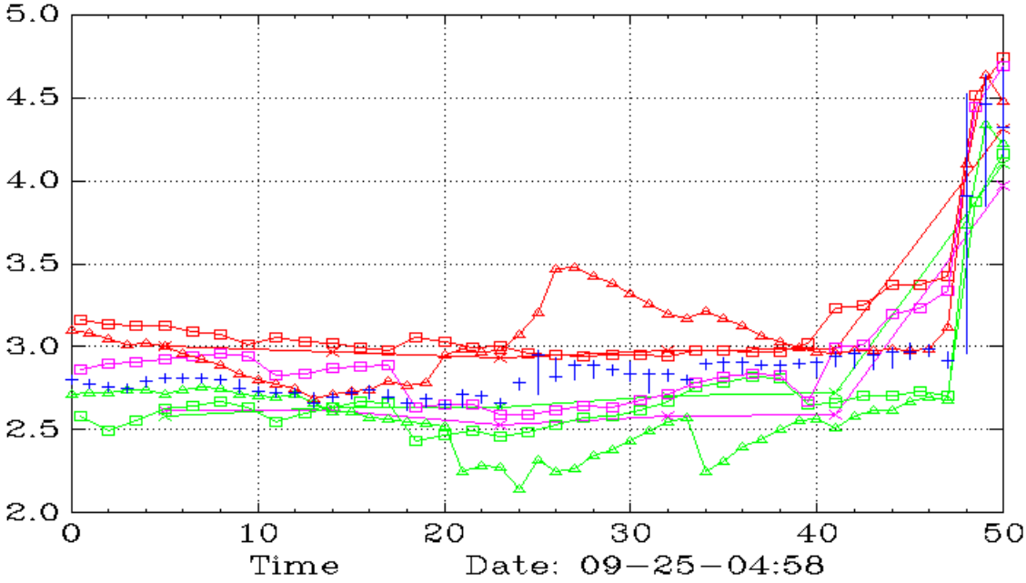
INLF (90,15,10)
