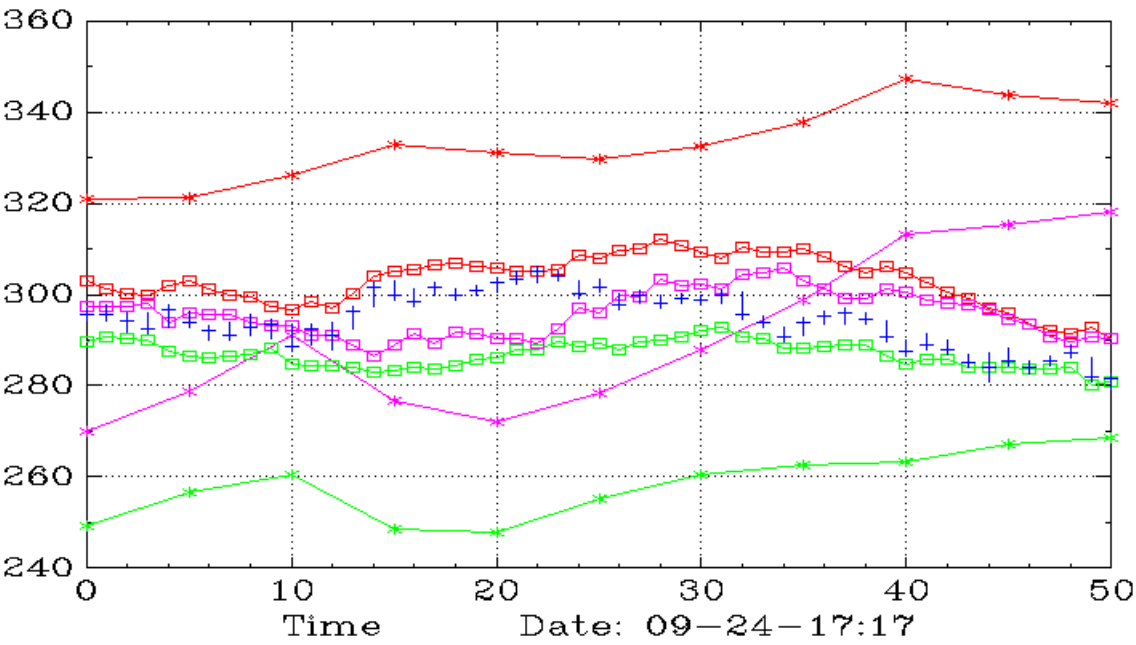
IWM (Weekly,Daily)
