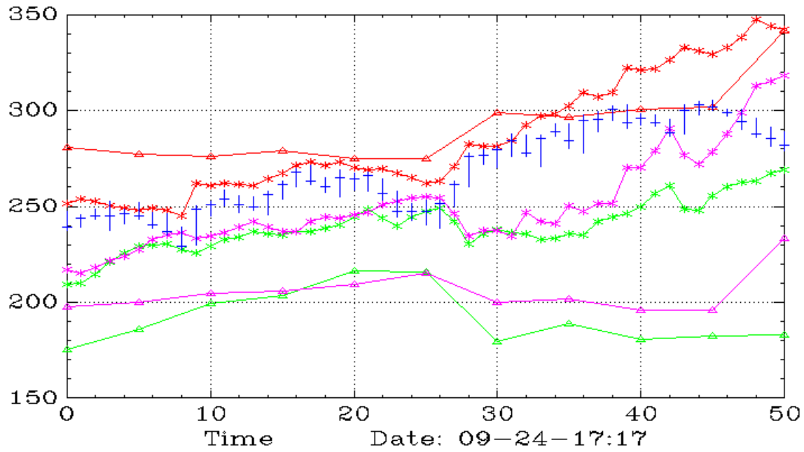
IWM (Monthly,Weekly)
