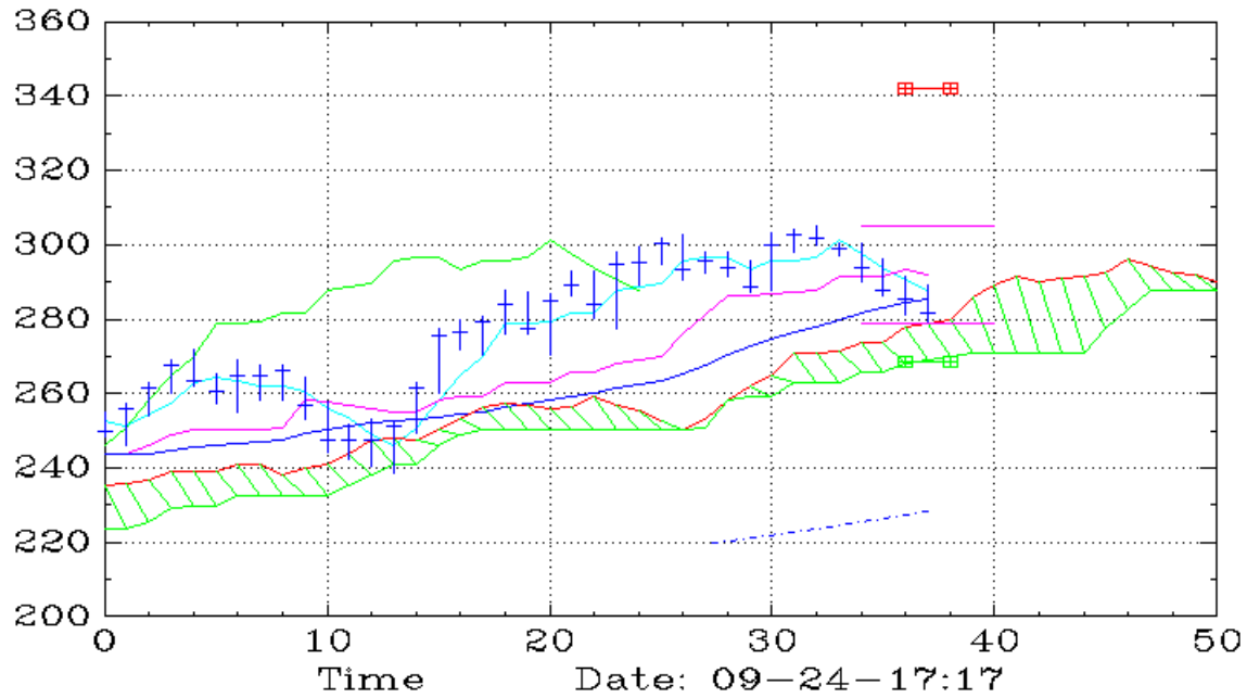
IWM (Weekly,Ichimoku)
