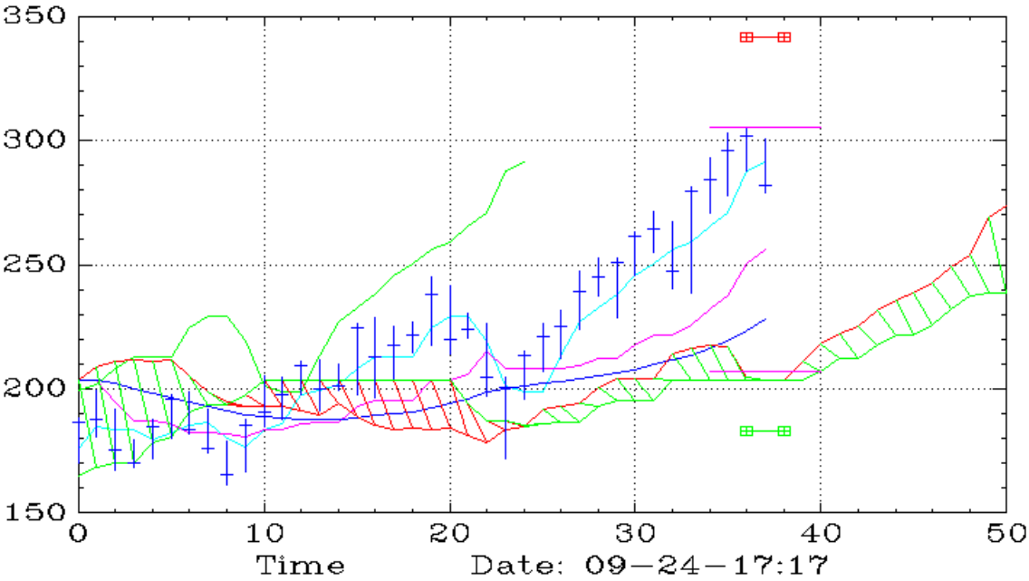
IWM (Monthly,Ichimoku)
