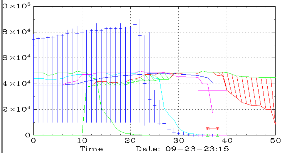
KIDZ (Monthly,Ichimoku)
