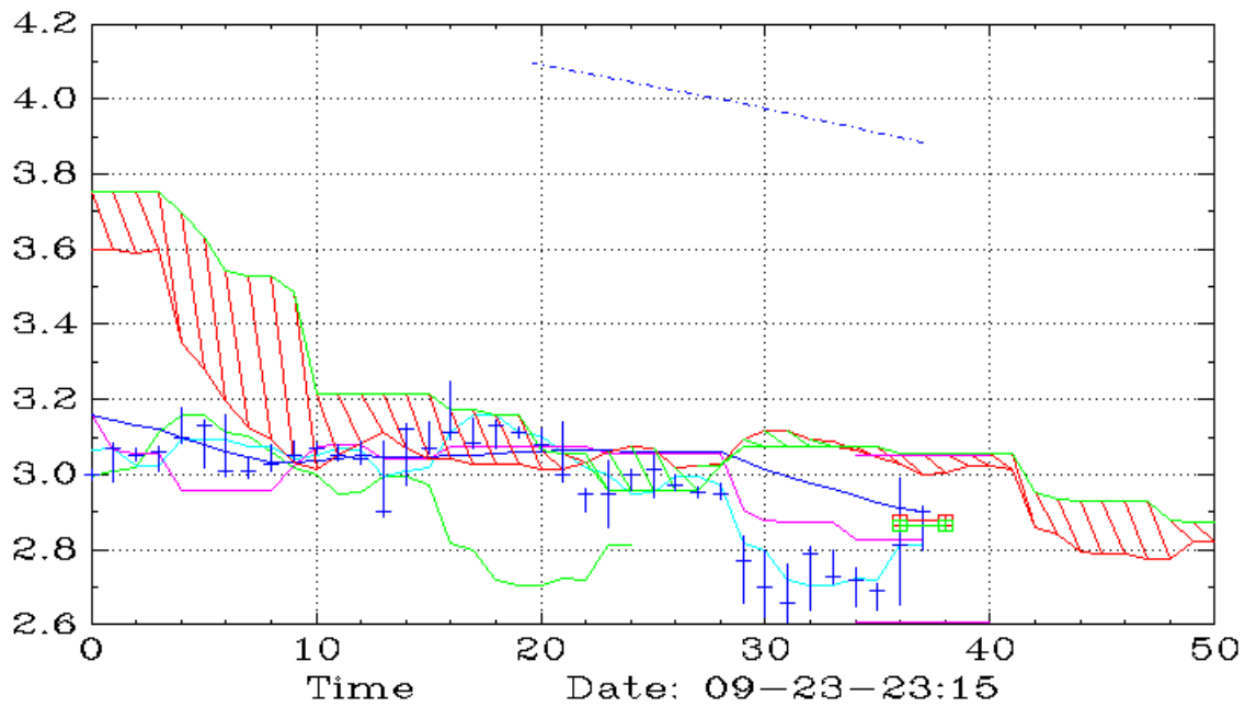
KIDZ (45,Ichimoku)
