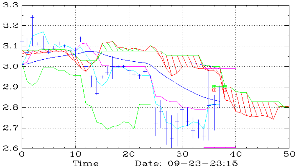
KIDZ (30,Ichimoku)
