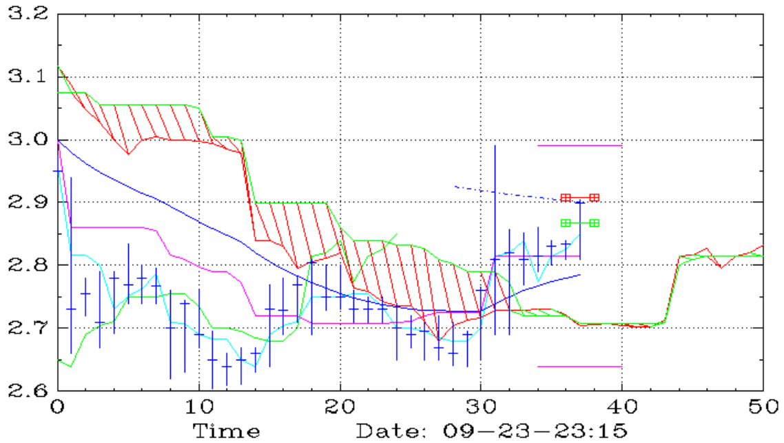
KIDZ (10,Ichimoku)
