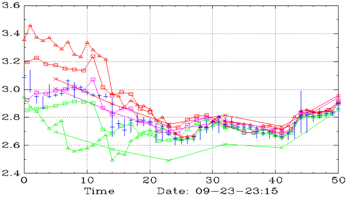
KIDZ (90,15,10)
