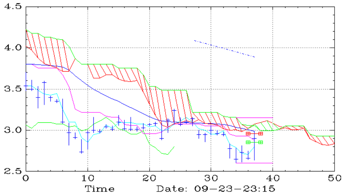
KIDZ (90,Ichimoku)
