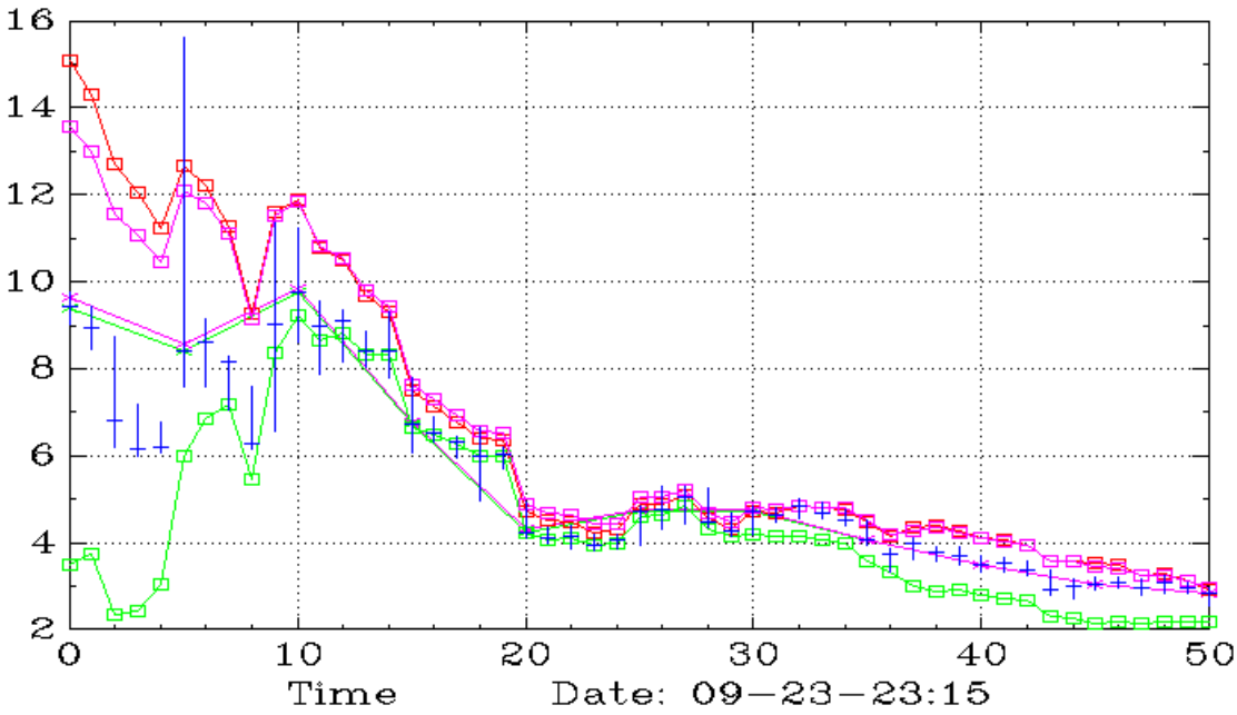
KIDZ (Weekly,Daily)
