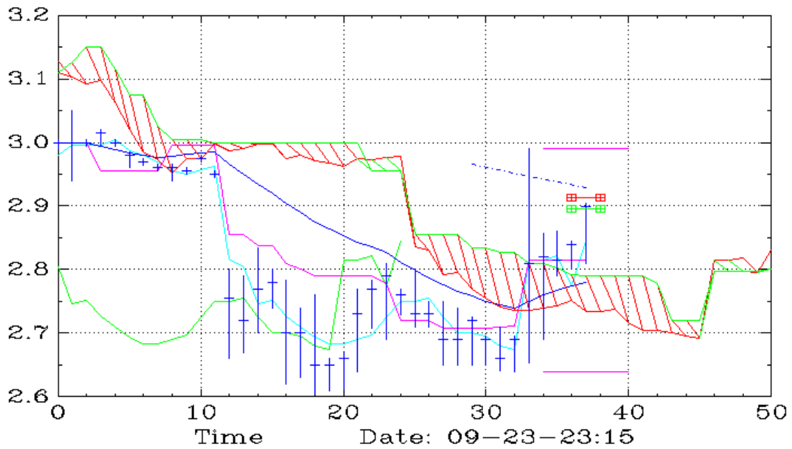
KIDZ (15,Ichimoku)
