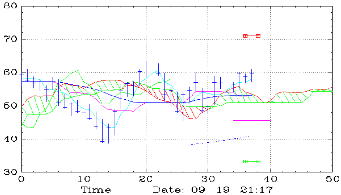
MAGX (Weekly,Ichimoku)
