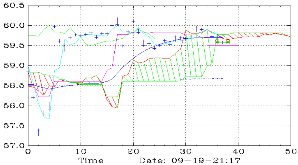
MAGX (15,Ichimoku)
