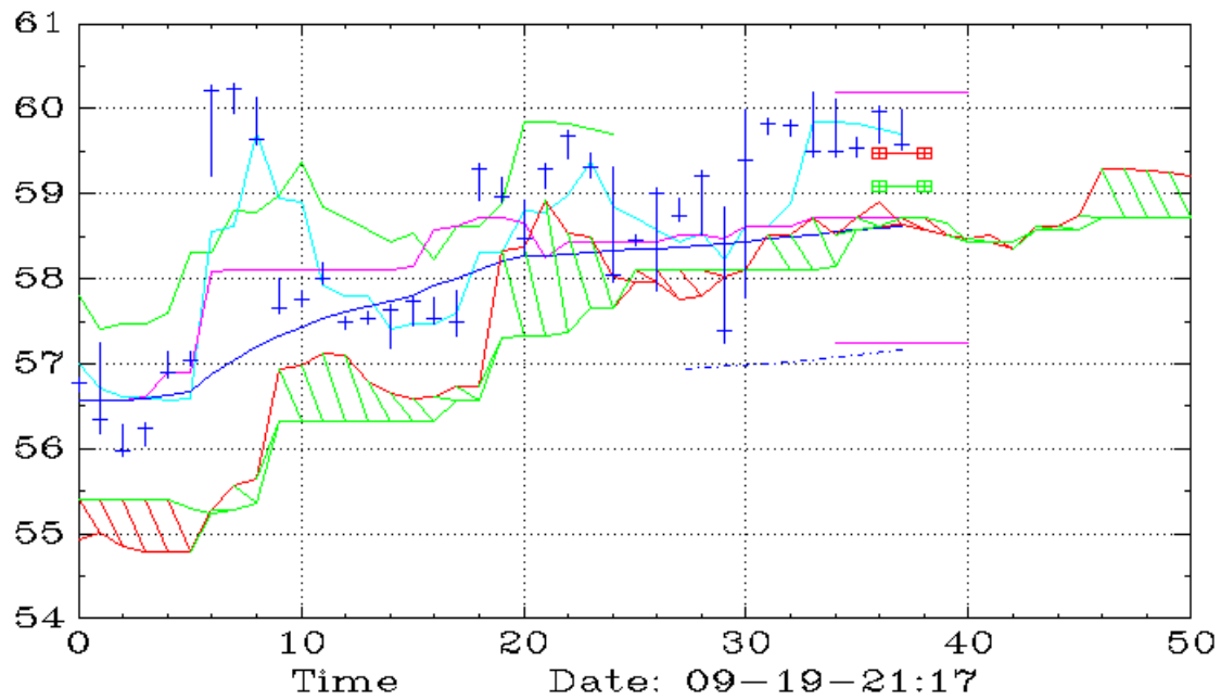
MAGX (90,Ichimoku)
