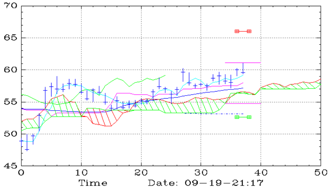
MAGX (Daily,Ichimoku)
