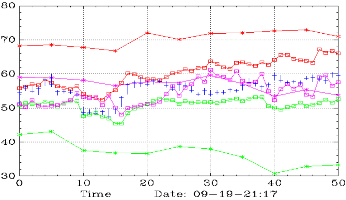
MAGX (Weekly,Daily)
