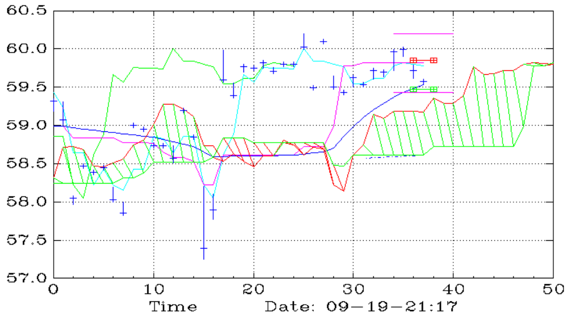
MAGX (30,Ichimoku)
