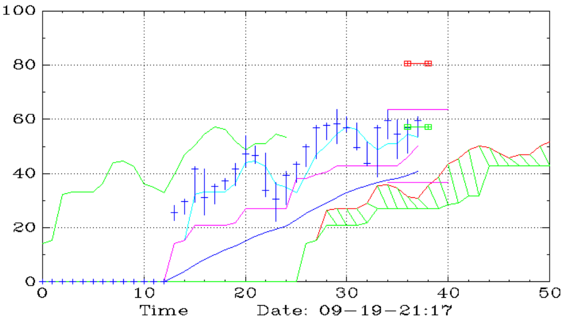
MAGX (Monthly,Ichimoku)
