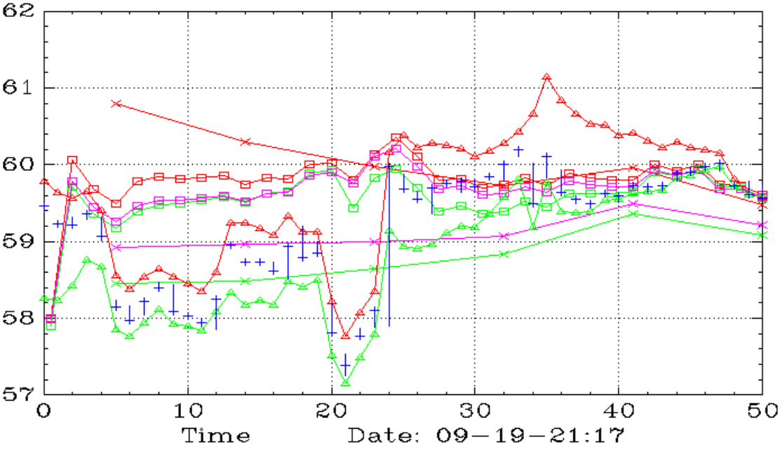
MAGX (90,15,10)
