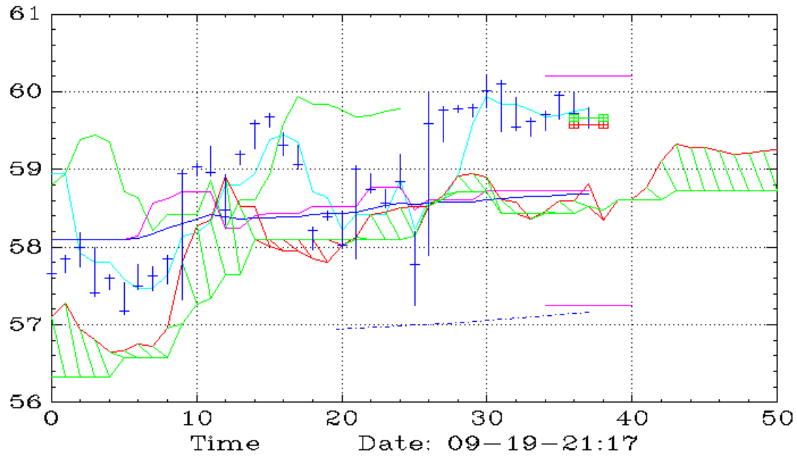
MAGX (45,Ichimoku)
