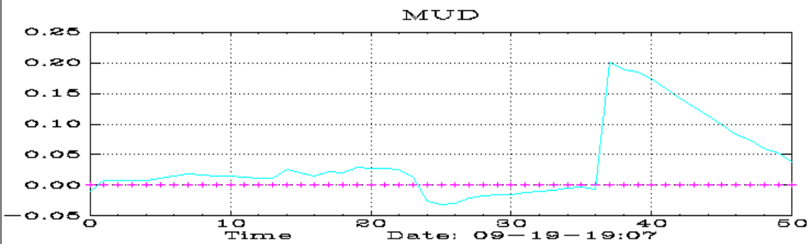
MUD Exhaustion Chart for 30
