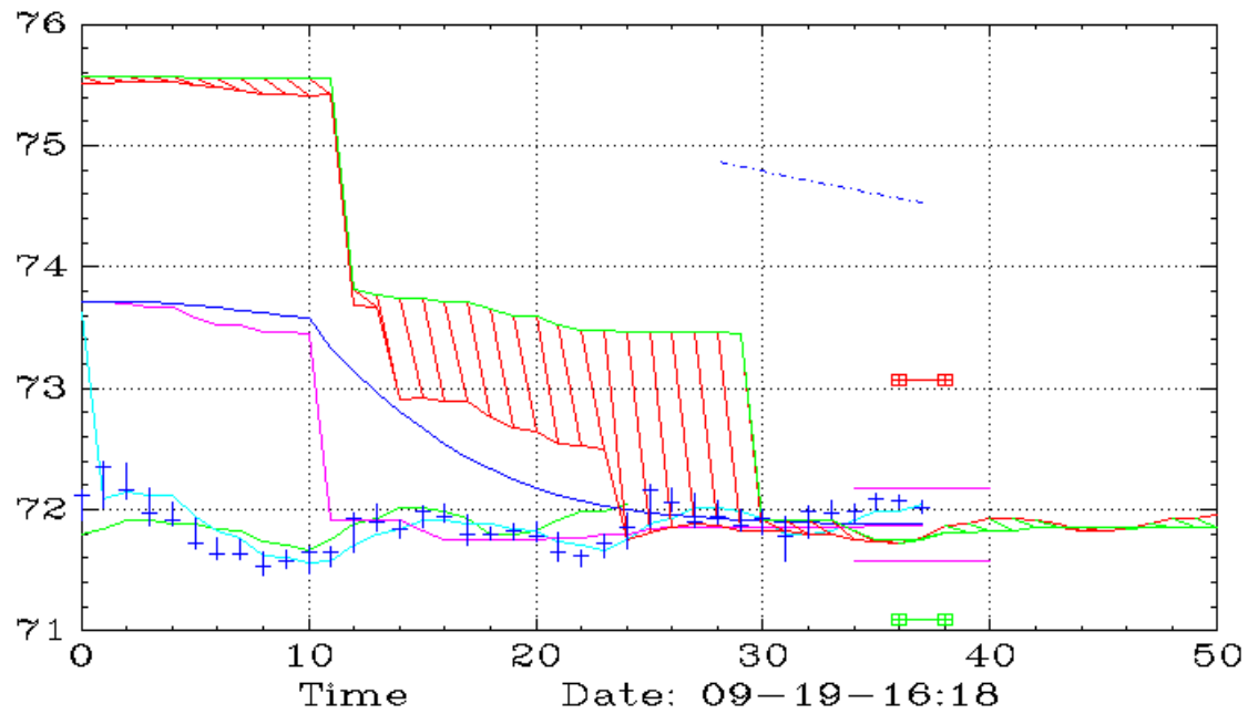
NFLX (10,Ichimoku)
