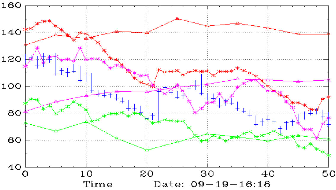
NFLX (Monthly,Weekly)
