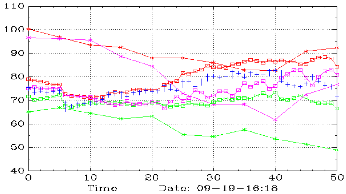
NFLX (Weekly,Daily)
