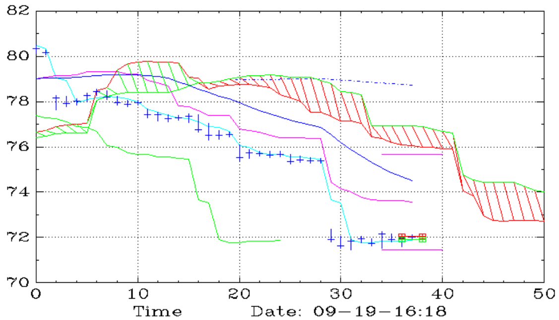
NFLX (45,Ichimoku)
