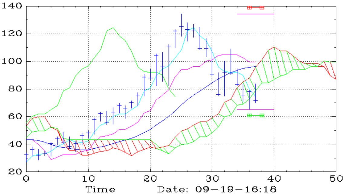
NFLX (Monthly,Ichimoku)
