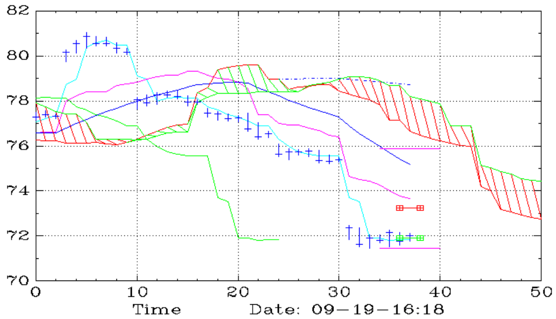
NFLX (60,Ichimoku)
