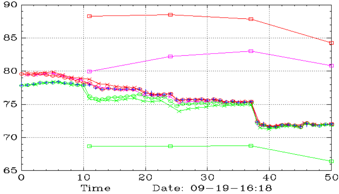
NFLX (Daily,45,30)
