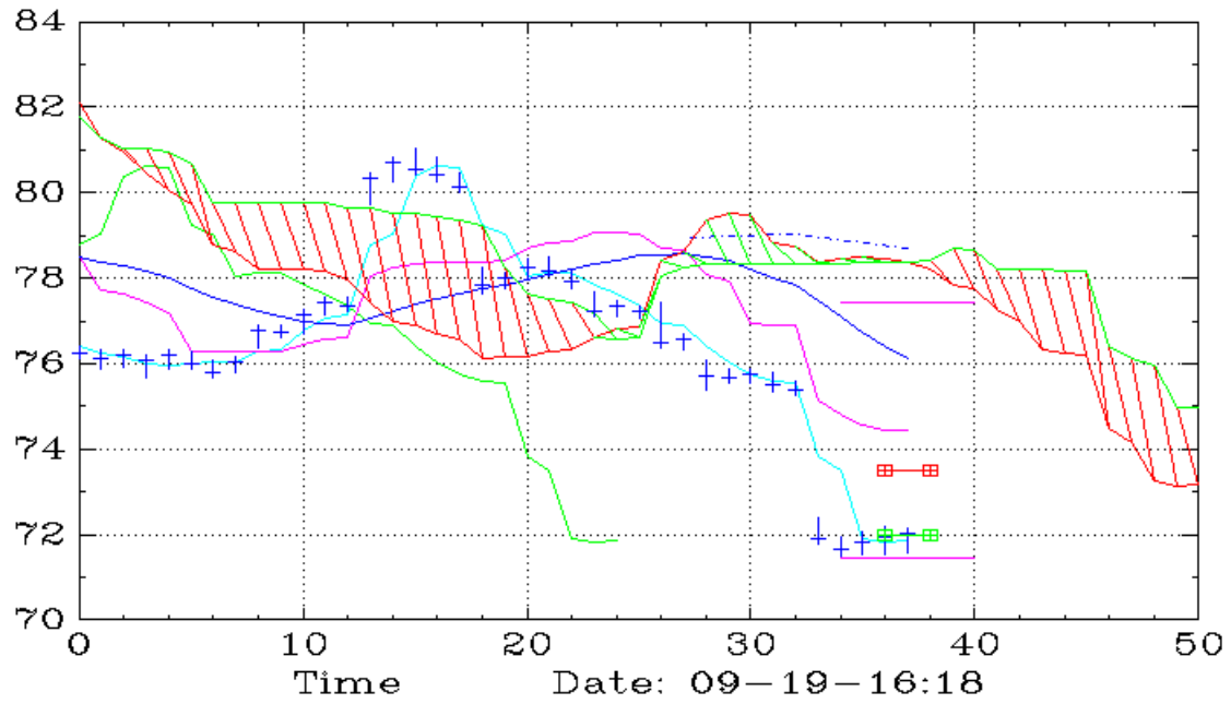
NFLX (90,Ichimoku)
