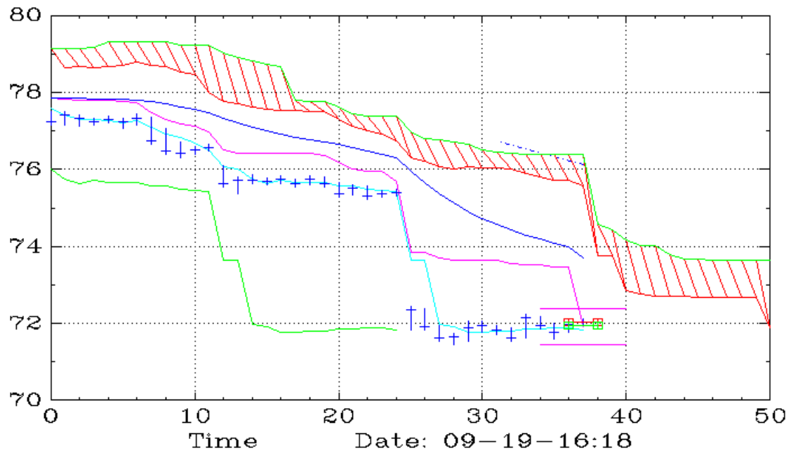
NFLX (30,Ichimoku)
