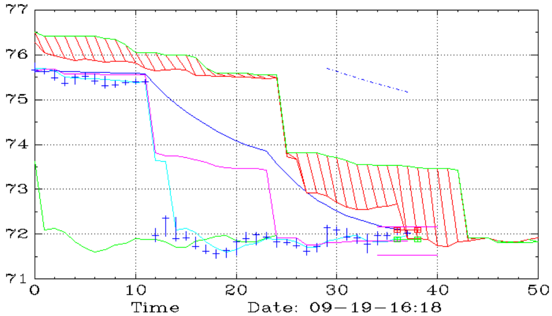
NFLX (15,Ichimoku)
