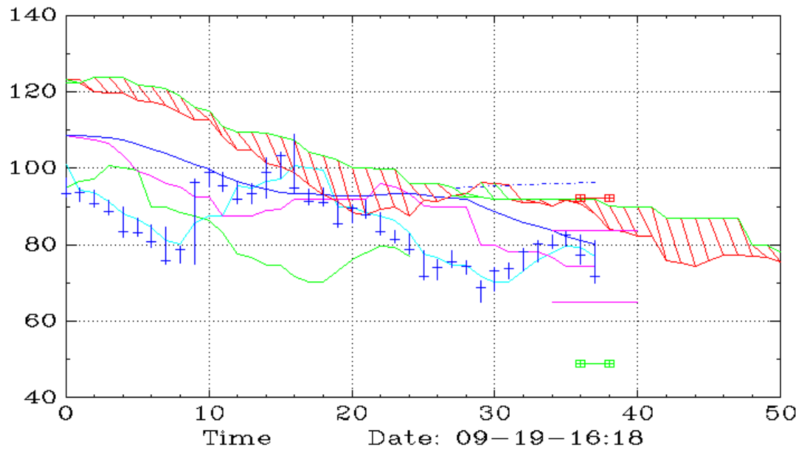
NFLX (Weekly,Ichimoku)
