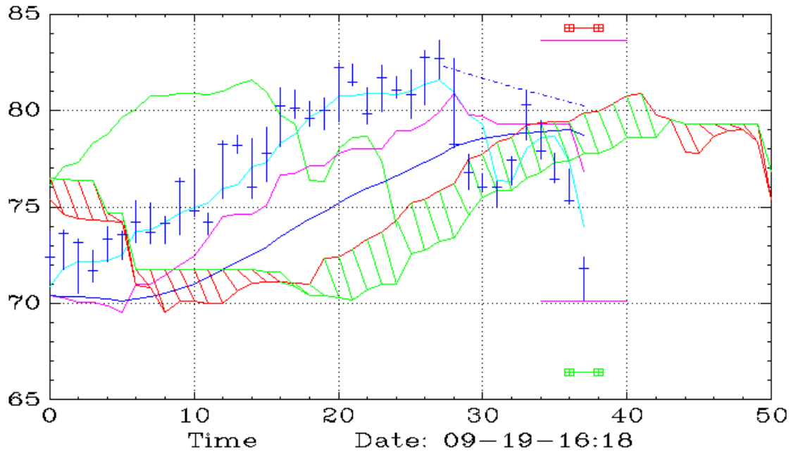
NFLX (Daily,Ichimoku)
