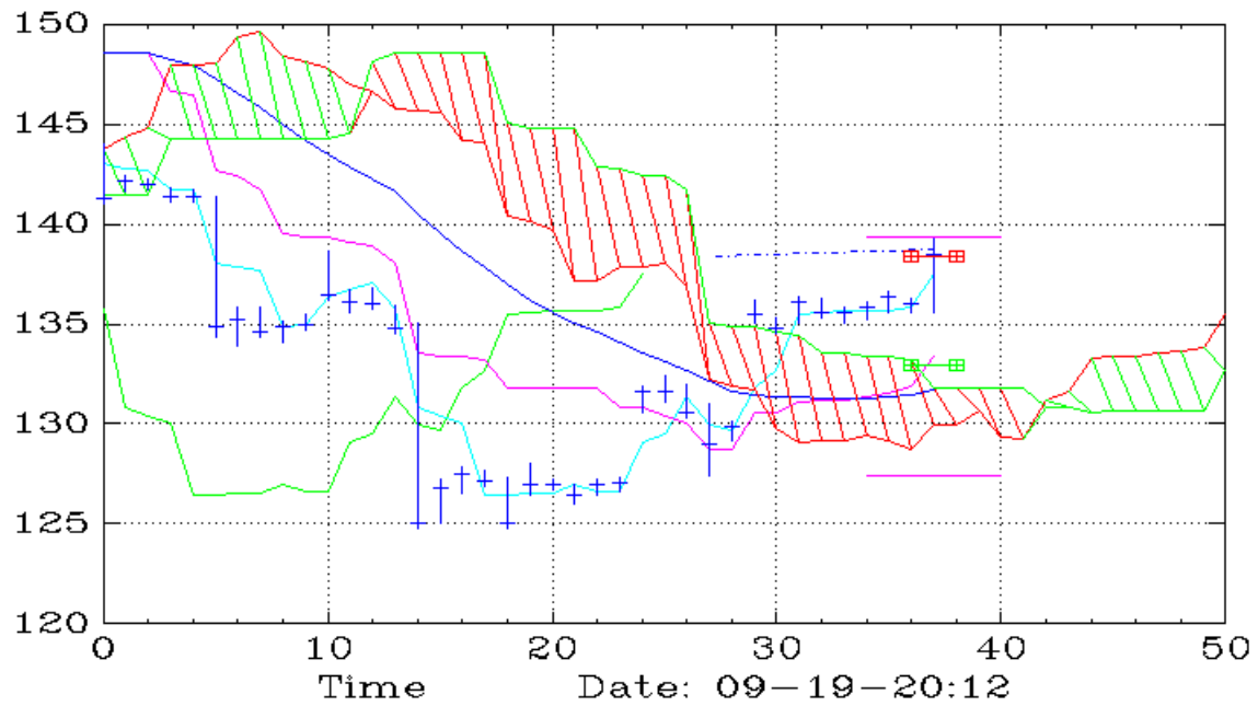
NVDU (90,Ichimoku)
