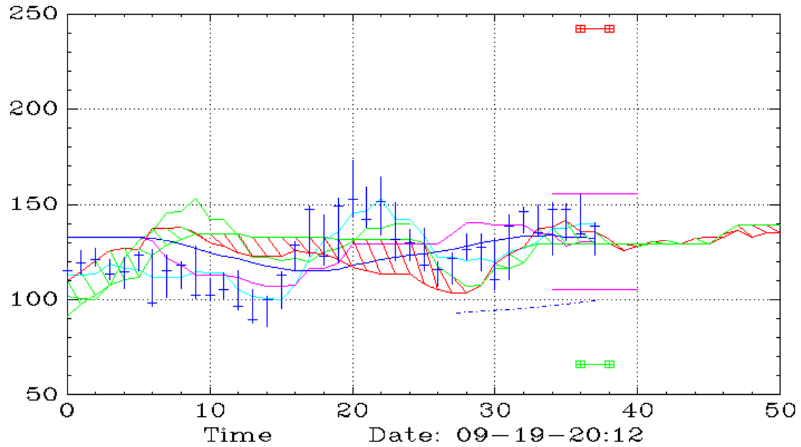
NVDU (Weekly,Ichimoku)
