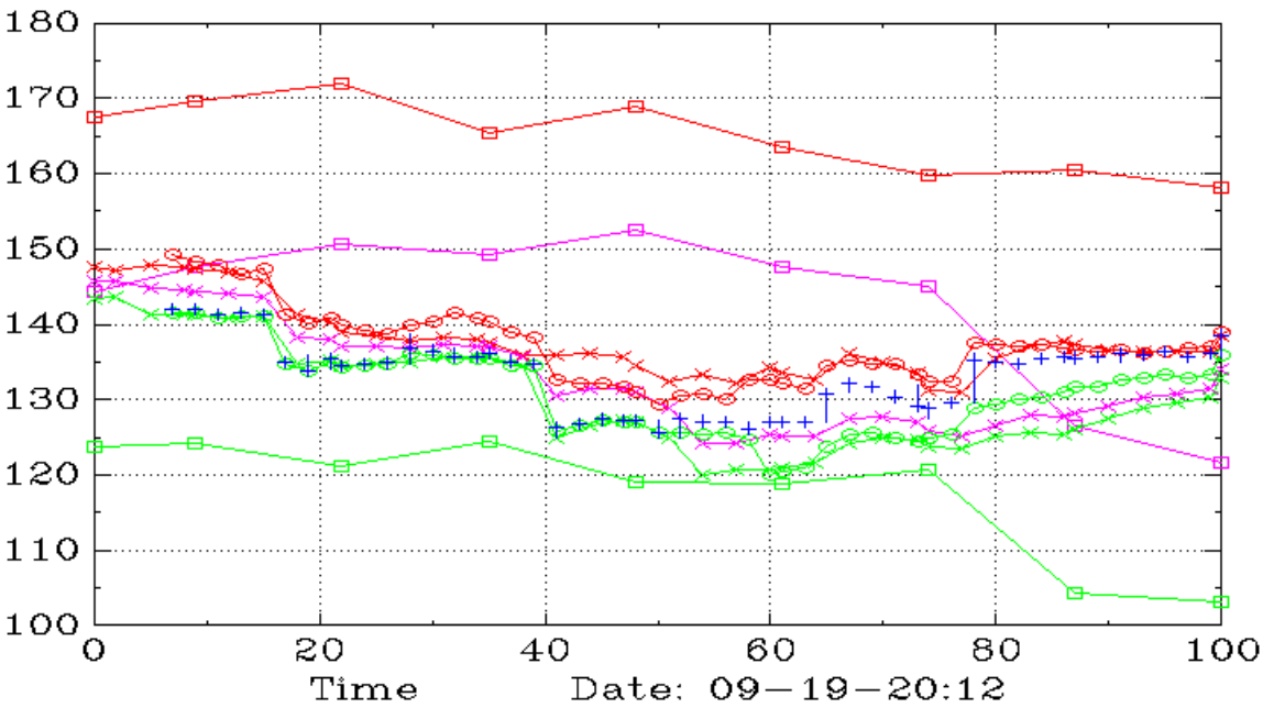
NVDU (Daily,90,60)
