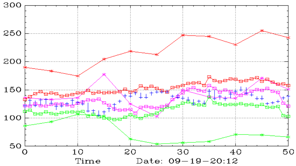
NVDU (Weekly,Daily)
