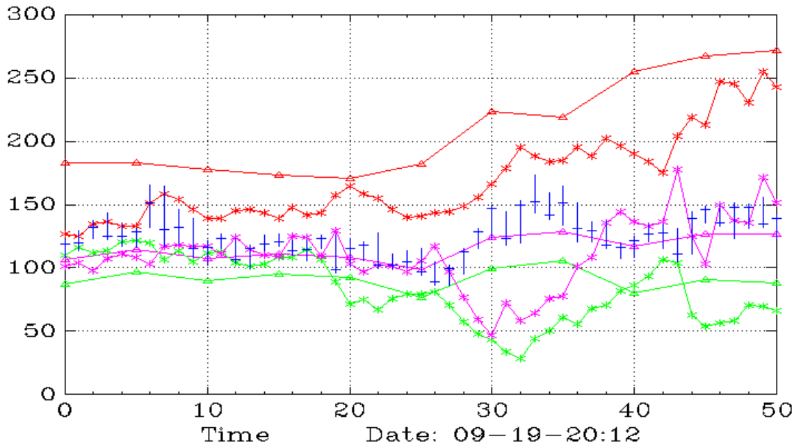
NVDU (Monthly,Weekly)
