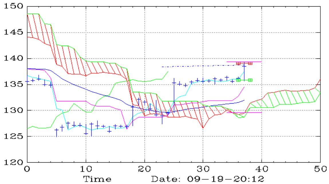
NVDU (60,Ichimoku)
