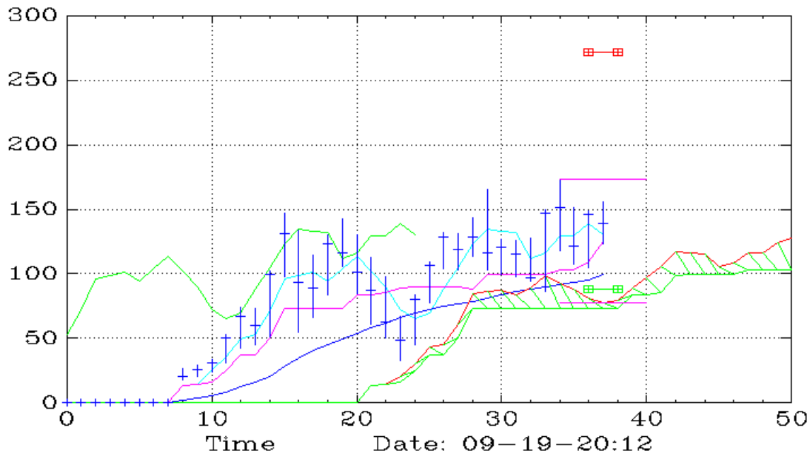
NVDU (Monthly,Ichimoku)
