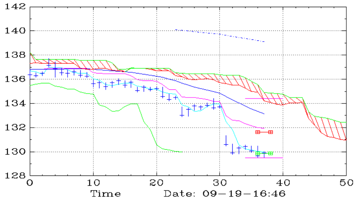
PEP (60,Ichimoku)
