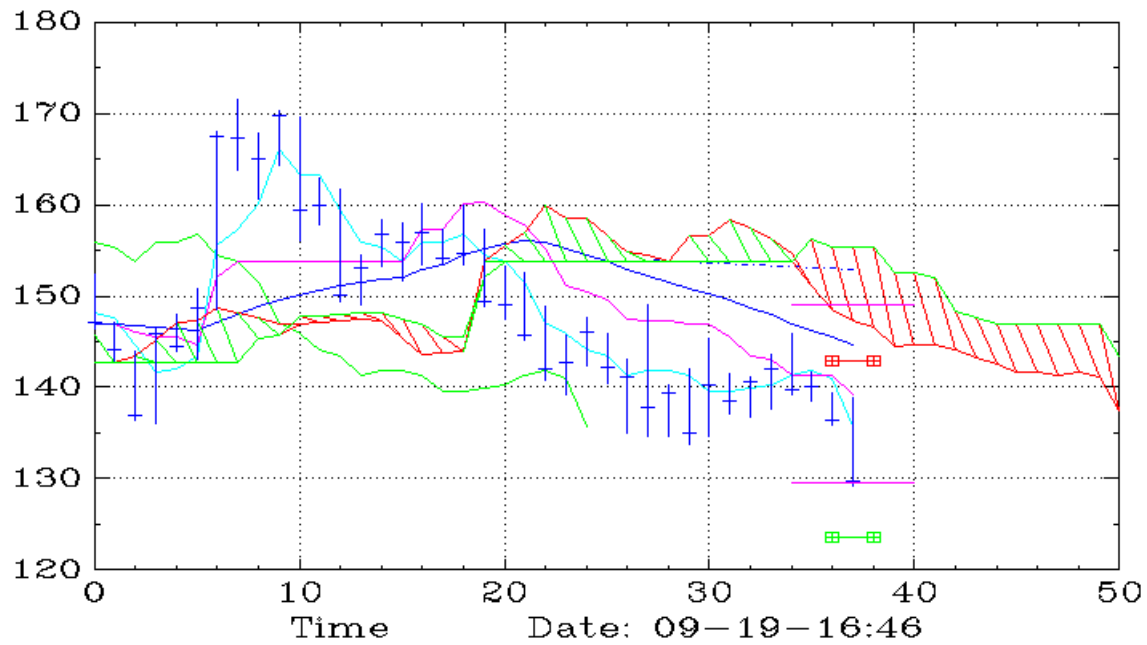
PEP (Weekly,Ichimoku)
