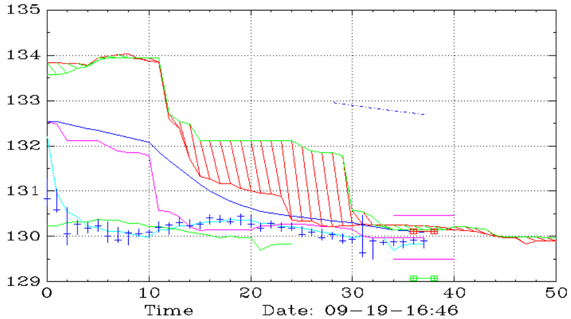
PEP (10,Ichimoku)
