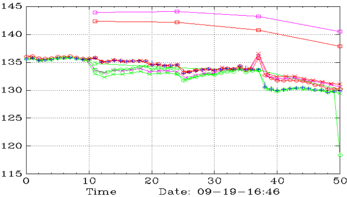
PEP (Daily,45,30)
