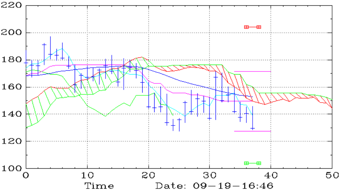
PEP (Monthly,Ichimoku)
