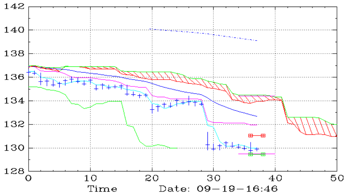
PEP (45,Ichimoku)
