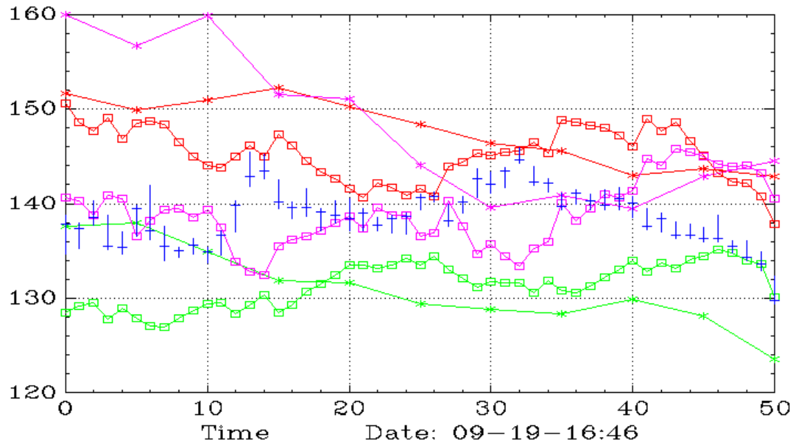
PEP (Weekly,Daily)
