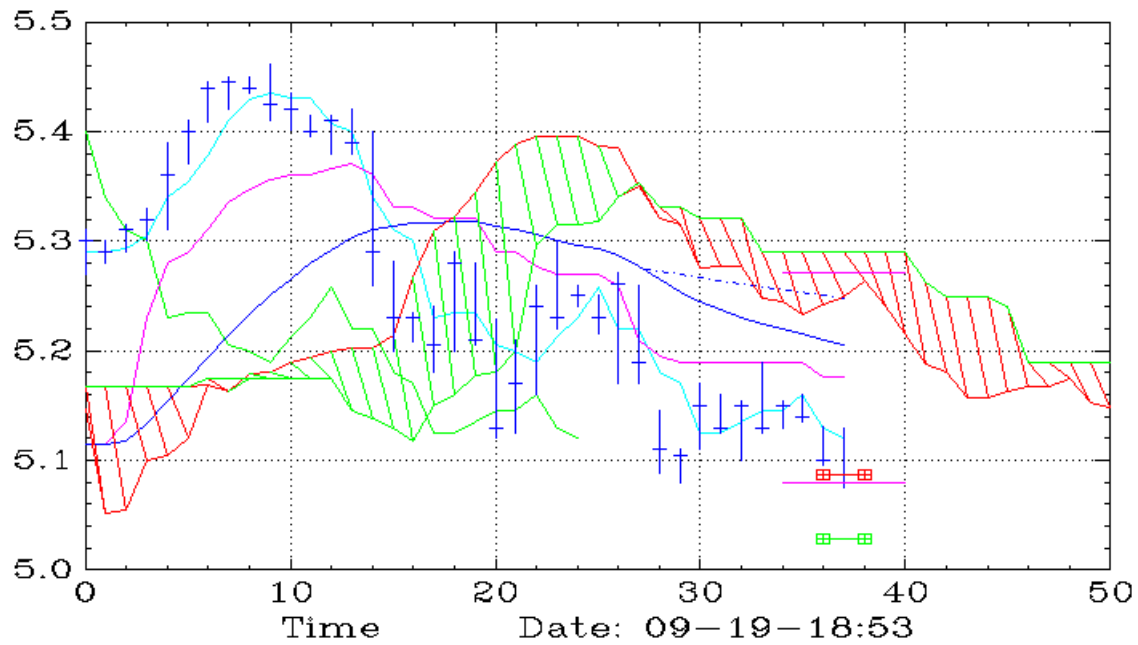
PLTD (90,Ichimoku)
