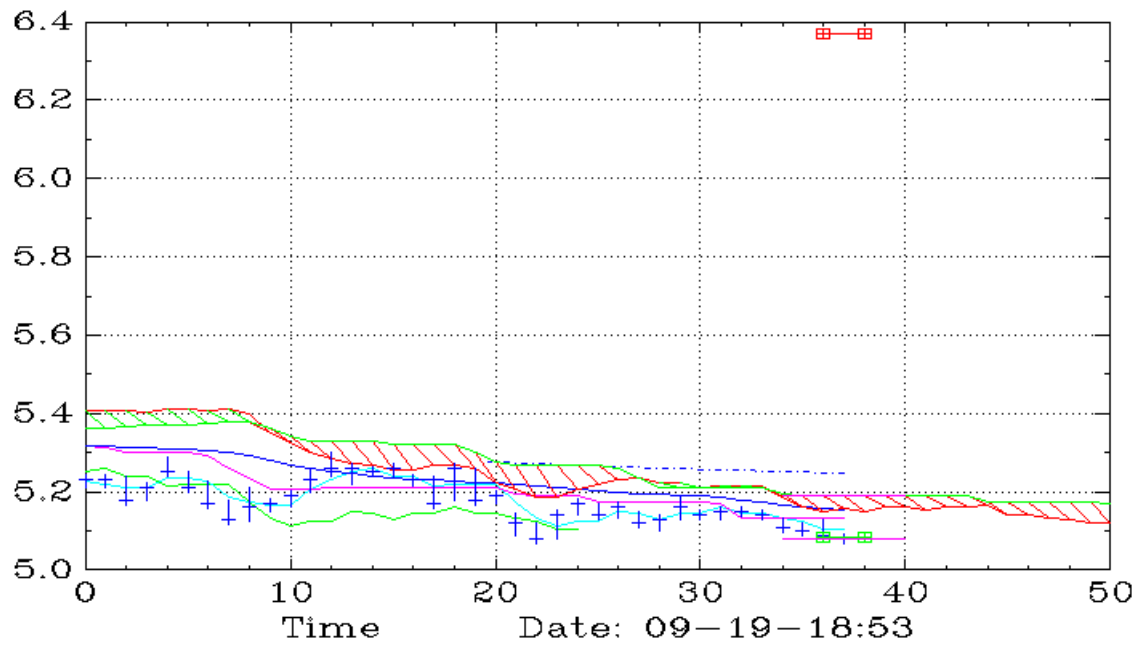
PLTD (45,Ichimoku)
