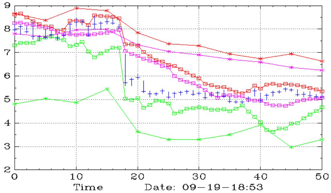
PLTD (Weekly,Daily)
