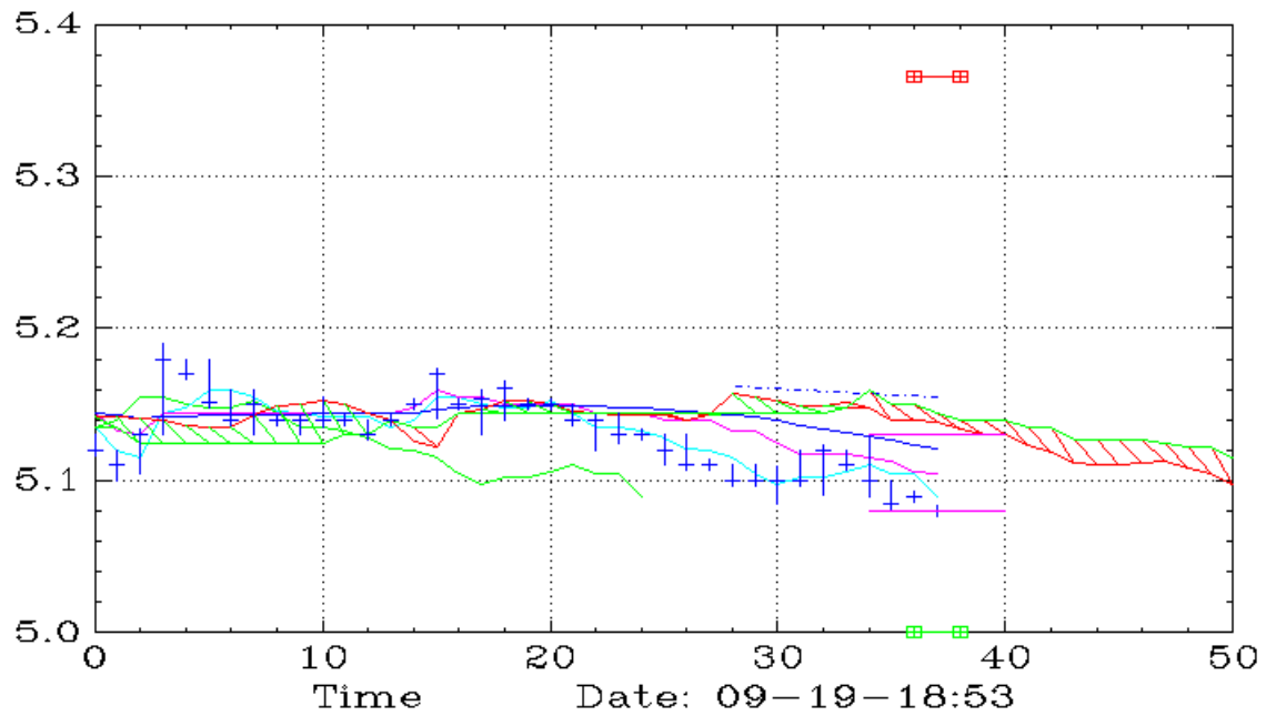
PLTD (10,Ichimoku)
