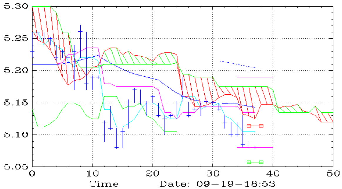
PLTD (30,Ichimoku)
