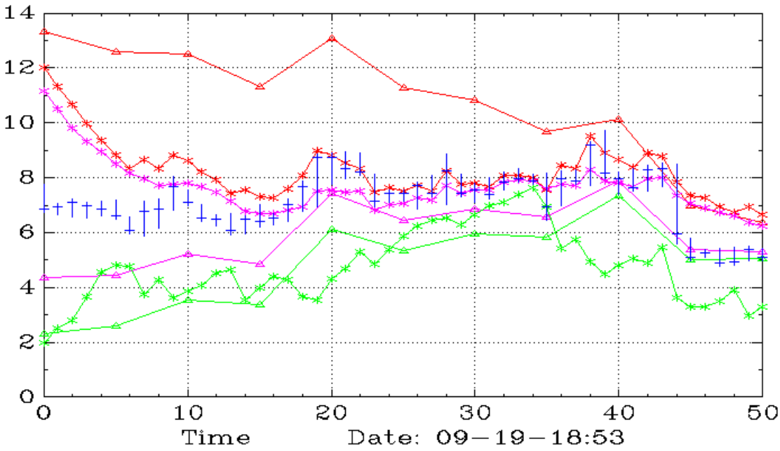
PLTD (Monthly,Weekly)
