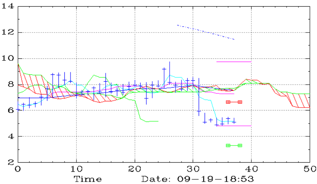
PLTD (Weekly,Ichimoku)
