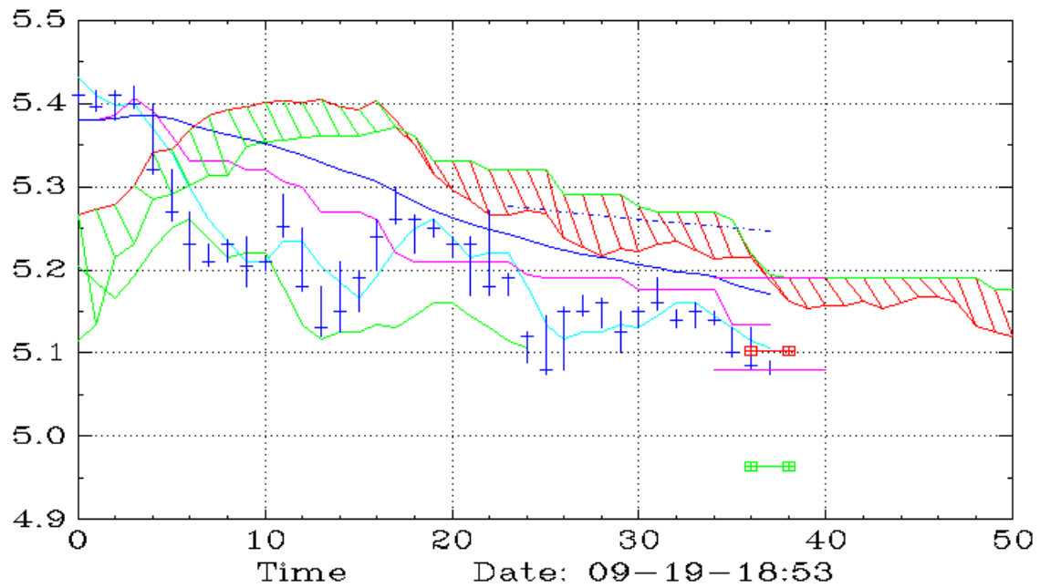
PLTD (60,Ichimoku)
