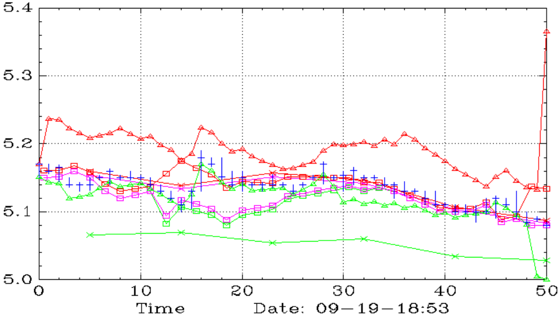
PLTD (90,15,10)
