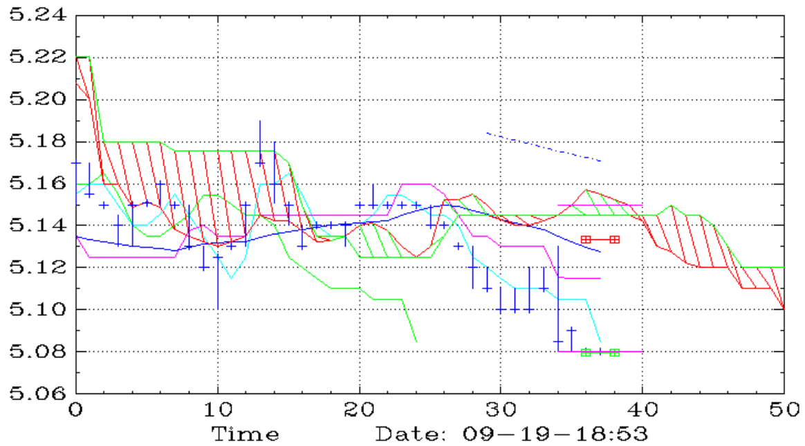
PLTD (15,Ichimoku)
