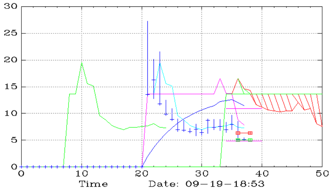
PLTD (Monthly,Ichimoku)
