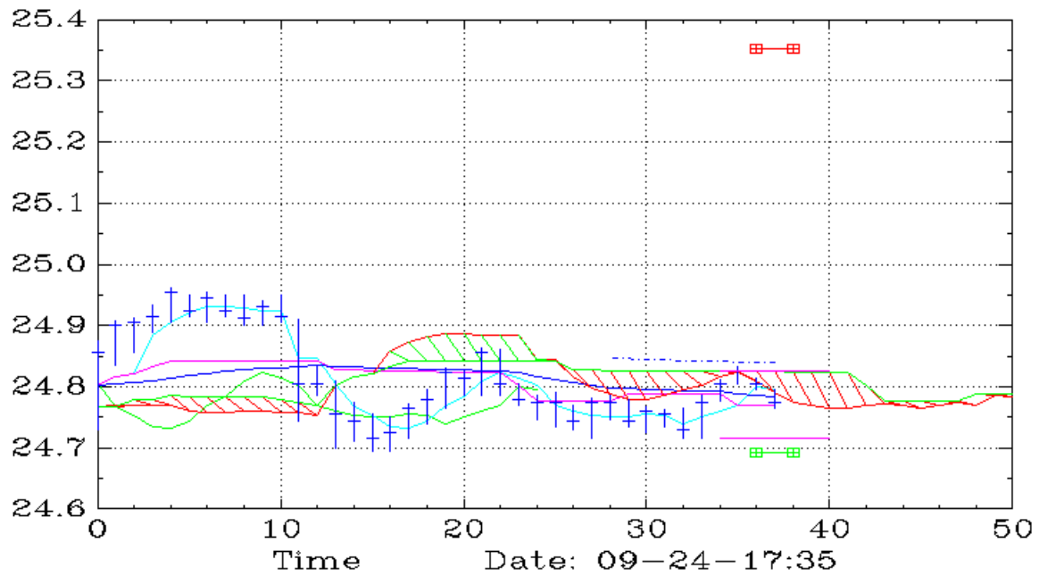
PSQ (10,Ichimoku)
