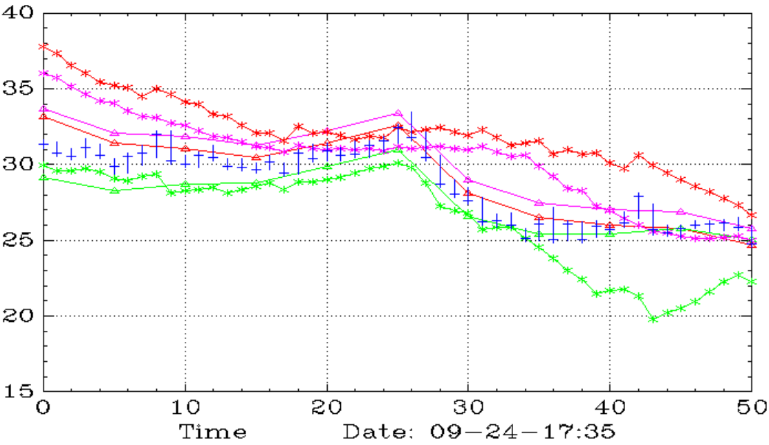
PSQ (Monthly,Weekly)
