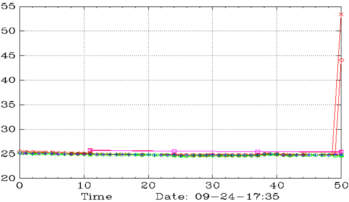
PSQ (Daily,45,30)
