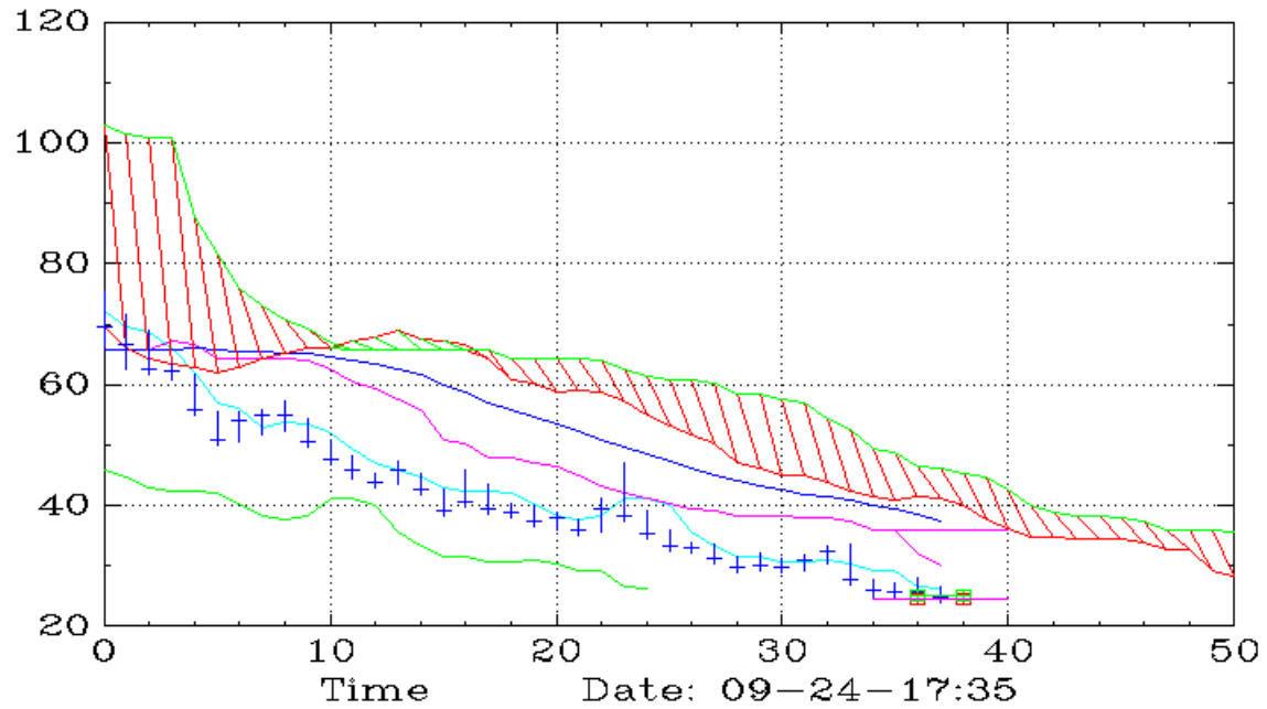
PSQ (Monthly,Ichimoku)
