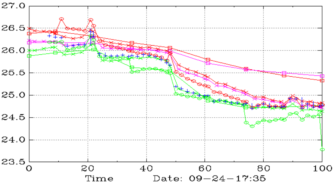
PSQ (Daily,90,60)
