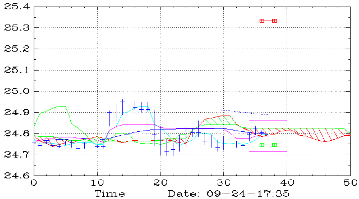
PSQ (15,Ichimoku)
