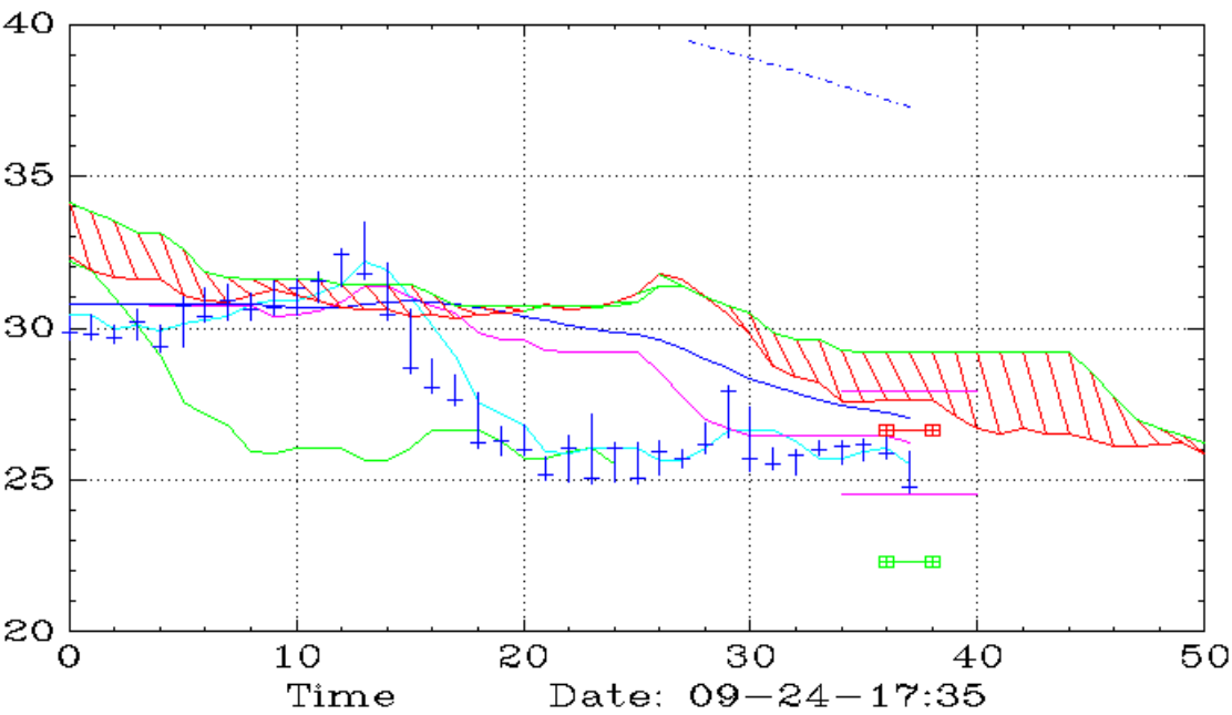
PSQ (Weekly,Ichimoku)
