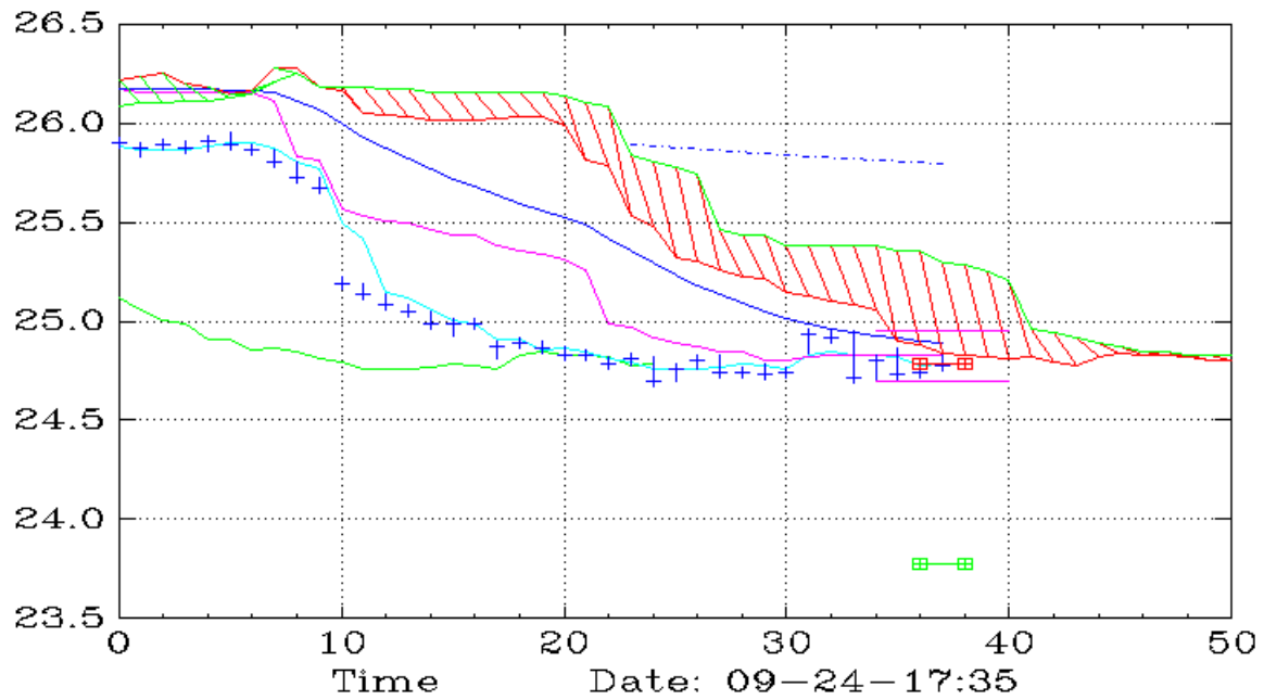
PSQ (60,Ichimoku)
