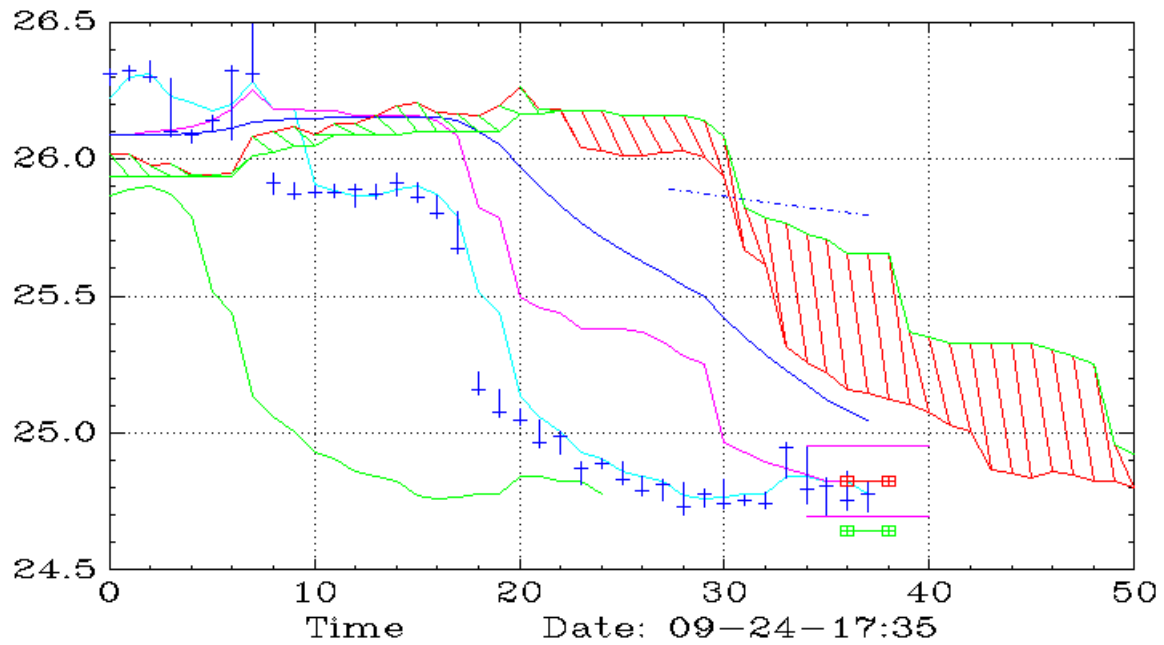
PSQ (90,Ichimoku)
