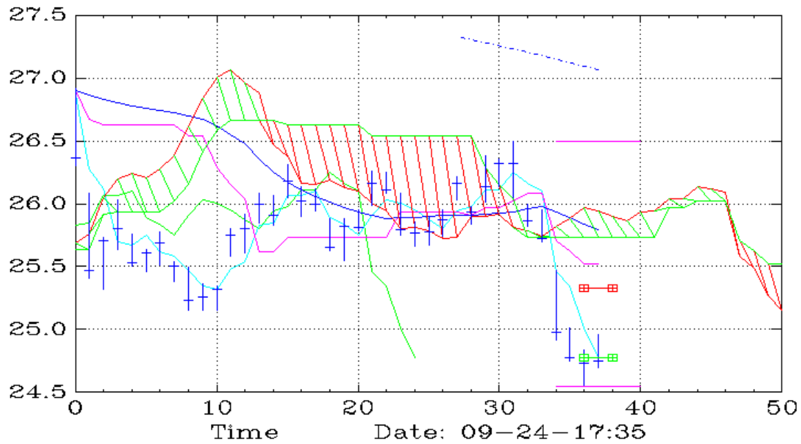
PSQ (Daily,Ichimoku)
