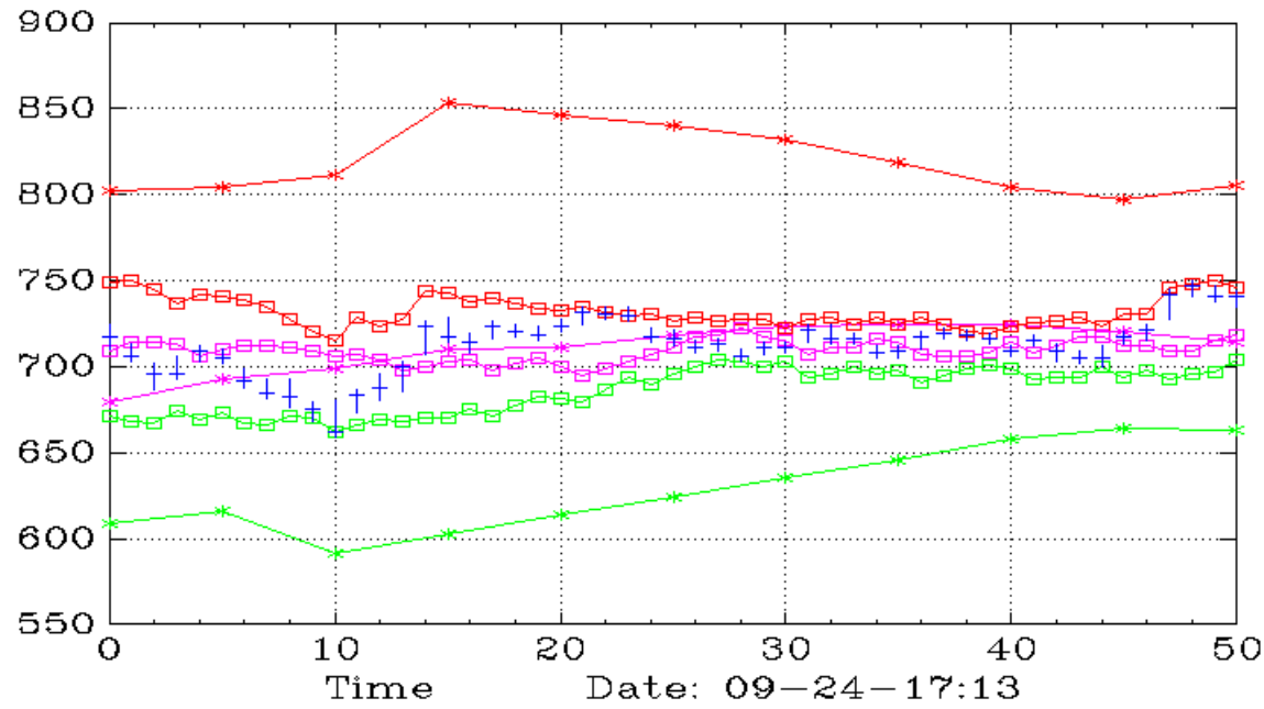
QQQ (Weekly,Daily)
