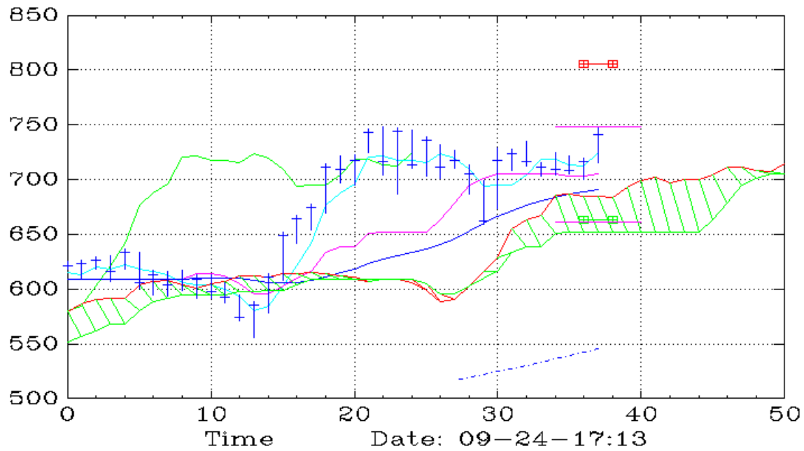
QQQ (Weekly,Ichimoku)
