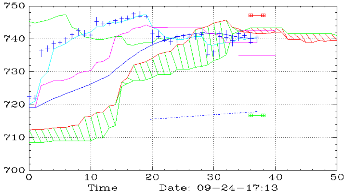
QQQ (45,Ichimoku)
