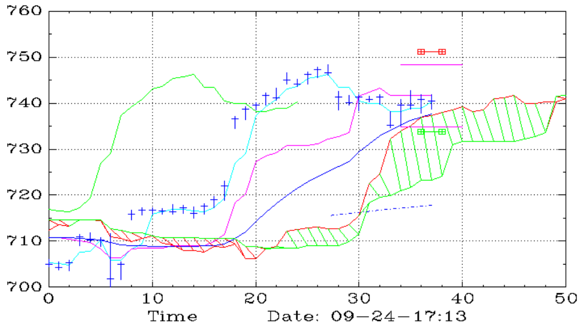
QQQ (90,Ichimoku)
