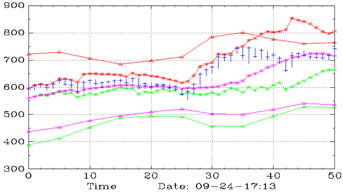
QQQ (Monthly,Weekly)
