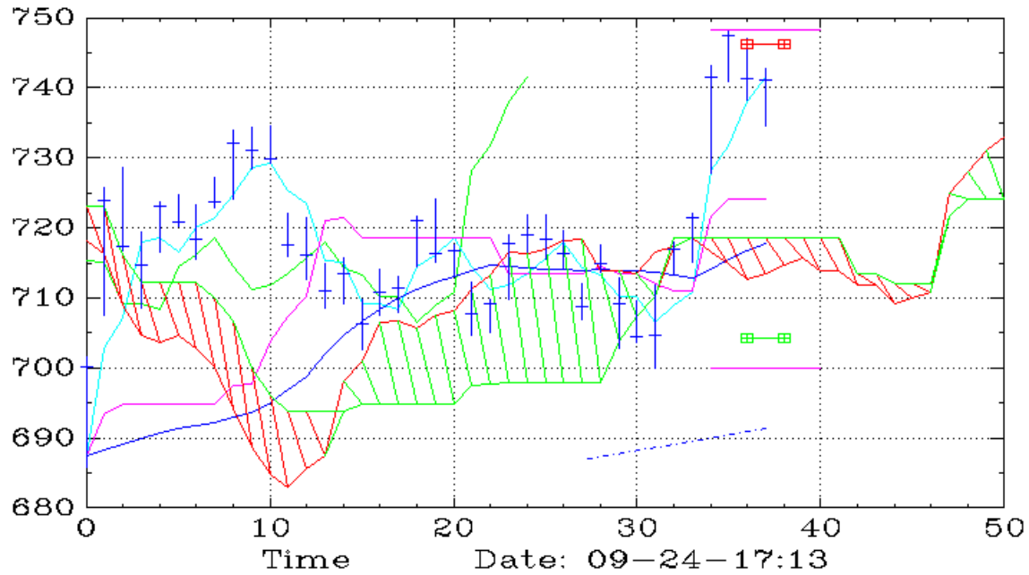
QQQ (Daily,Ichimoku)
