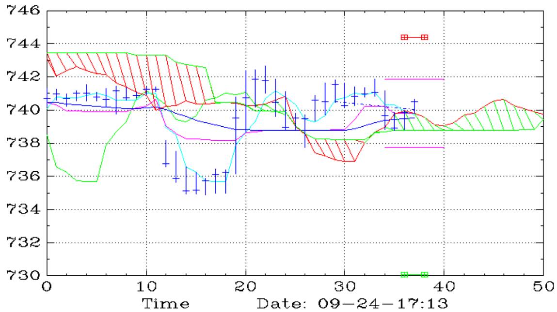
QQQ (15,Ichimoku)
