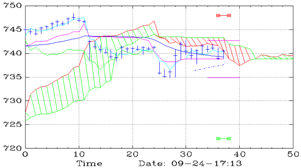
QQQ (30,Ichimoku)
