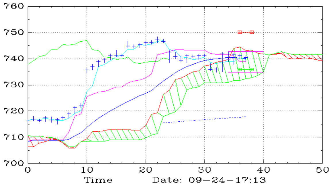
QQQ (60,Ichimoku)
