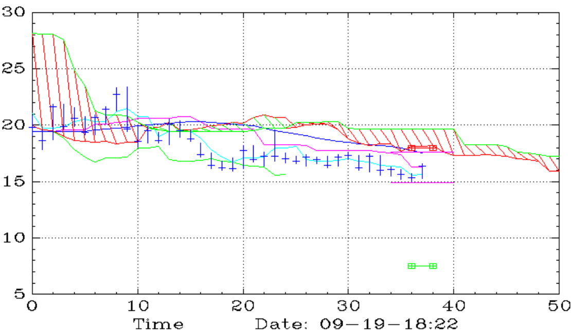
REK (Monthly,Ichimoku)
