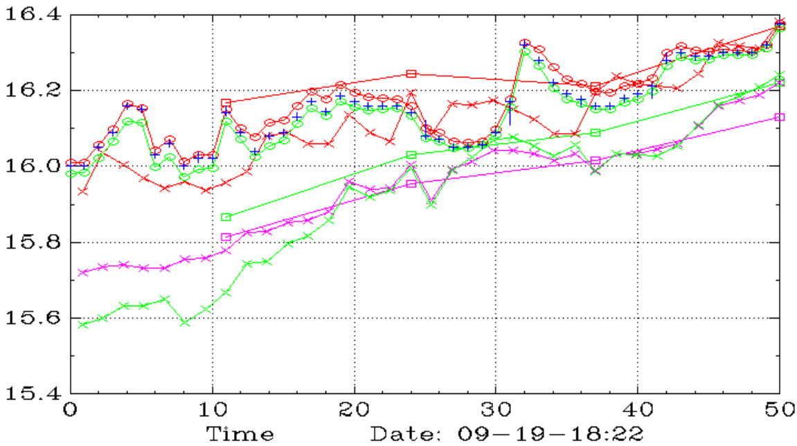
REK (Daily,45,30)
