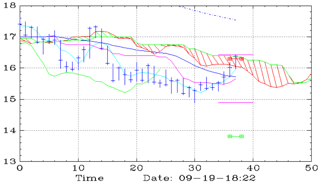
REK (Weekly,Ichimoku)
