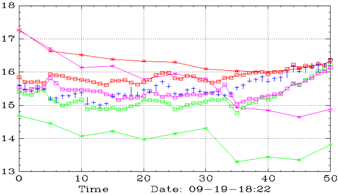
REK (Weekly,Daily)
