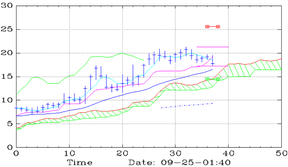
RLAY (Weekly,Ichimoku)
