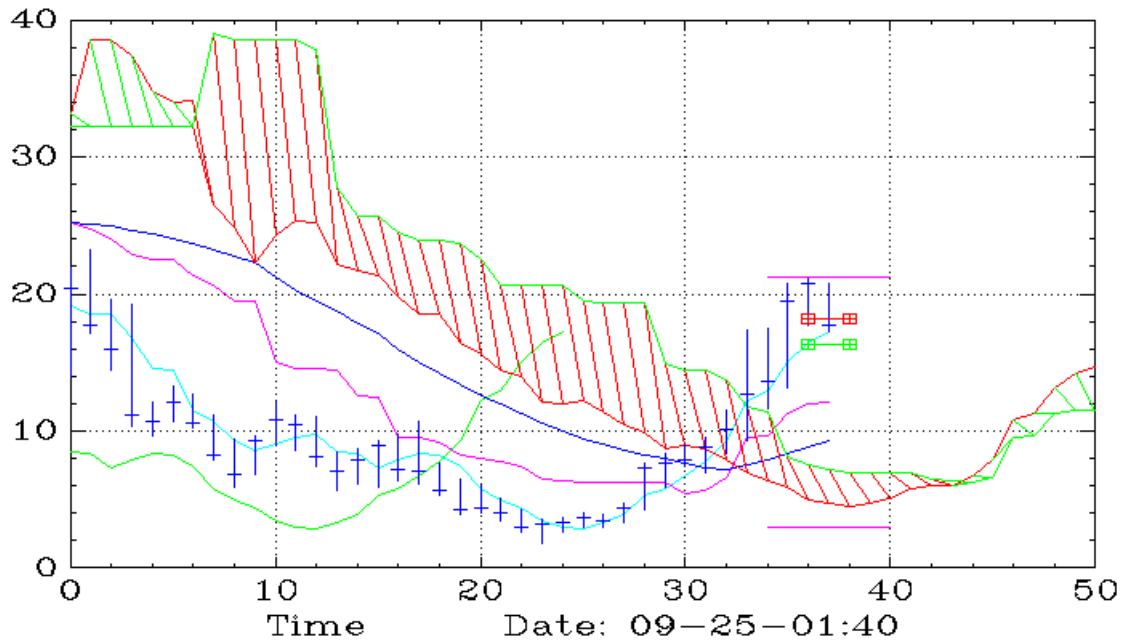
RLAY (Monthly,Ichimoku)
