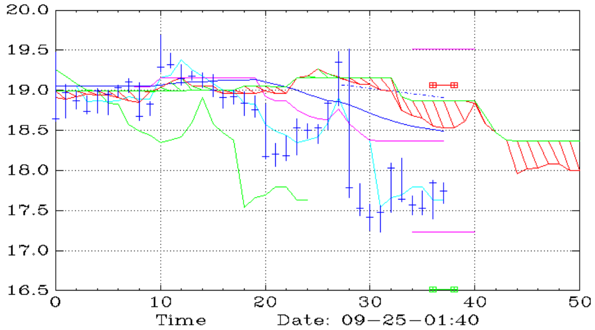
RLAY (90,Ichimoku)
