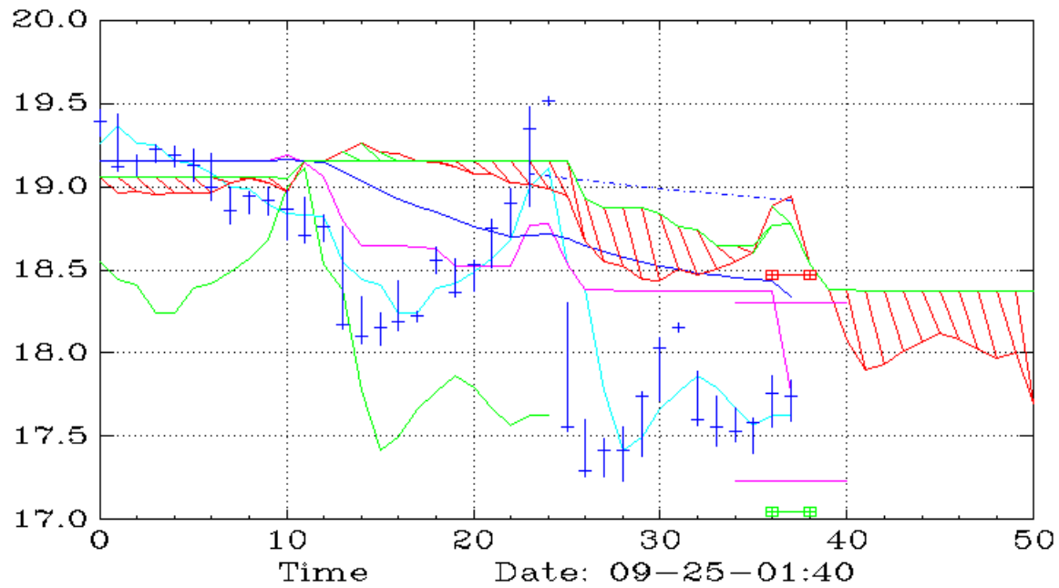
RLAY (60,Ichimoku)
