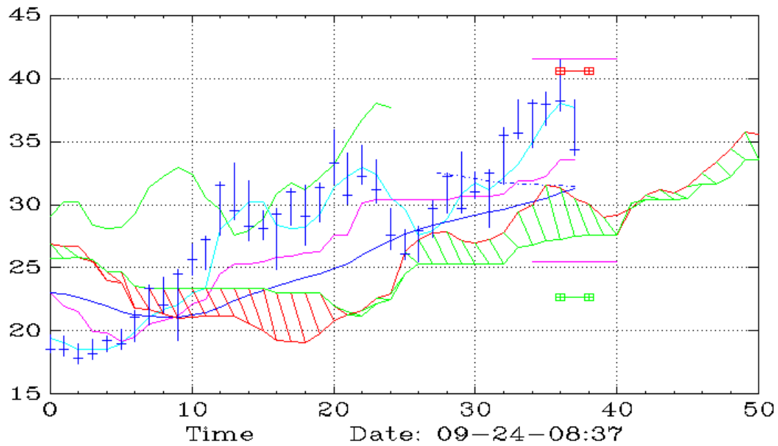
SM (Weekly,Ichimoku)
