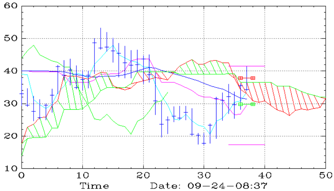
SM (Monthly,Ichimoku)
