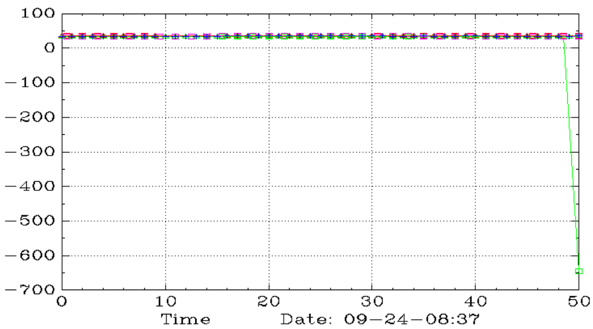
SM (90,15,10)
