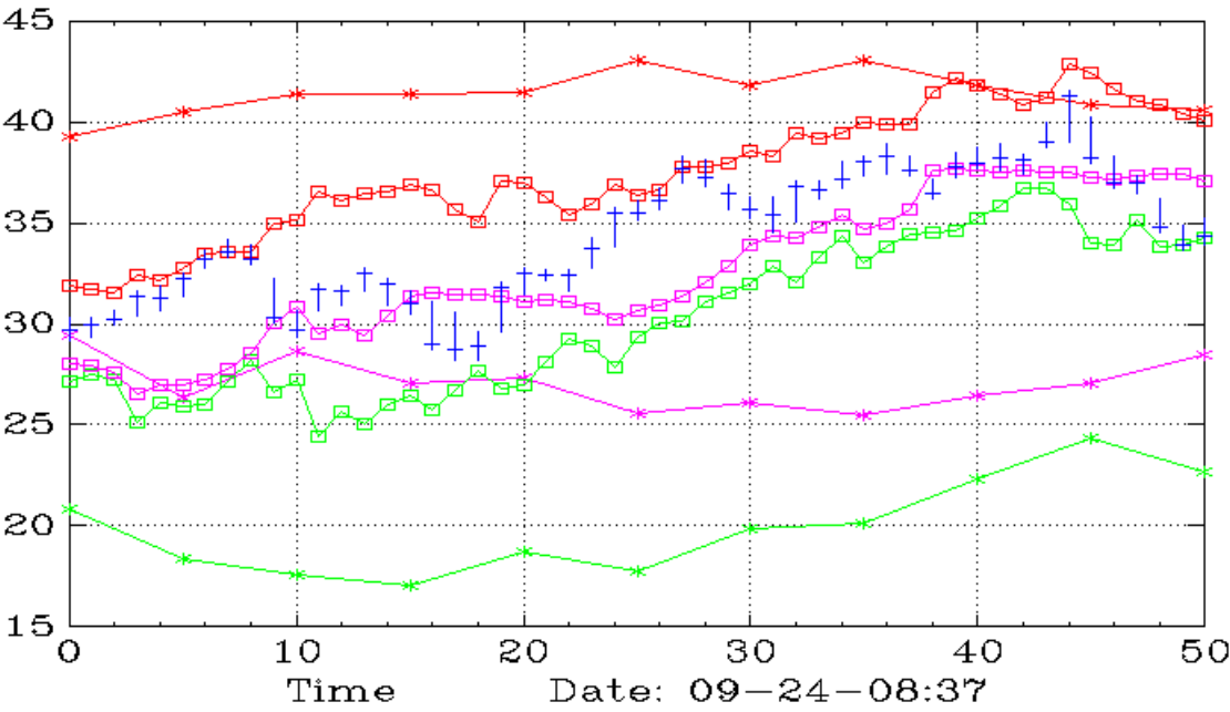
SM (Weekly,Daily)
