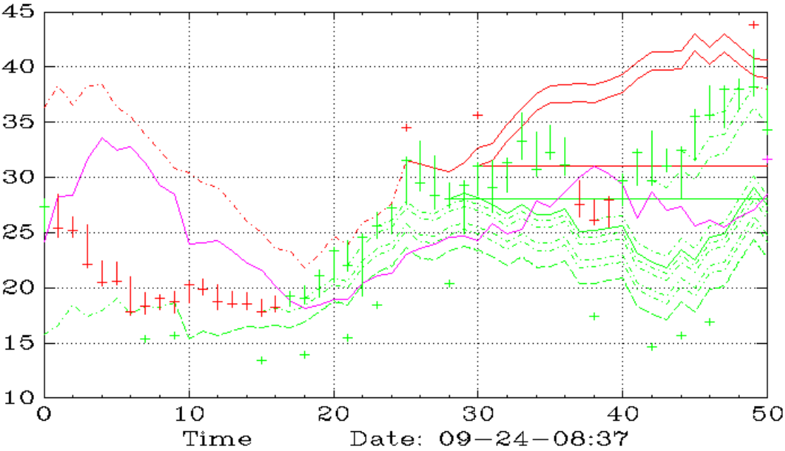
SM (Weekly,SAR)
