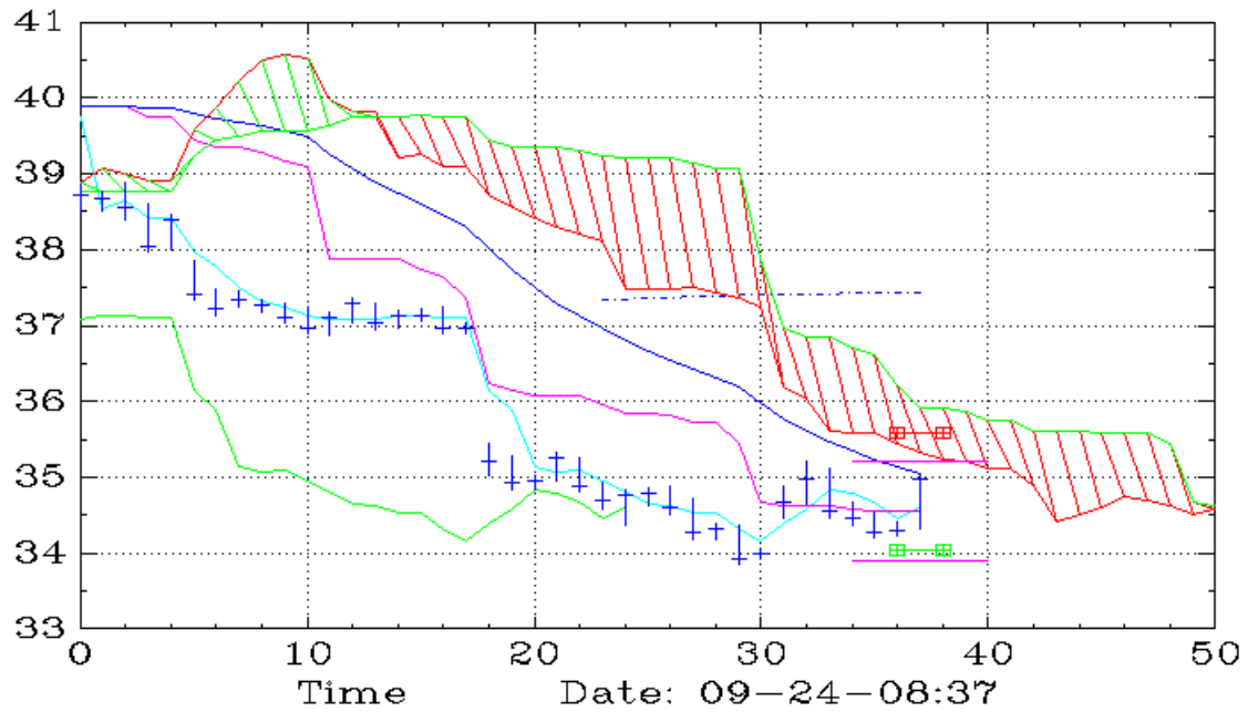
SM (60,Ichimoku)
