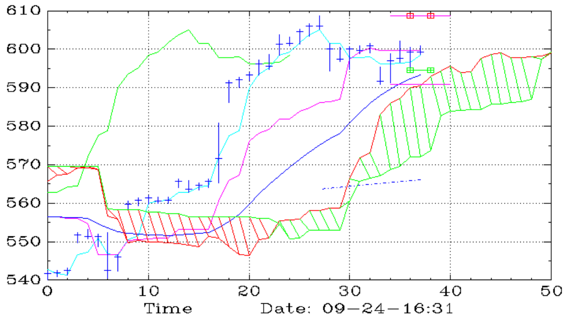
SMH (90,Ichimoku)
