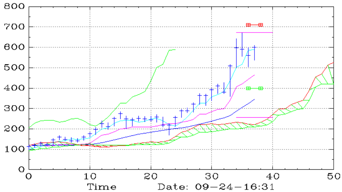
SMH (Monthly,Ichimoku)
