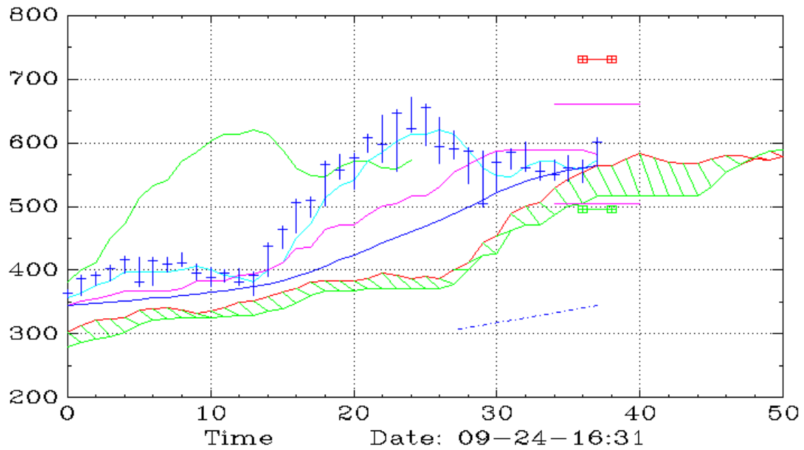
SMH (Weekly,Ichimoku)
