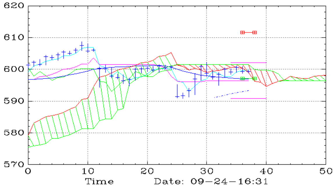
SMH (30,Ichimoku)
