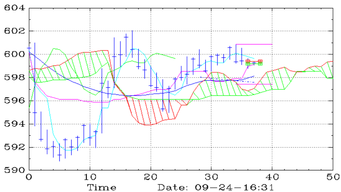
SMH (10,Ichimoku)
