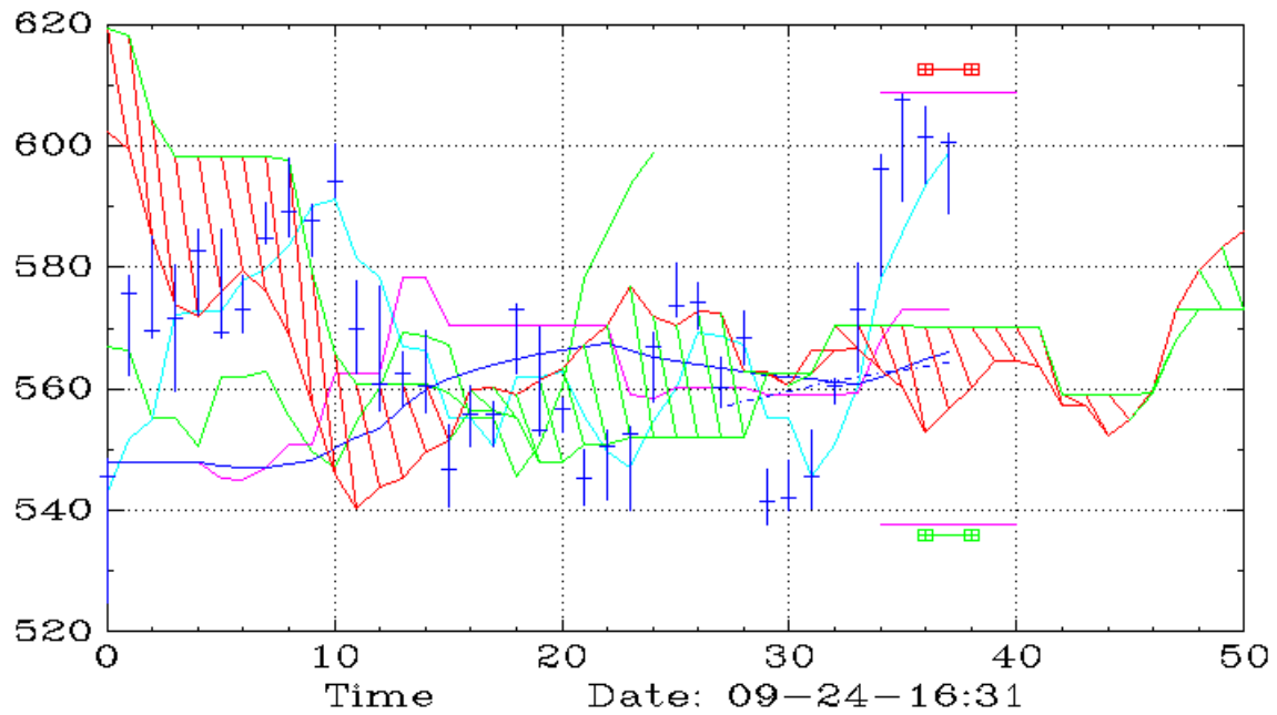
SMH (Daily,Ichimoku)
