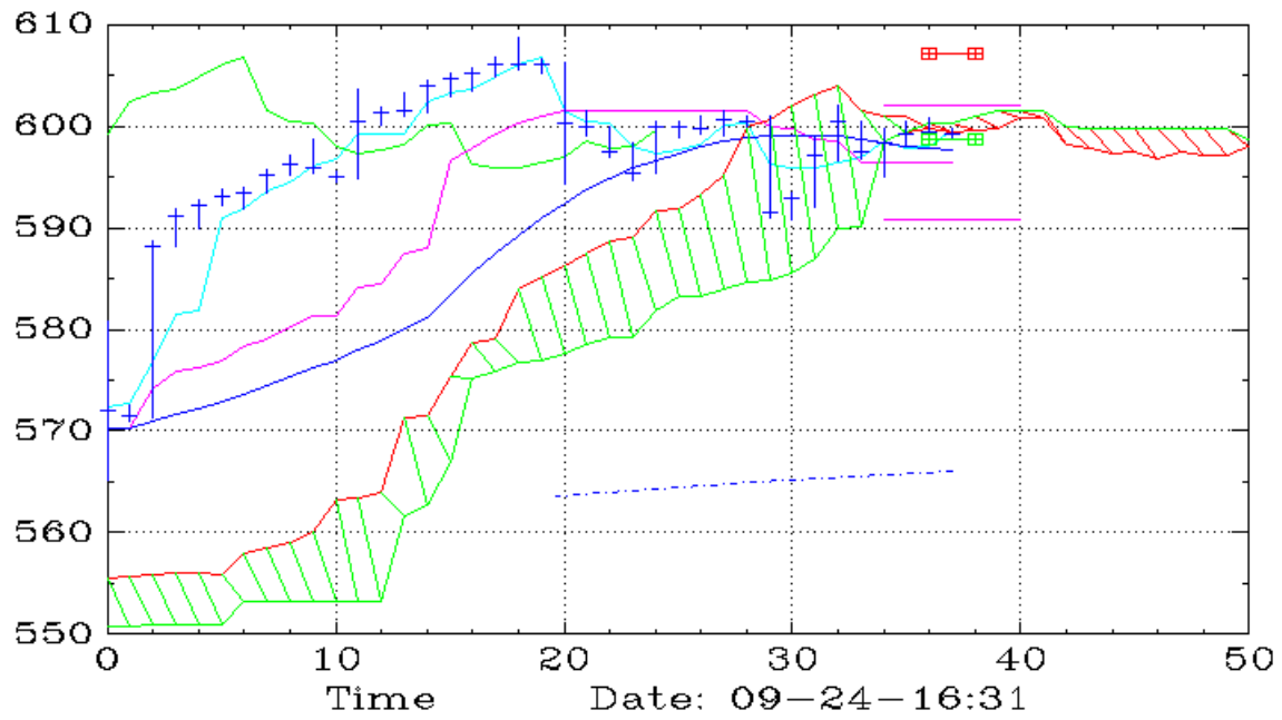
SMH (45,Ichimoku)
