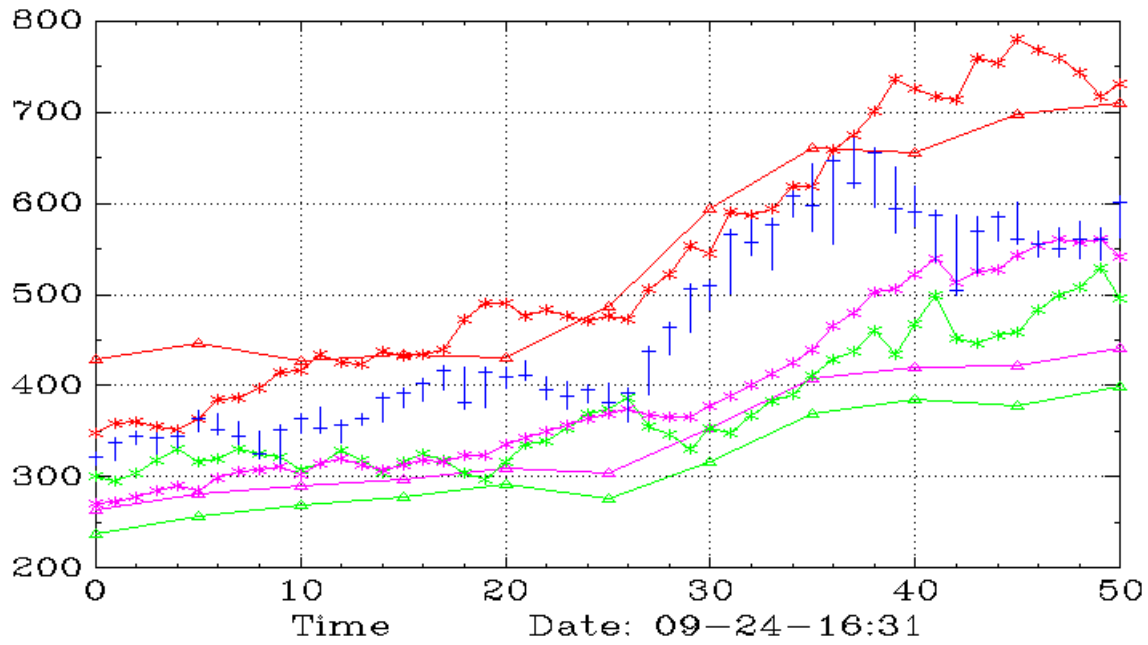
SMH (Monthly,Weekly)
