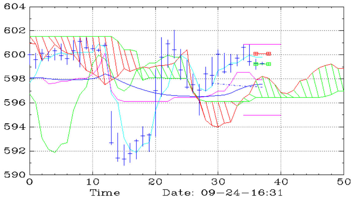
SMH (15,Ichimoku)
