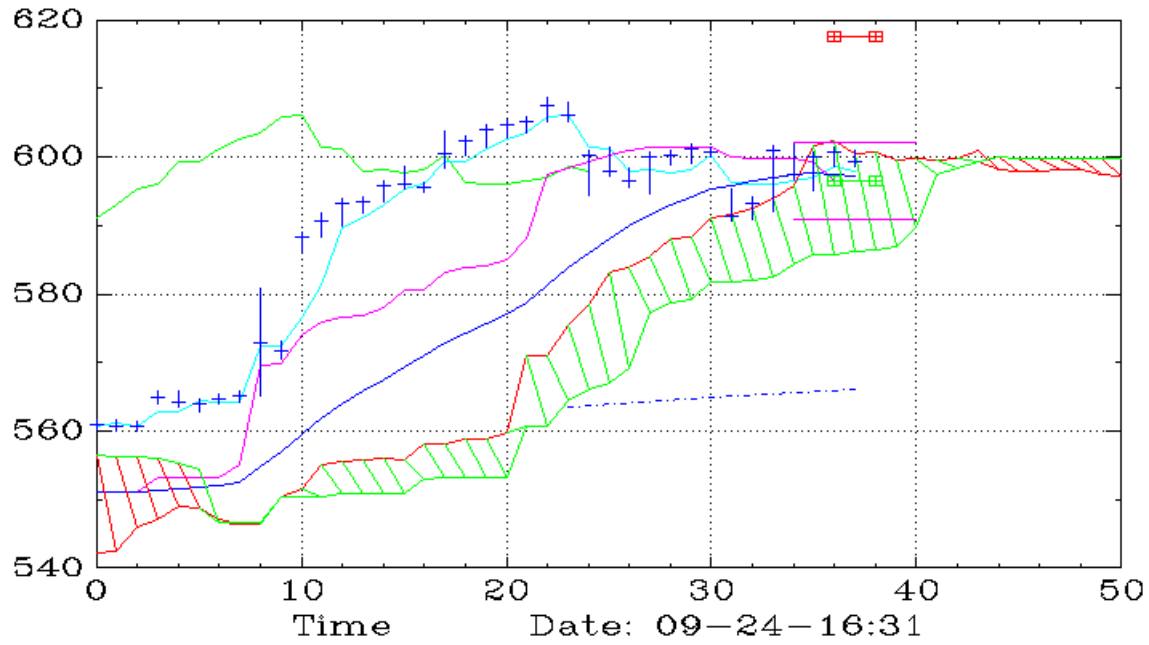
SMH (60,Ichimoku)
