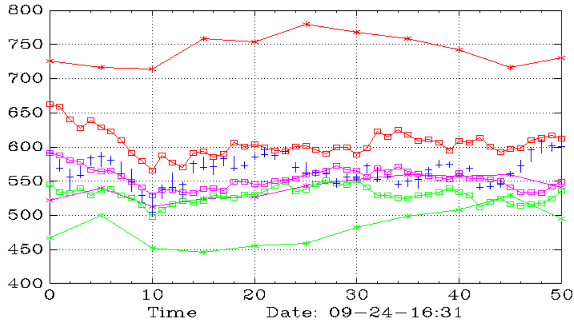
SMH (Weekly,Daily)
