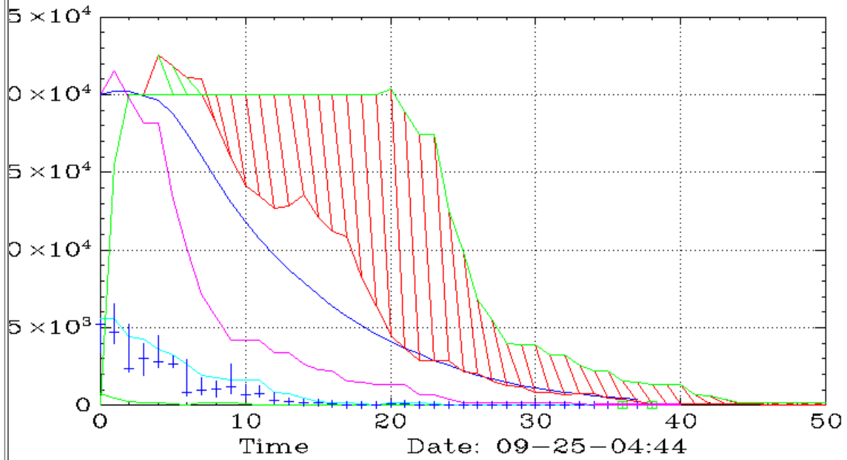
SPRC (Monthly,Ichimoku)
