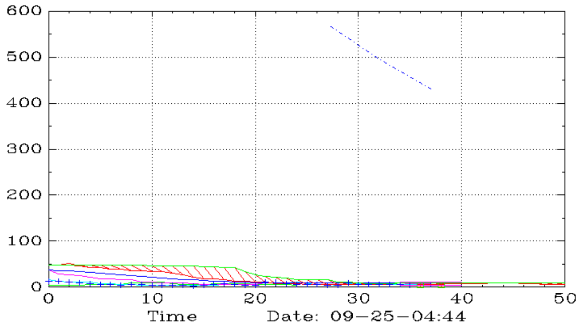
SPRC (Weekly,Ichimoku)
