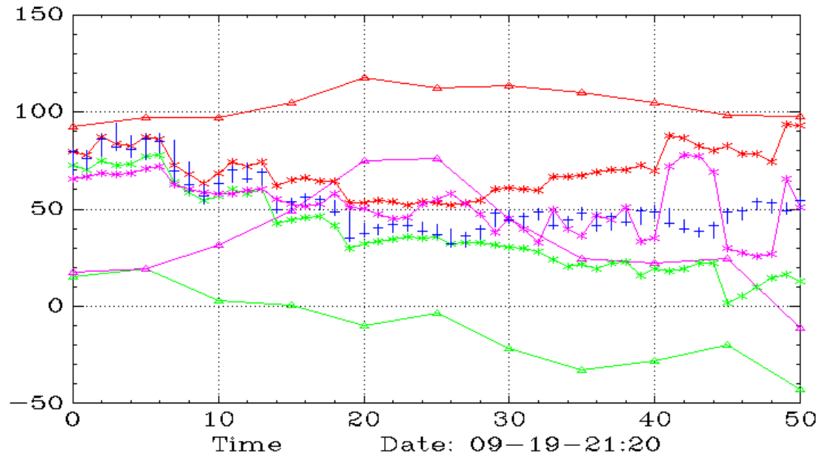
TARK (Monthly,Weekly)
