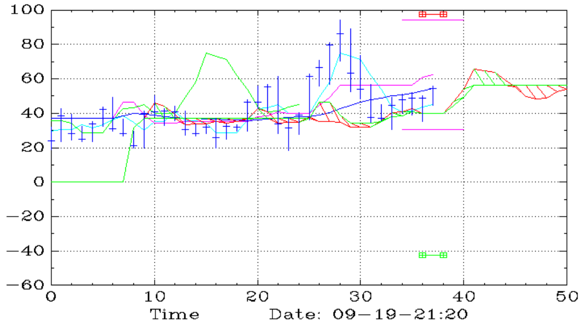
TARK (Monthly,Ichimoku)
