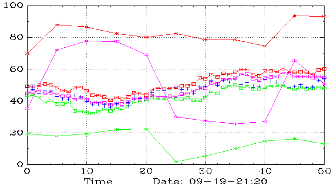
TARK (Weekly,Daily)
