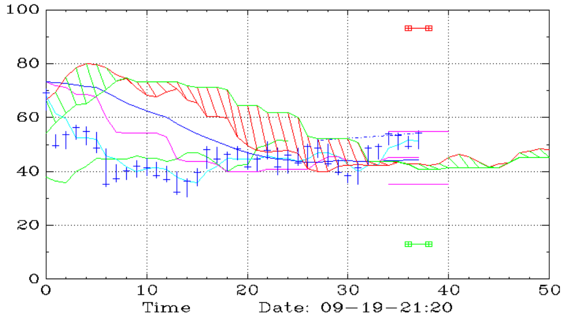
TARK (Weekly,Ichimoku)
