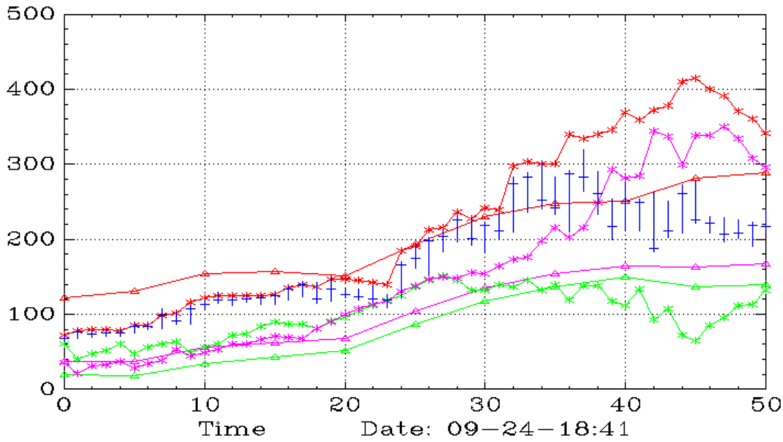
TSEM (Monthly,Weekly)
