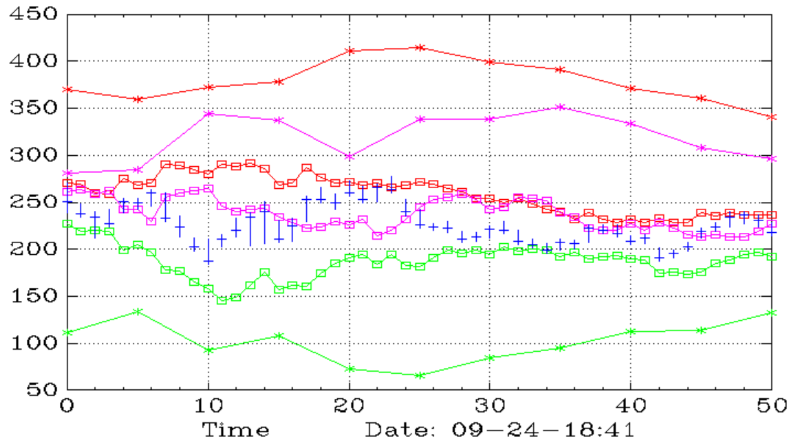
TSEM (Weekly,Daily)
