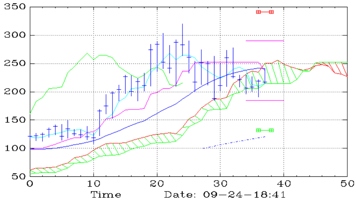
TSEM (Weekly,Ichimoku)
