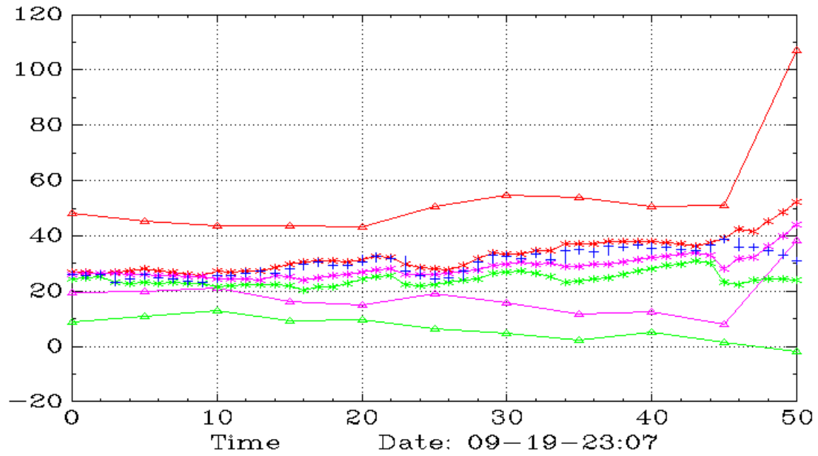
UMDD (Monthly,Weekly)
