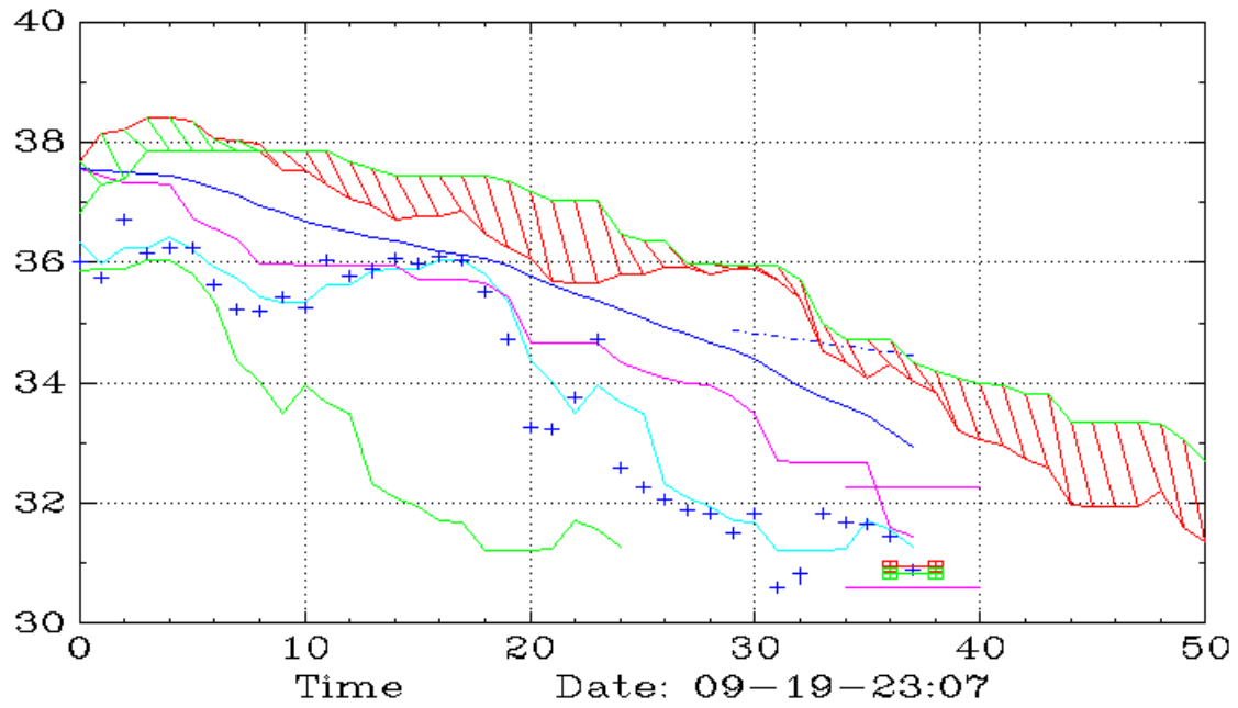
UMDD (15,Ichimoku)
