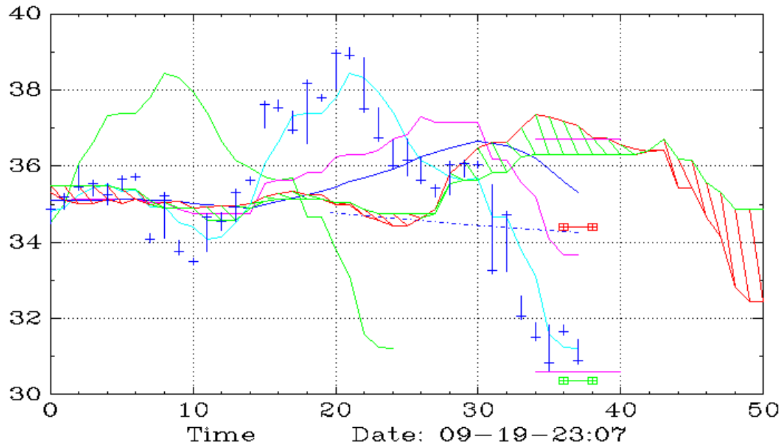
UMDD (45,Ichimoku)
