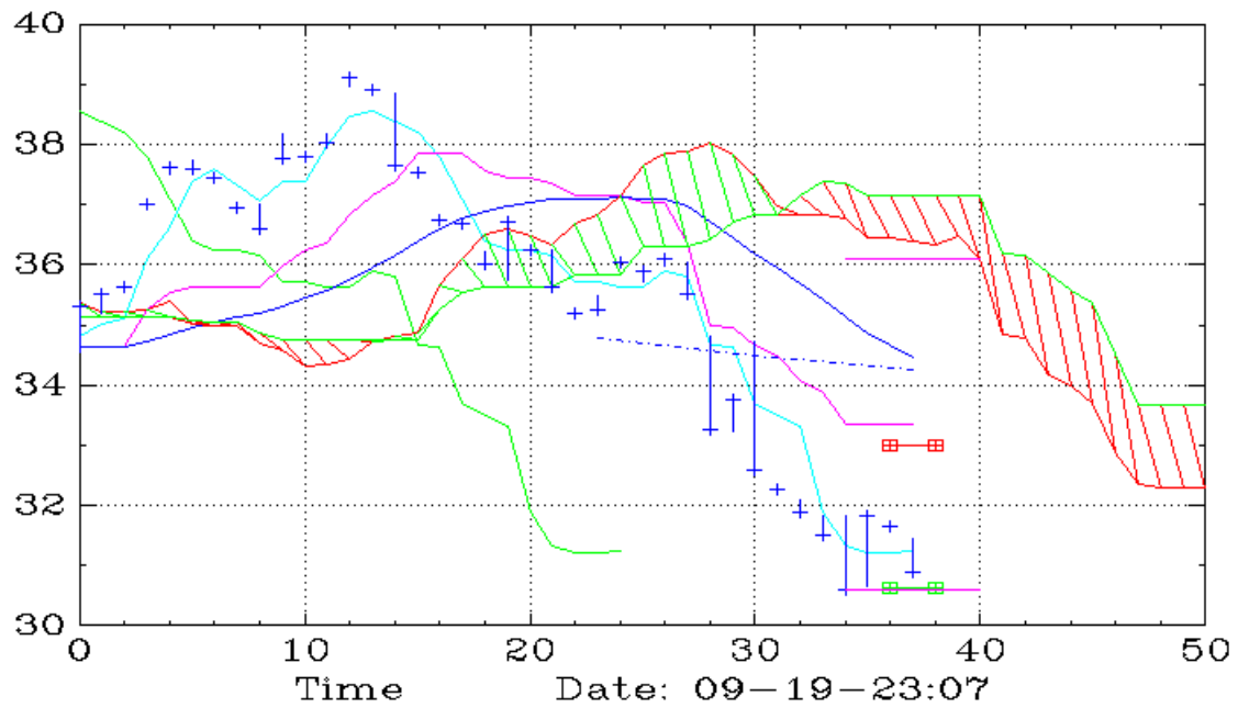
UMDD (60,Ichimoku)
