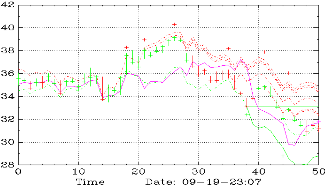
UMDD (Daily,SAR)
