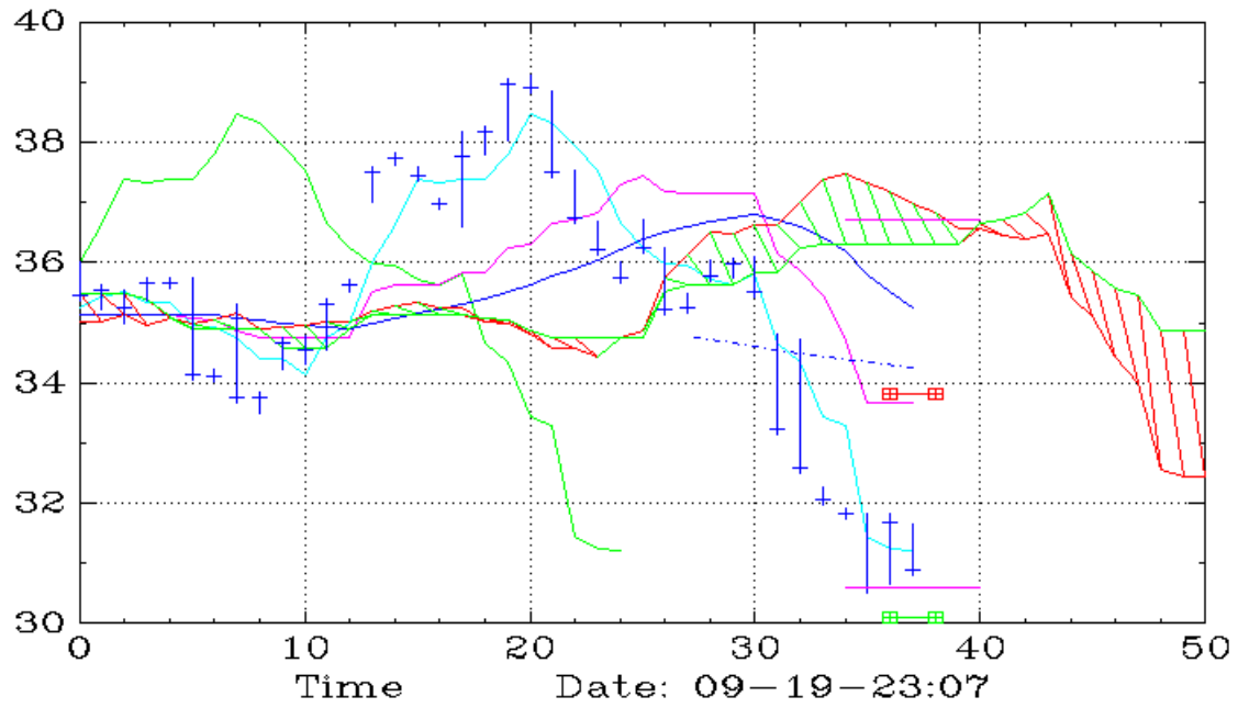
UMDD (90,Ichimoku)
