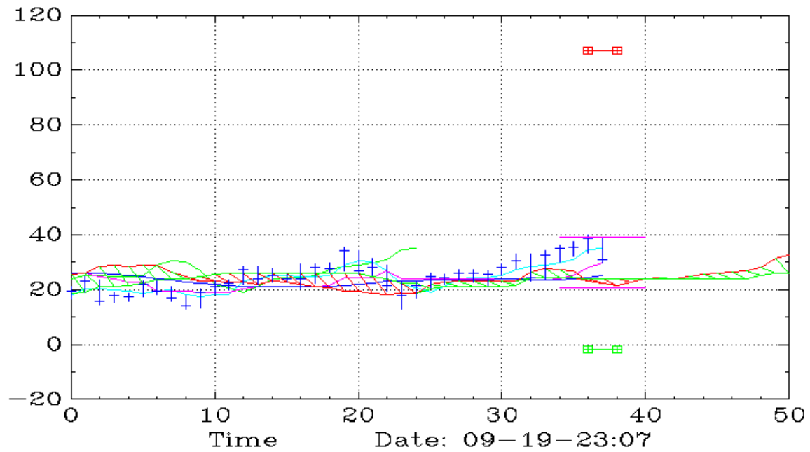
UMDD (Monthly,Ichimoku)
