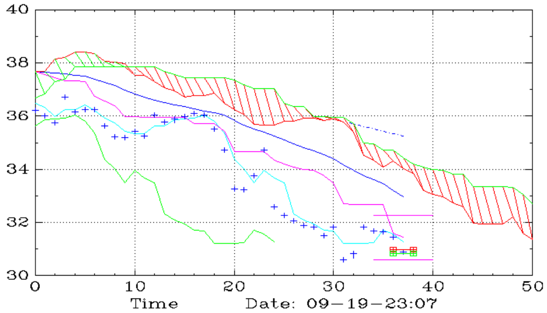
UMDD (30,Ichimoku)
