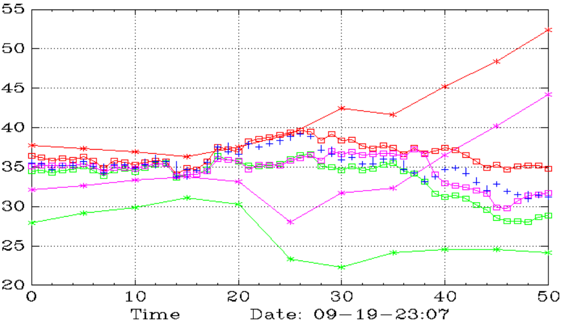
UMDD (Weekly,Daily)
