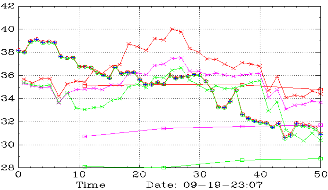
UMDD (Daily,45,30)
