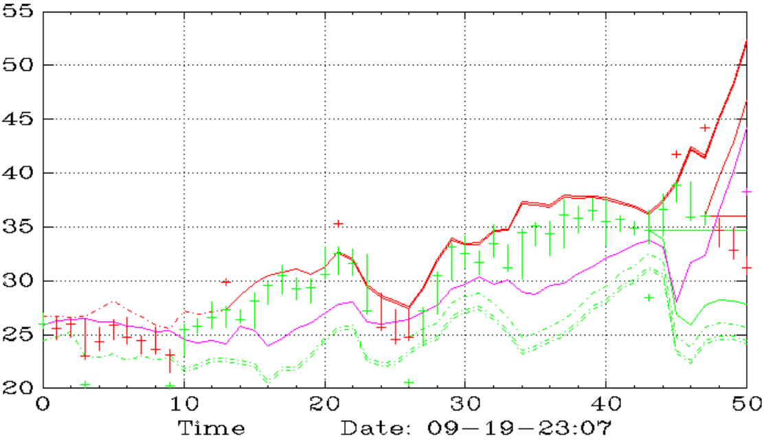
UMDD (Weekly,SAR)
