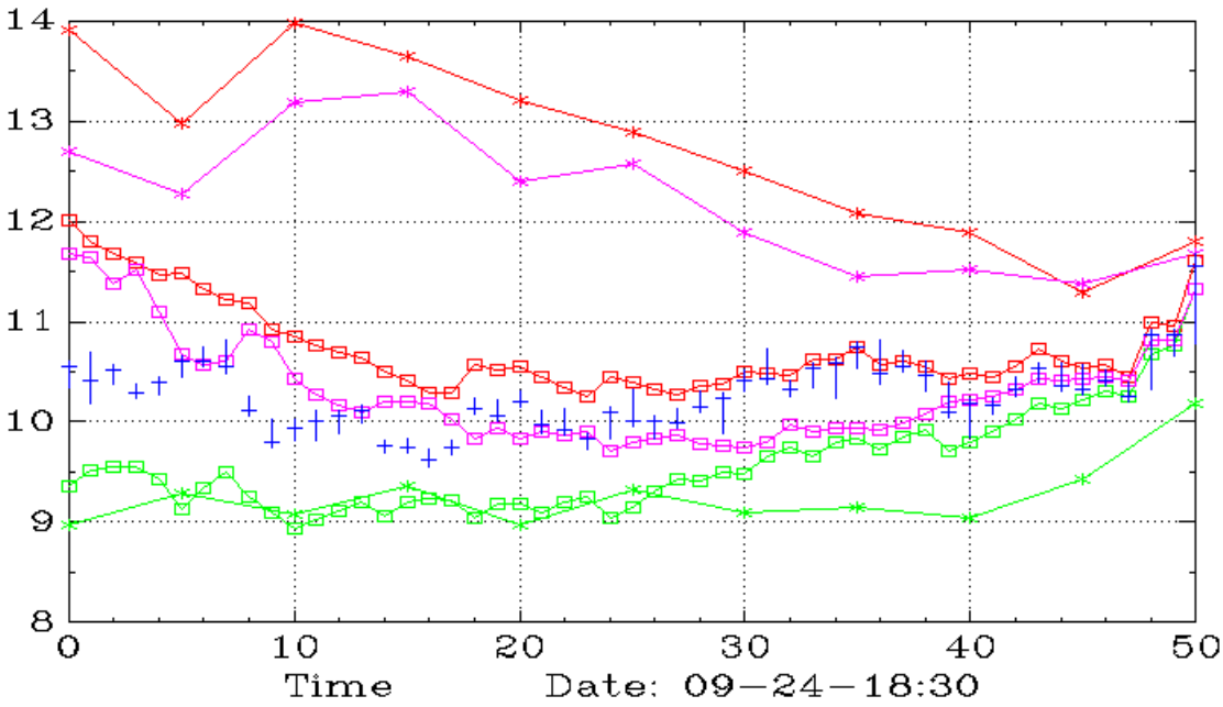
UNG (Weekly,Daily)
