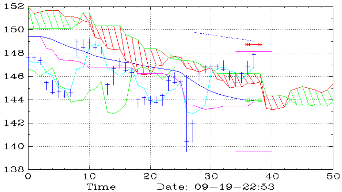
UPRO (90,Ichimoku)
