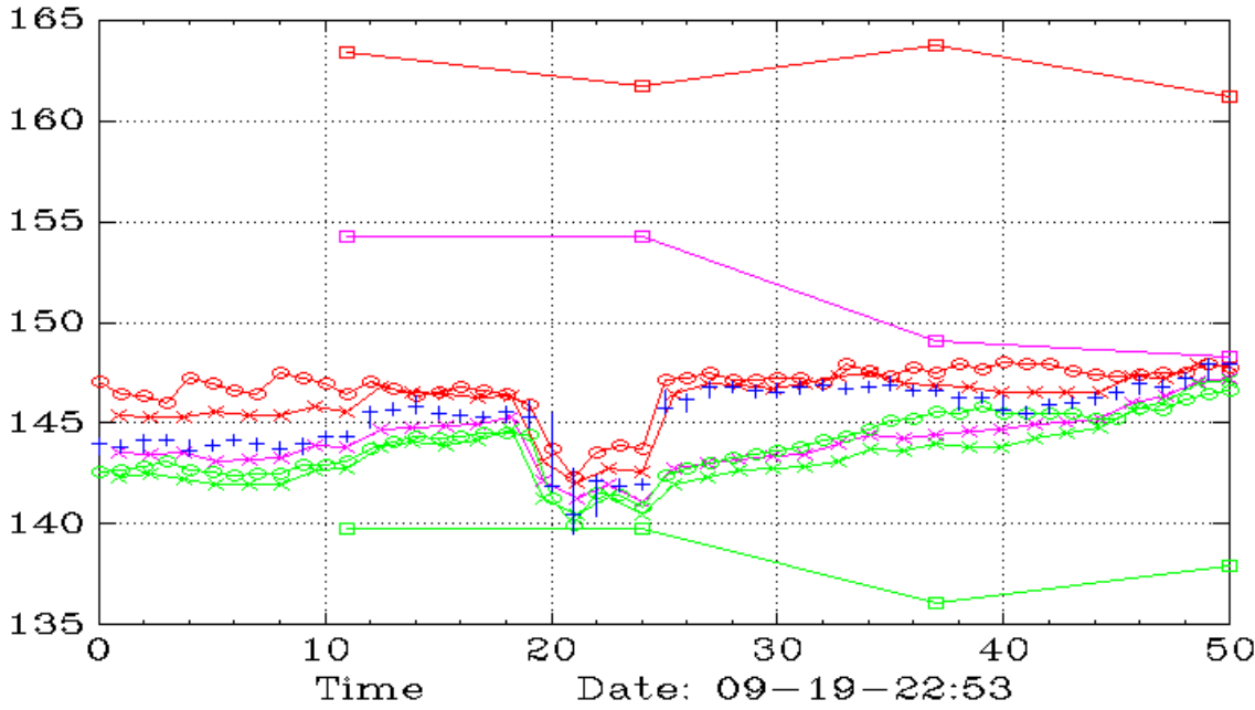
UPRO (Daily,45,30)
