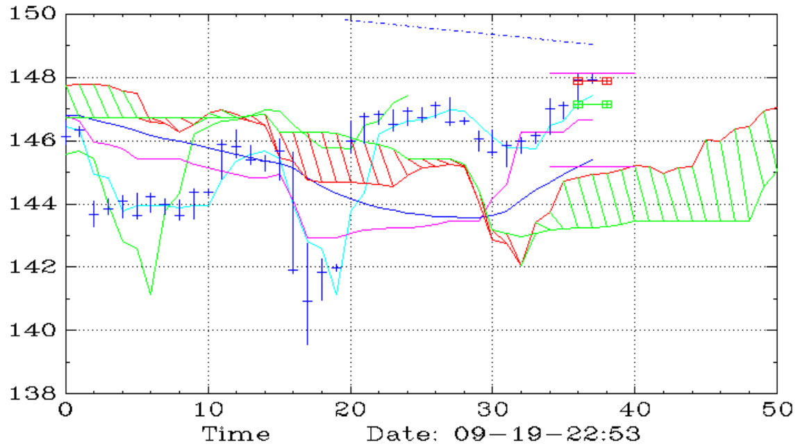
UPRO (45,Ichimoku)
