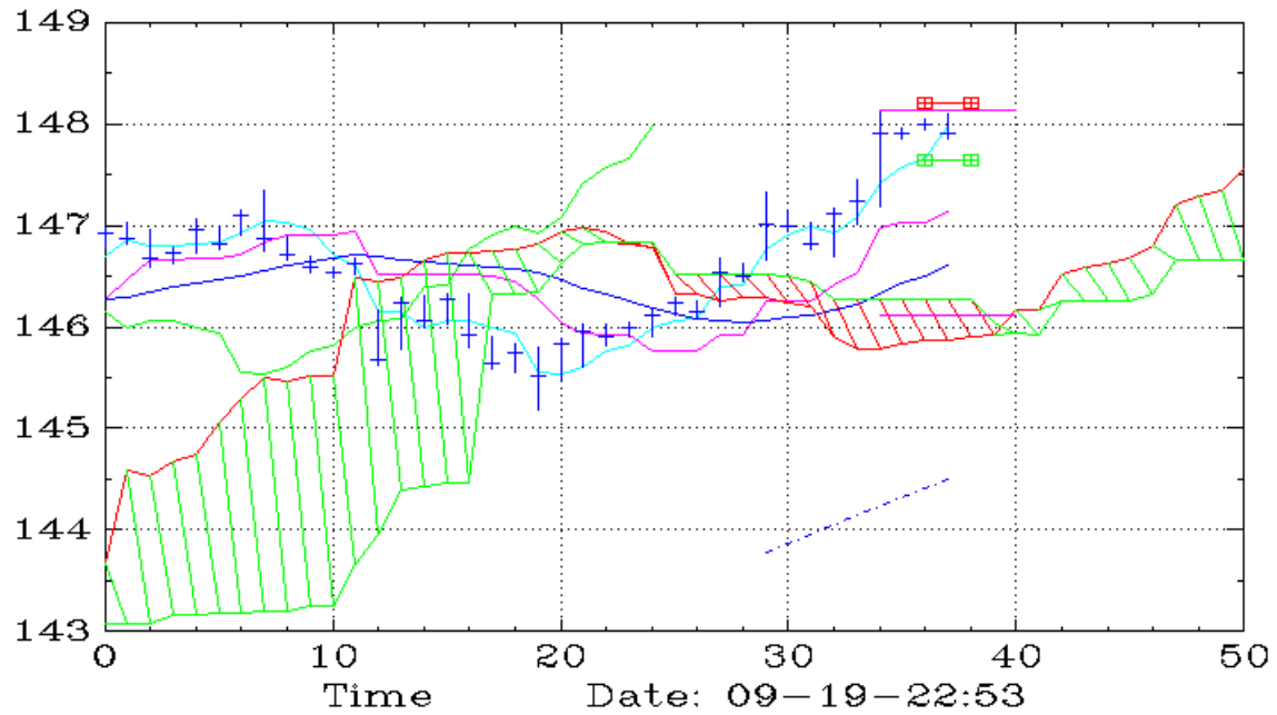
UPRO (15,Ichimoku)
