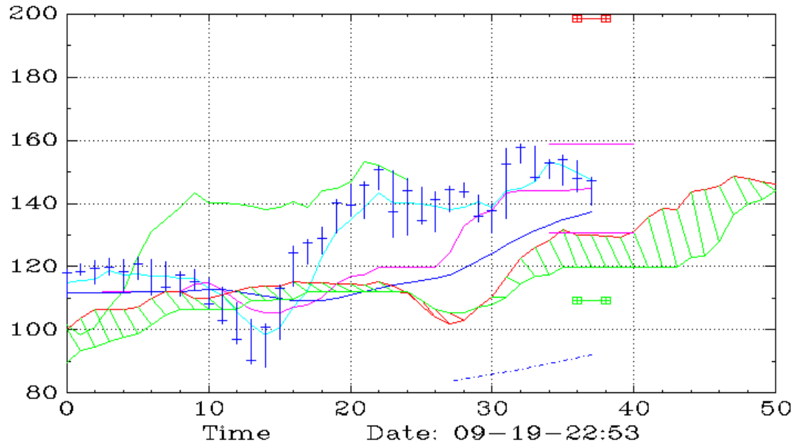
UPRO (Weekly,Ichimoku)
