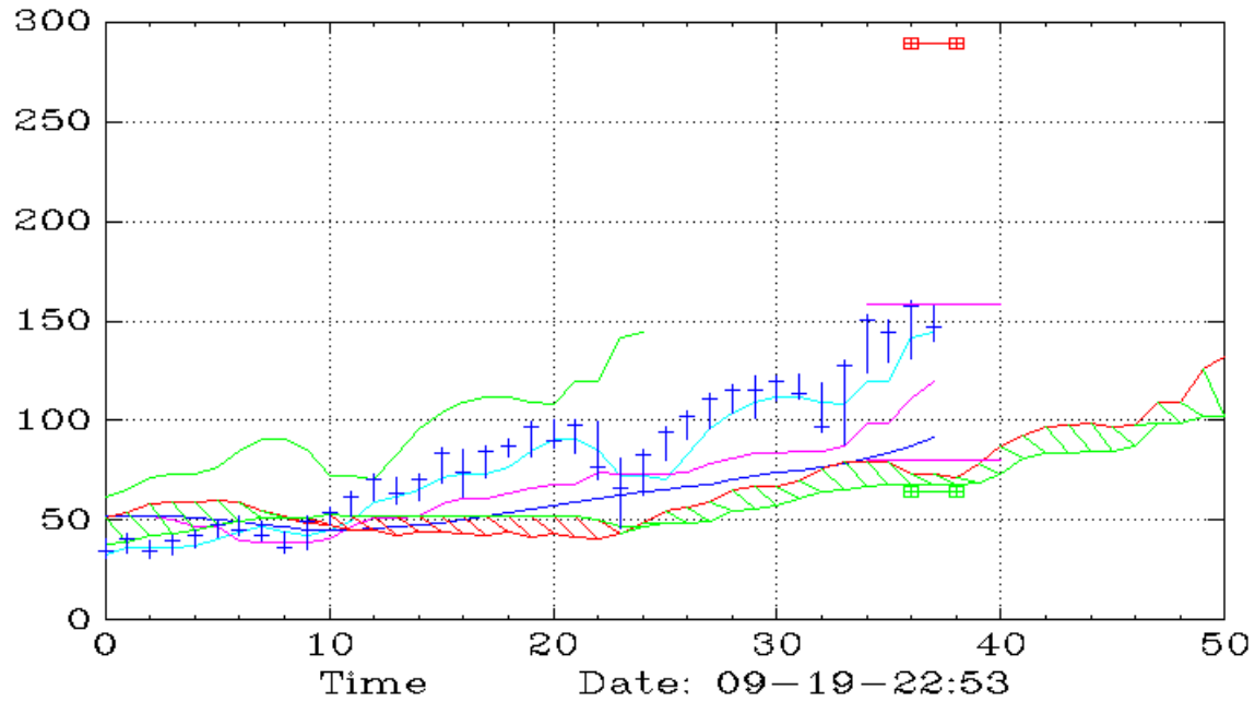
UPRO (Monthly,Ichimoku)
