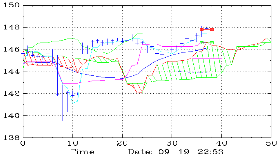
UPRO (30,Ichimoku)
