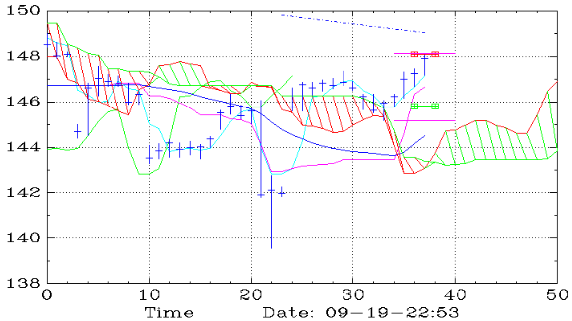
UPRO (60,Ichimoku)
