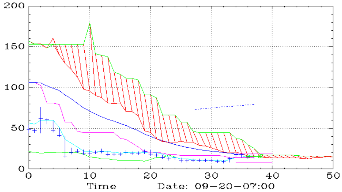
UXRP (Weekly,Ichimoku)
