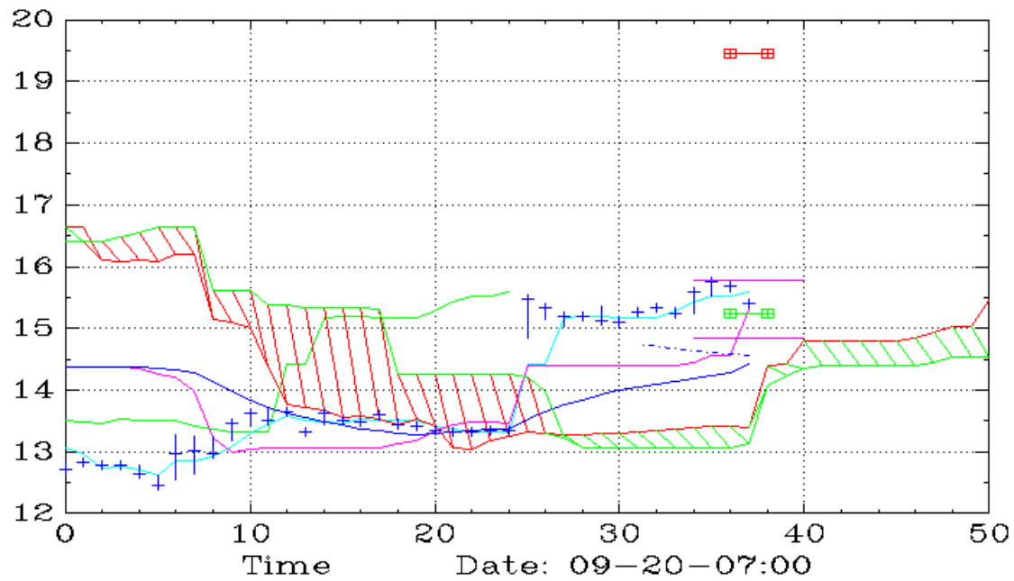
UXRP (30,Ichimoku)
