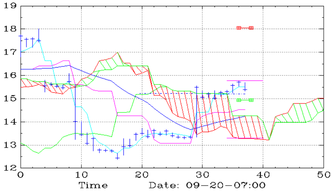
UXRP (45,Ichimoku)
