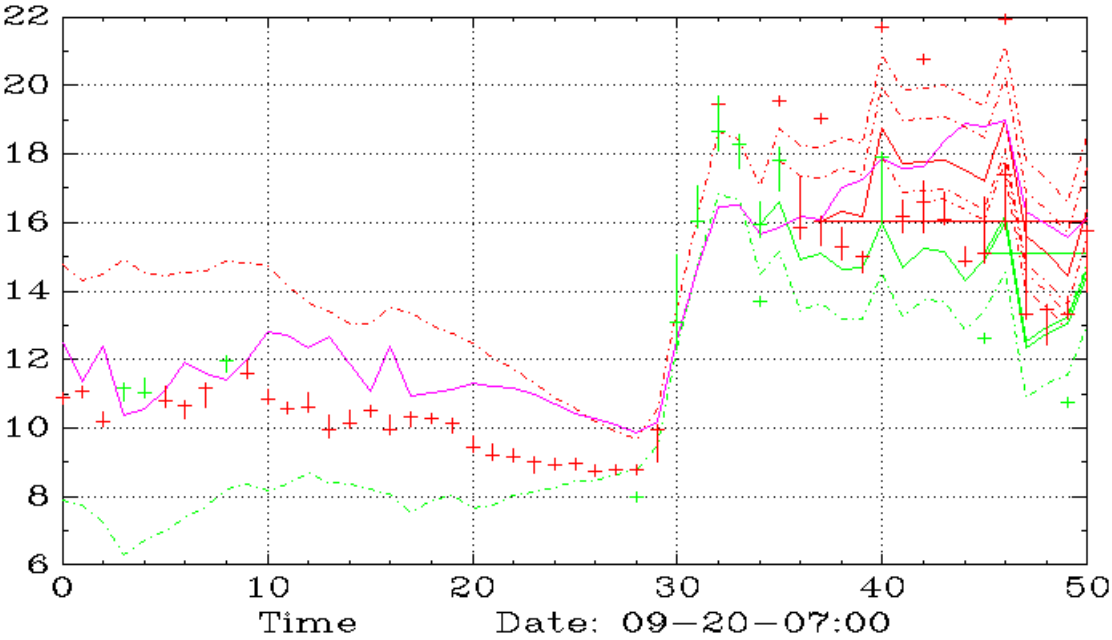
UXRP (Daily,SAR)
