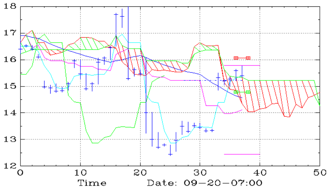
UXRP (90,Ichimoku)
