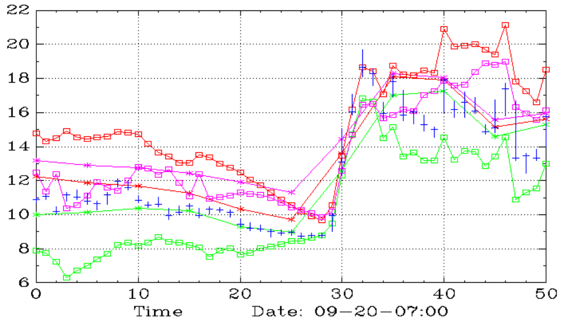
UXRP (Weekly,Daily)
