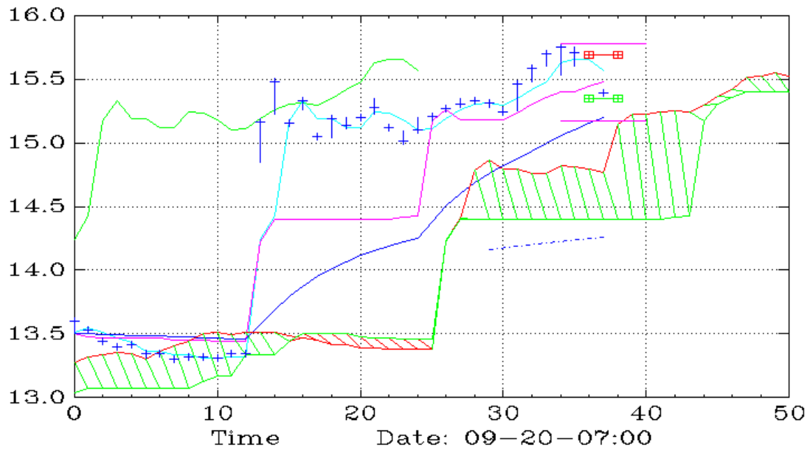
UXRP (15,Ichimoku)
