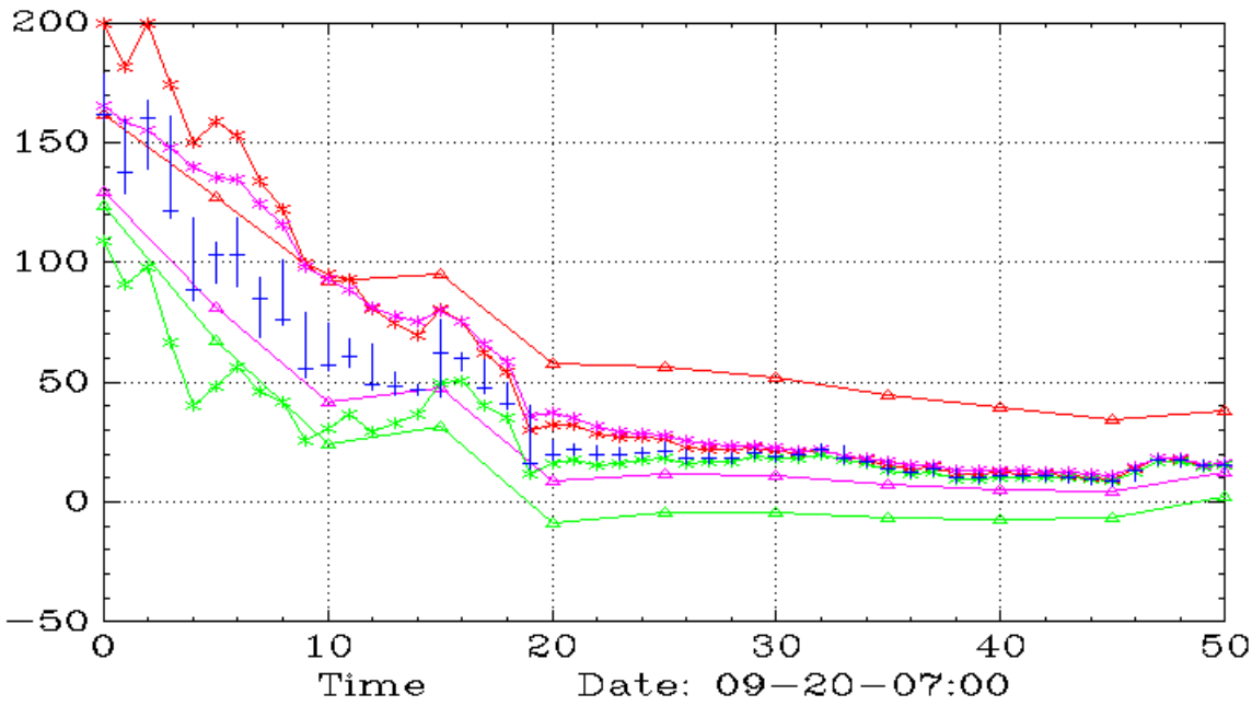
UXRP (Monthly,Weekly)
