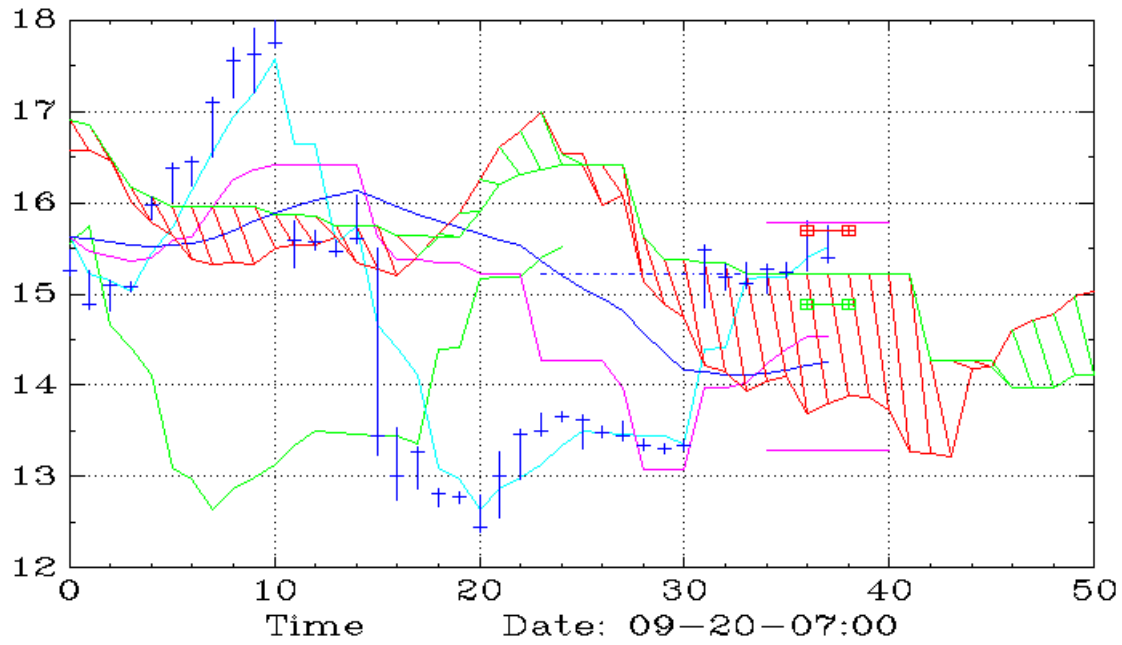
UXRP (60,Ichimoku)
