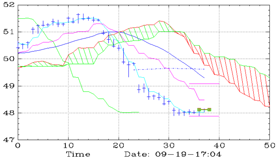
VZ (60,Ichimoku)
