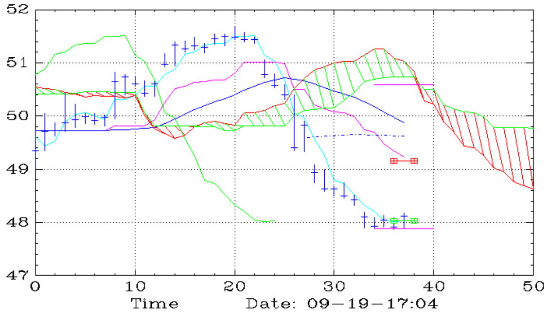
VZ (90,Ichimoku)
