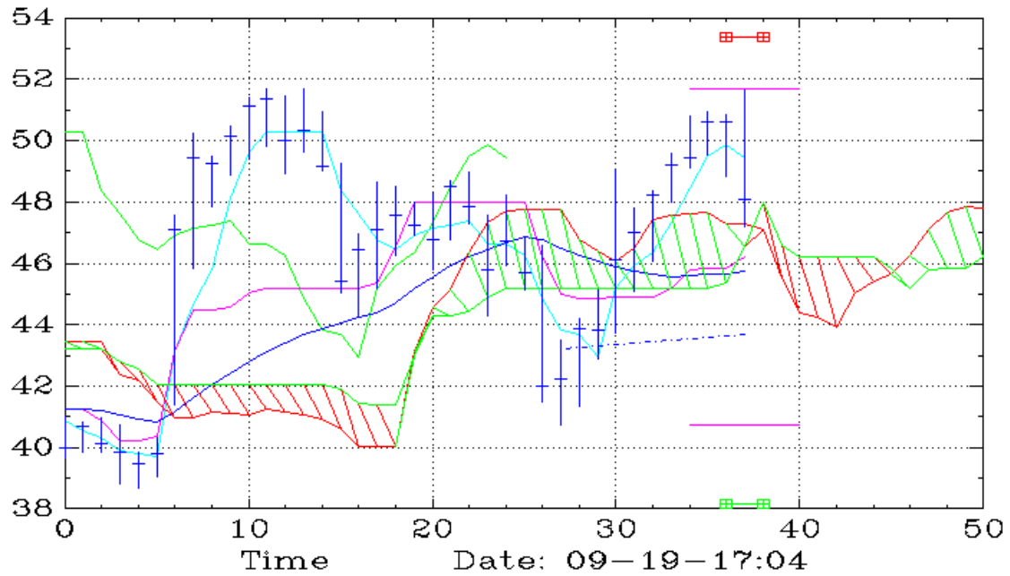
VZ (Weekly,Ichimoku)
