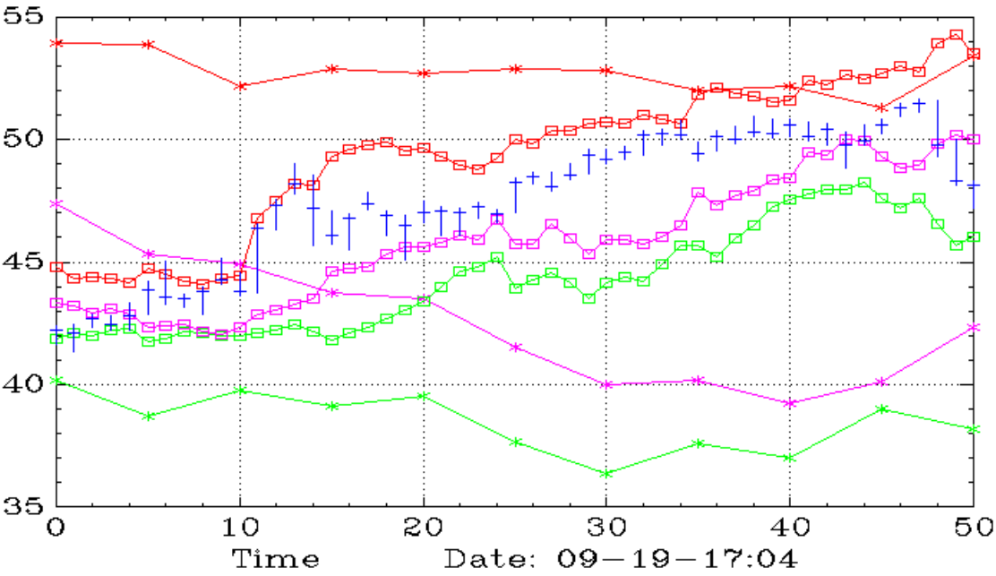
VZ (Weekly,Daily)
