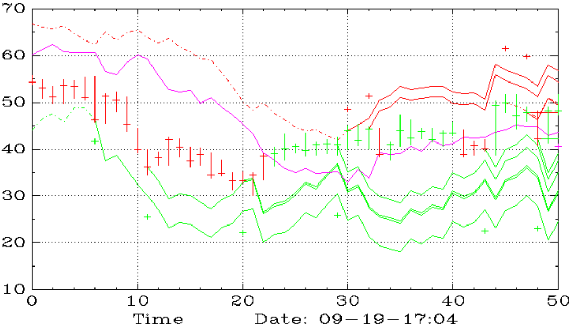
VZ (Monthly,SAR)
