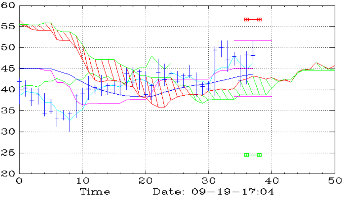
VZ (Monthly,Ichimoku)
