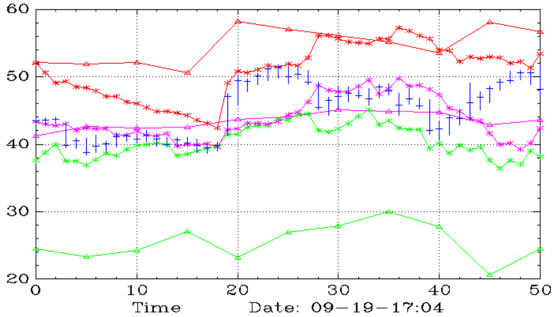
VZ (Monthly,Weekly)
