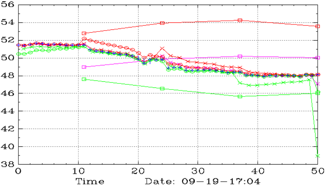
VZ (Daily,45,30)
