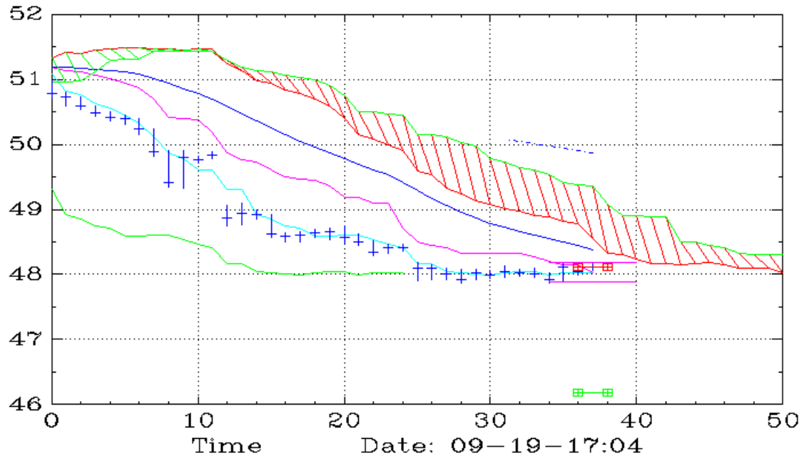
VZ (30,Ichimoku)
