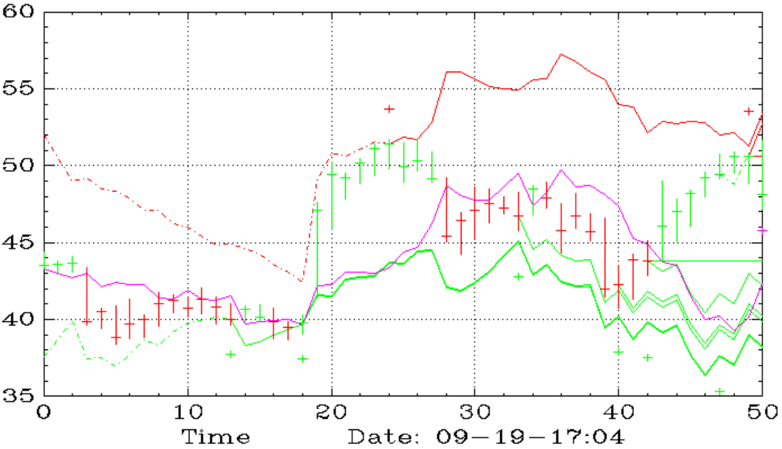
VZ (Weekly,SAR)
