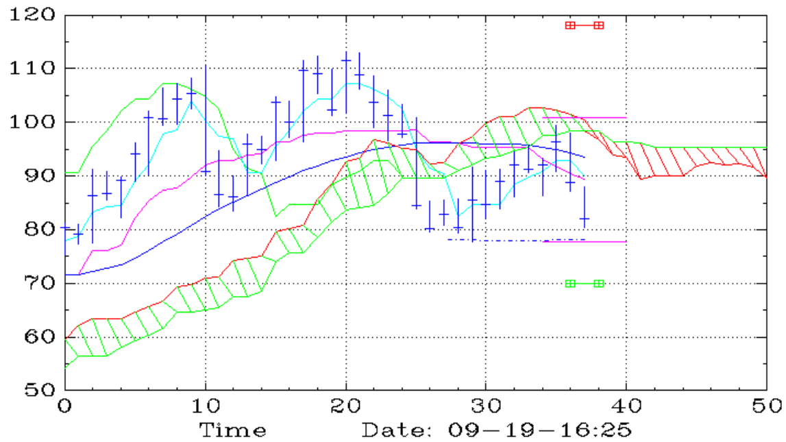
WFRD (Weekly,Ichimoku)
