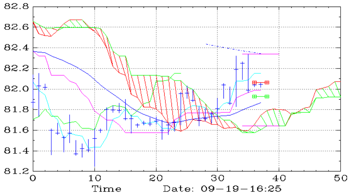
WFRD (10,Ichimoku)
