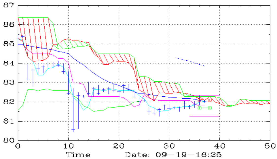
WFRD (30,Ichimoku)
