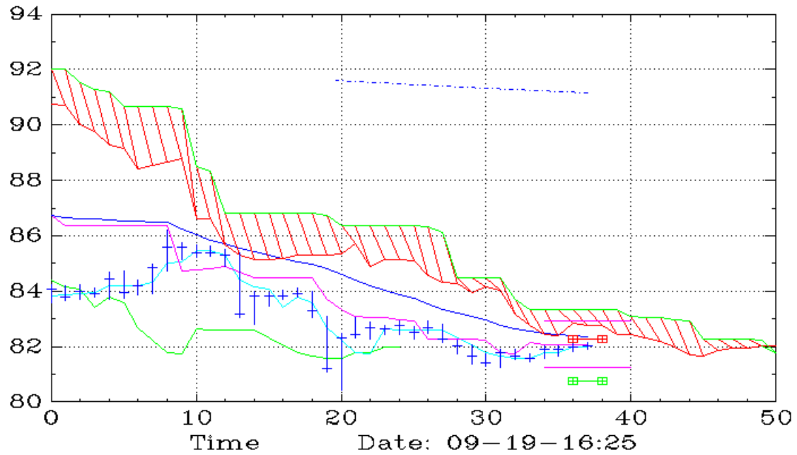
WFRD (45,Ichimoku)
