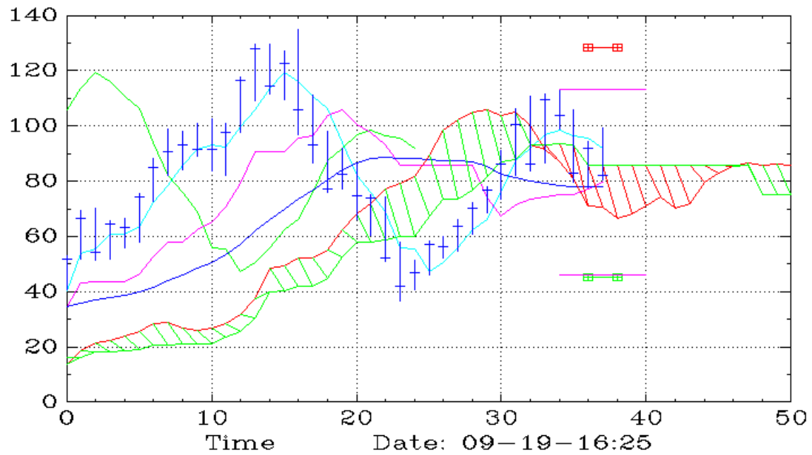
WFRD (Monthly,Ichimoku)
