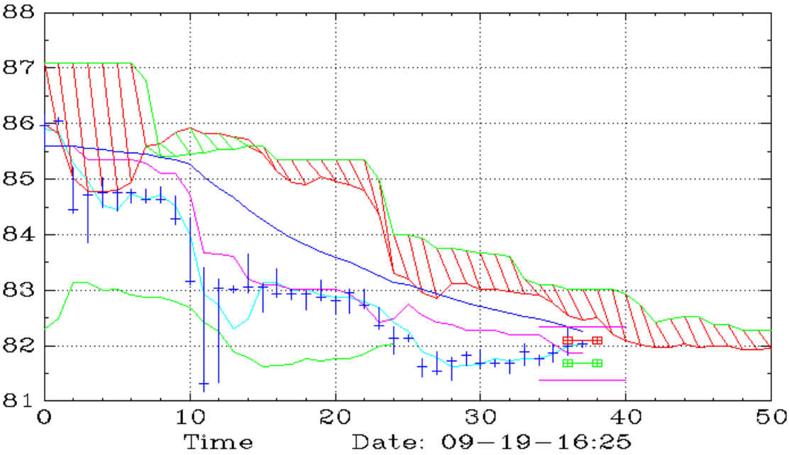
WFRD (30,VAP_Ichimoku)
