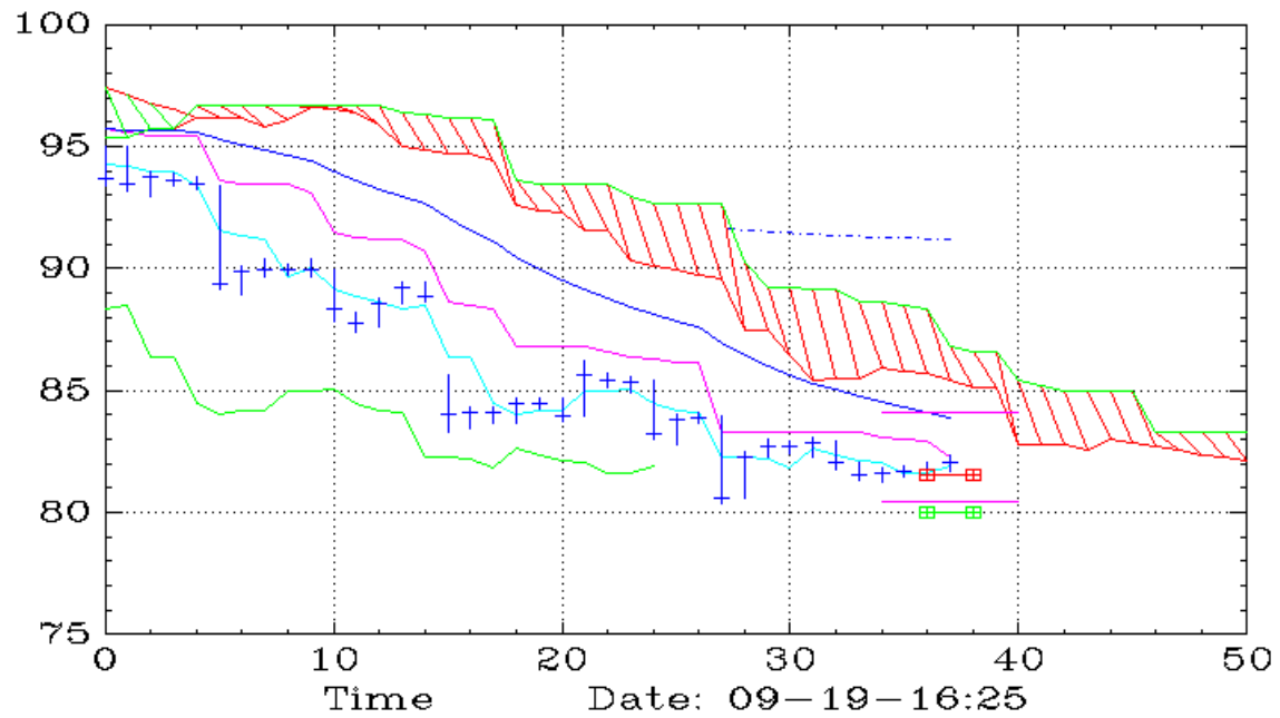
WFRD (90,Ichimoku)
