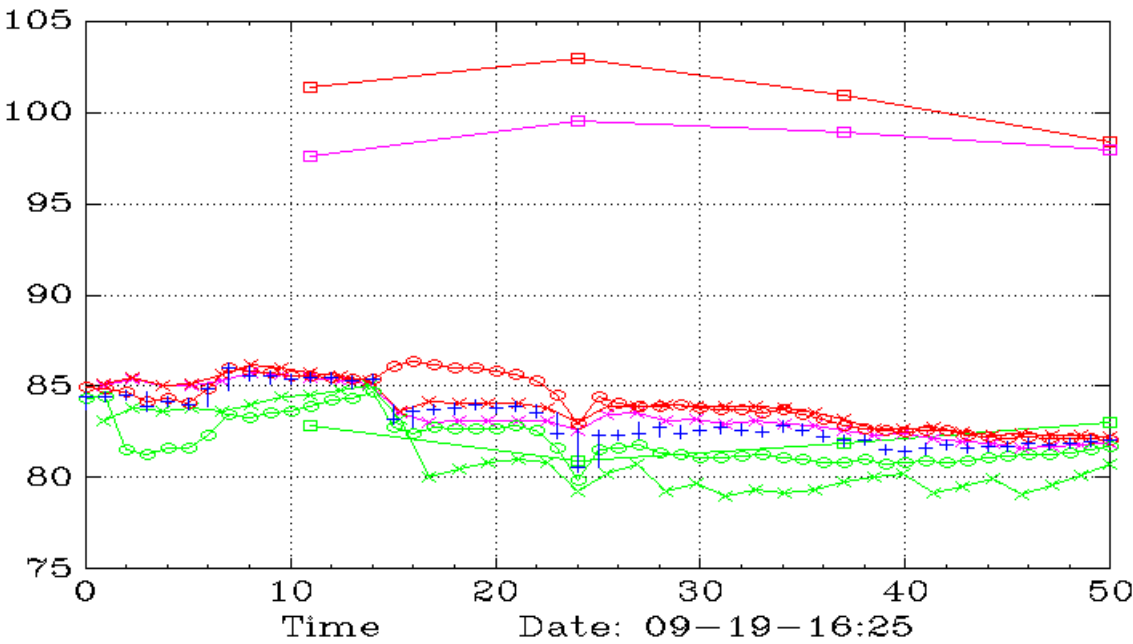
WFRD (Daily,45,30)
