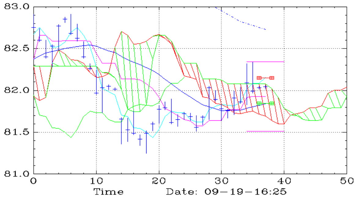
WFRD (15,Ichimoku)
