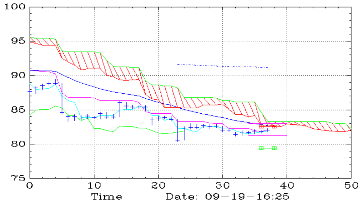
WFRD (60,Ichimoku)
