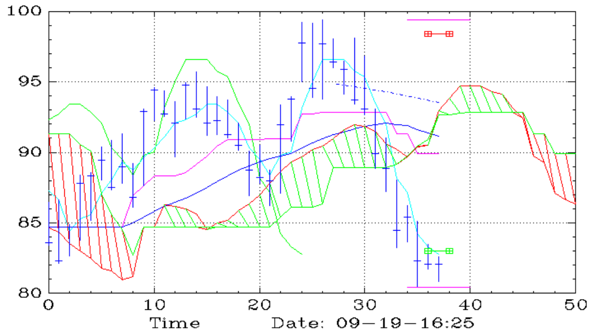
WFRD (Daily,Ichimoku)
