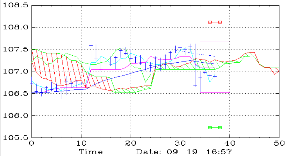
WMT (15,Ichimoku)
