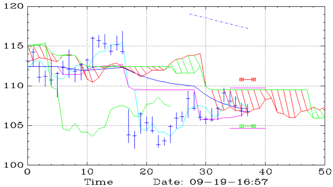
WMT (Daily,Ichimoku)
