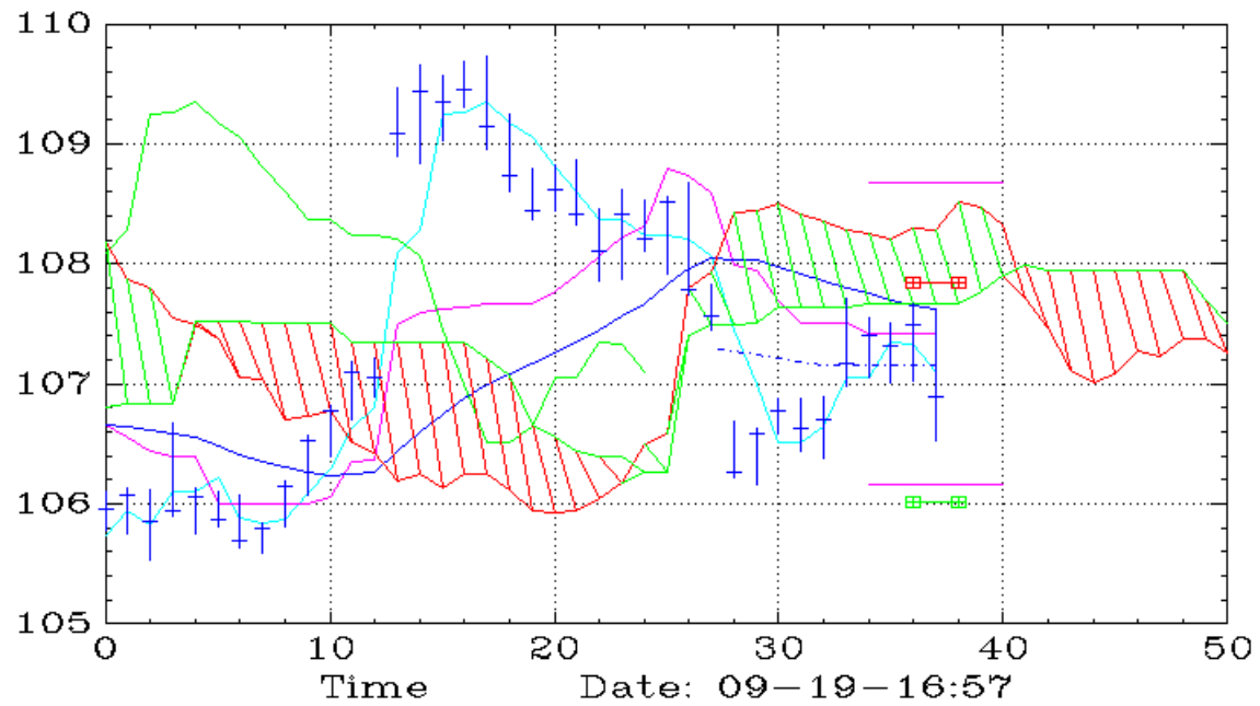
WMT (90,Ichimoku)
