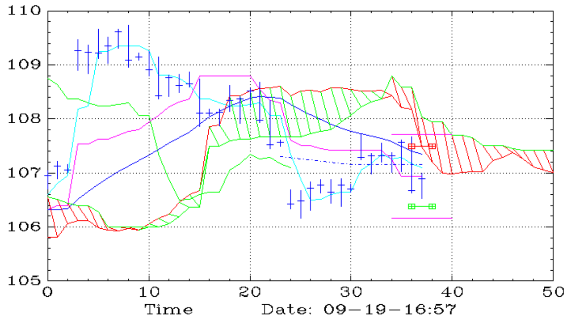
WMT (60,Ichimoku)
