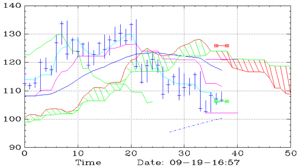
WMT (Weekly,Ichimoku)
