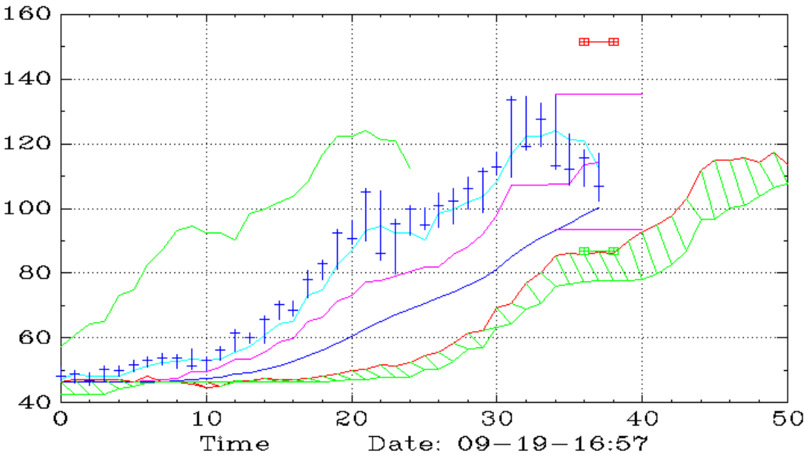
WMT (Monthly,Ichimoku)
