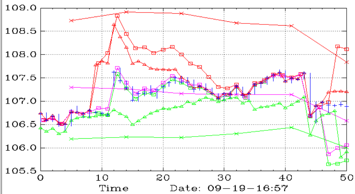
WMT (90,15,10)
