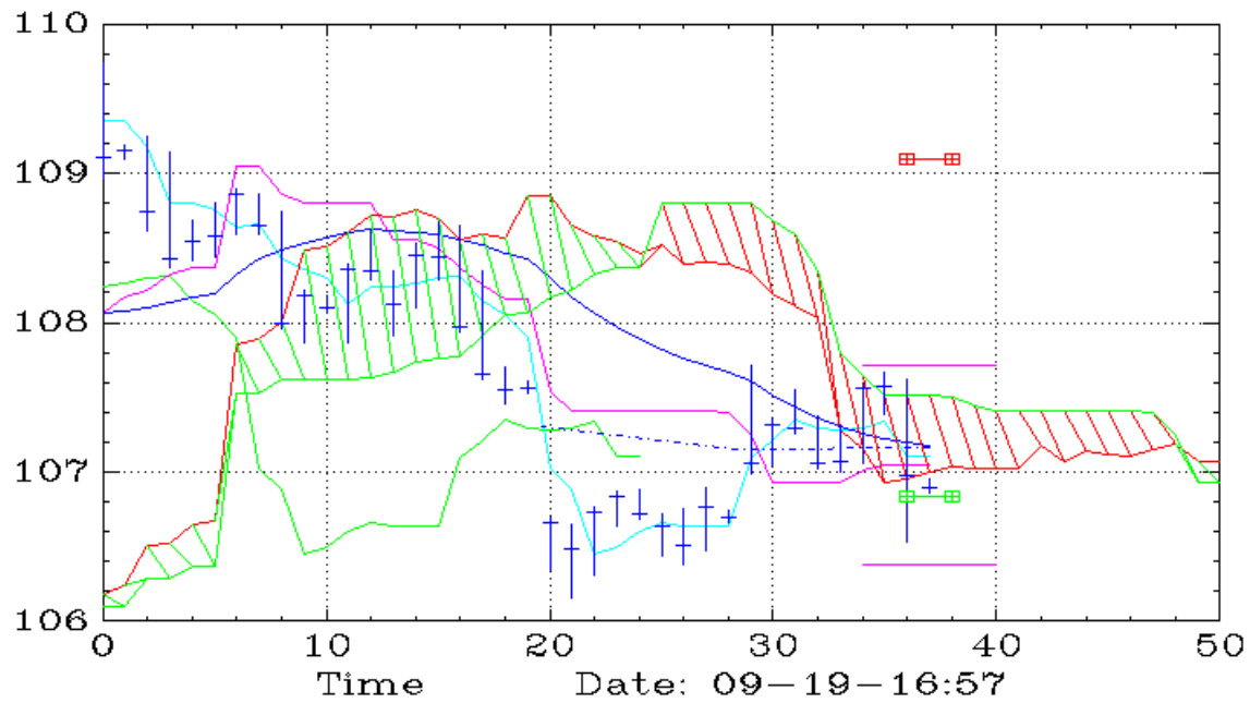
WMT (45,Ichimoku)
