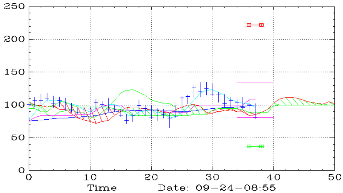
WYNN (Monthly,Ichimoku)
