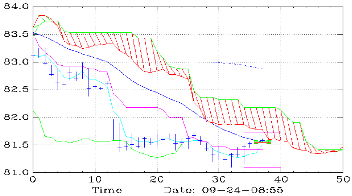
WYNN (15,Ichimoku)
