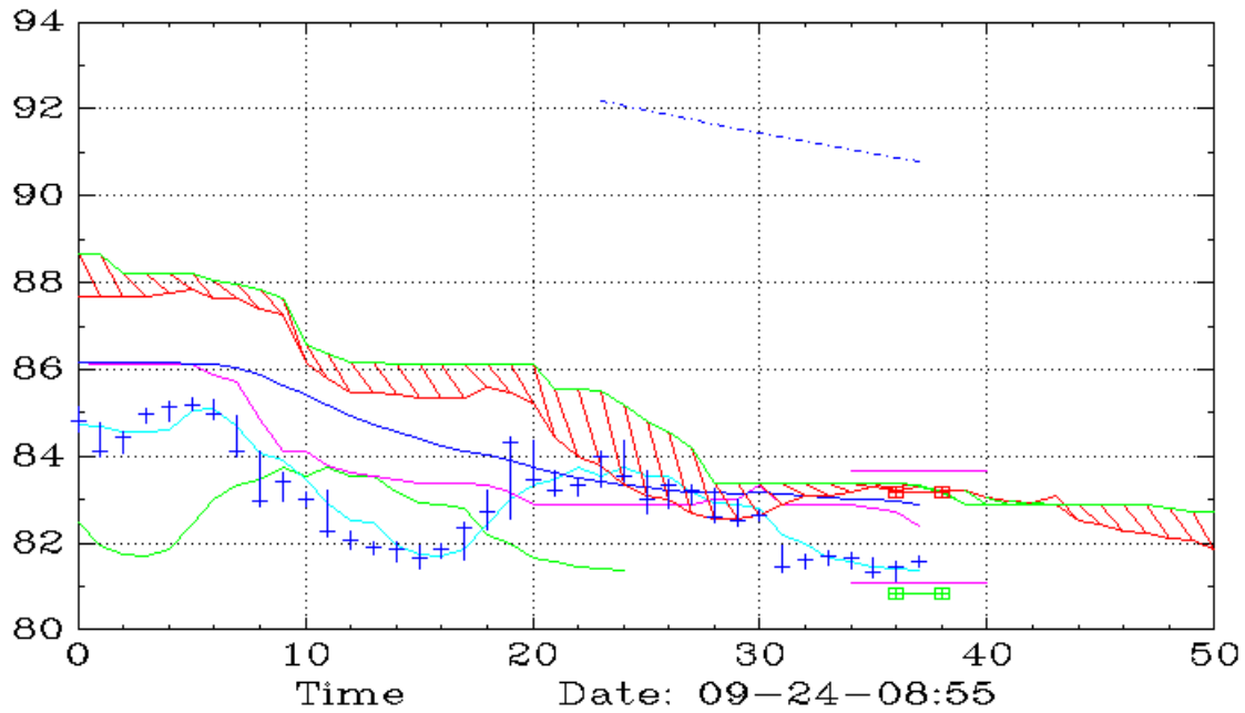
WYNN (60,Ichimoku)
