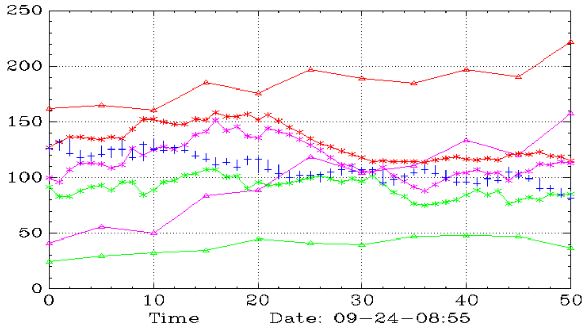
WYNN (Monthly,Weekly)
