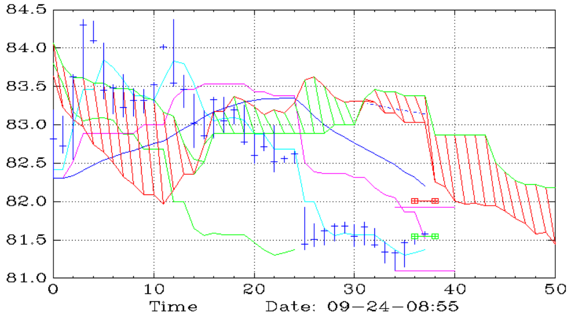
WYNN (30,Ichimoku)
