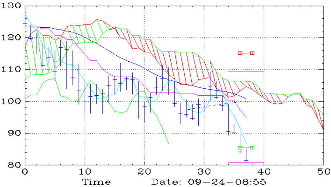
WYNN (Weekly,Ichimoku)
