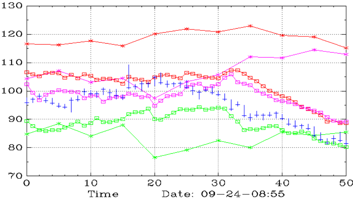
WYNN (Weekly,Daily)
