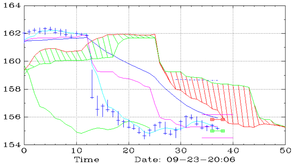
XBI (15,Ichimoku)
