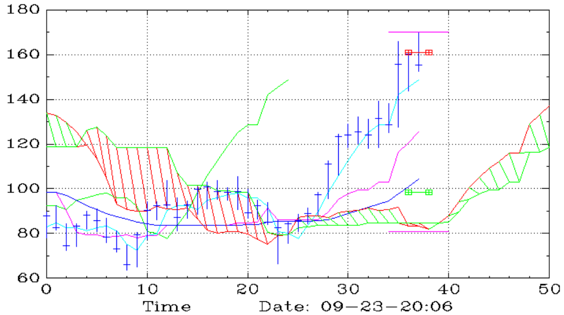
XBI (Monthly,Ichimoku)
