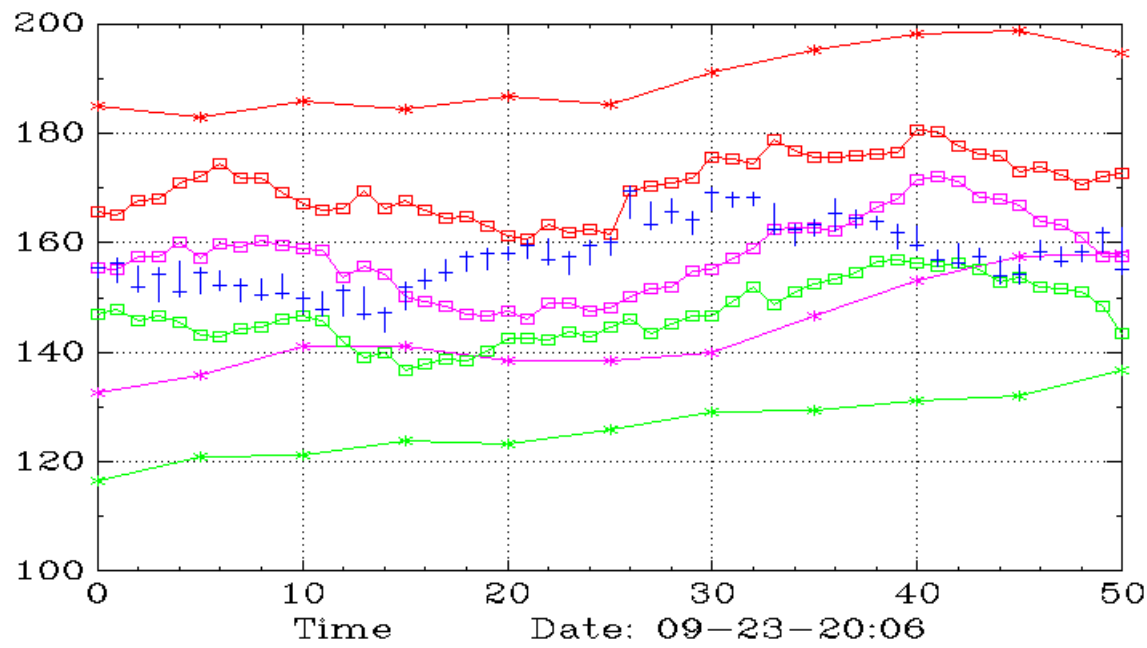
XBI (Weekly,Daily)
