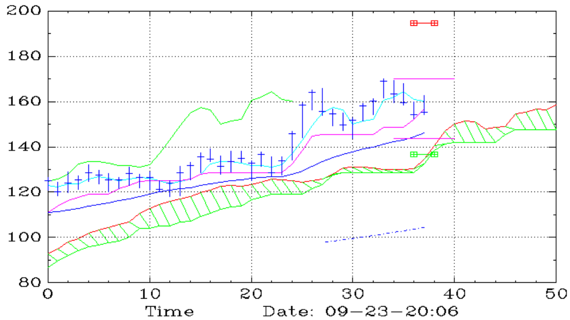
XBI (Weekly,Ichimoku)
