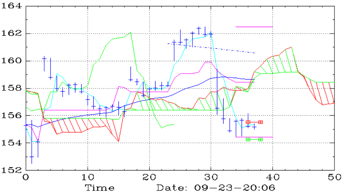
XBI (60,Ichimoku)
