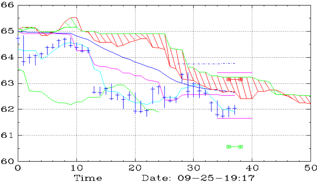
XLE (90,Ichimoku)
