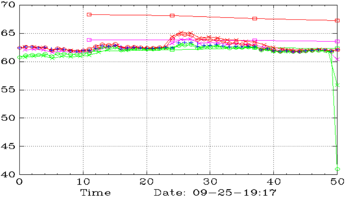
XLE (Daily,45,30)
