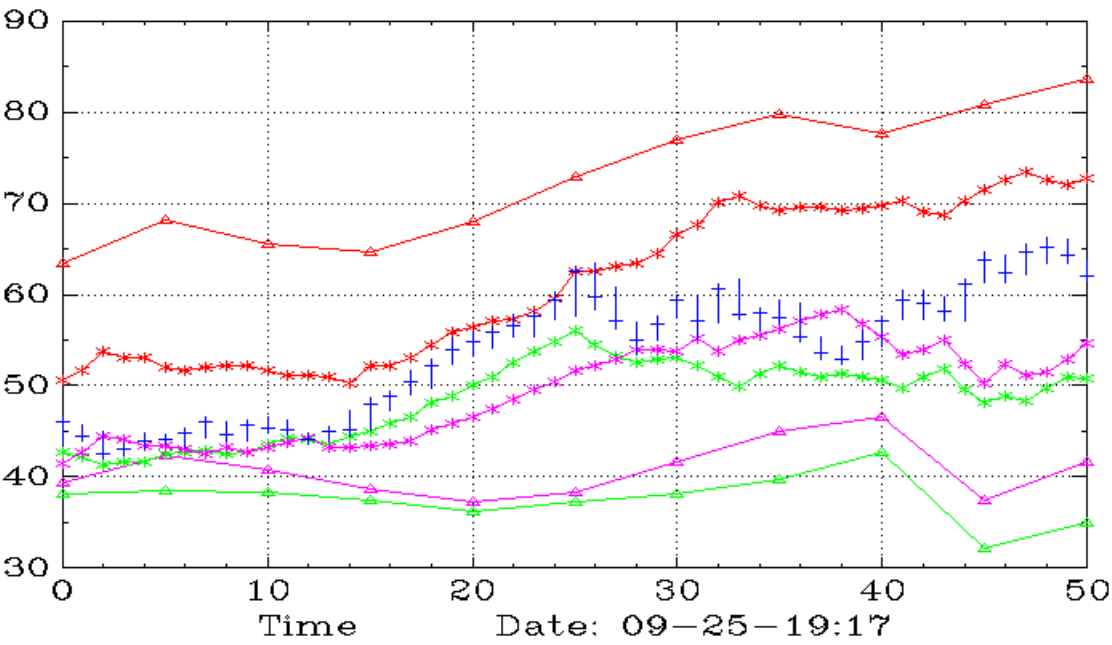
XLE (Monthly,Weekly)
