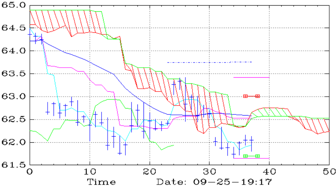
XLE (60,Ichimoku)
