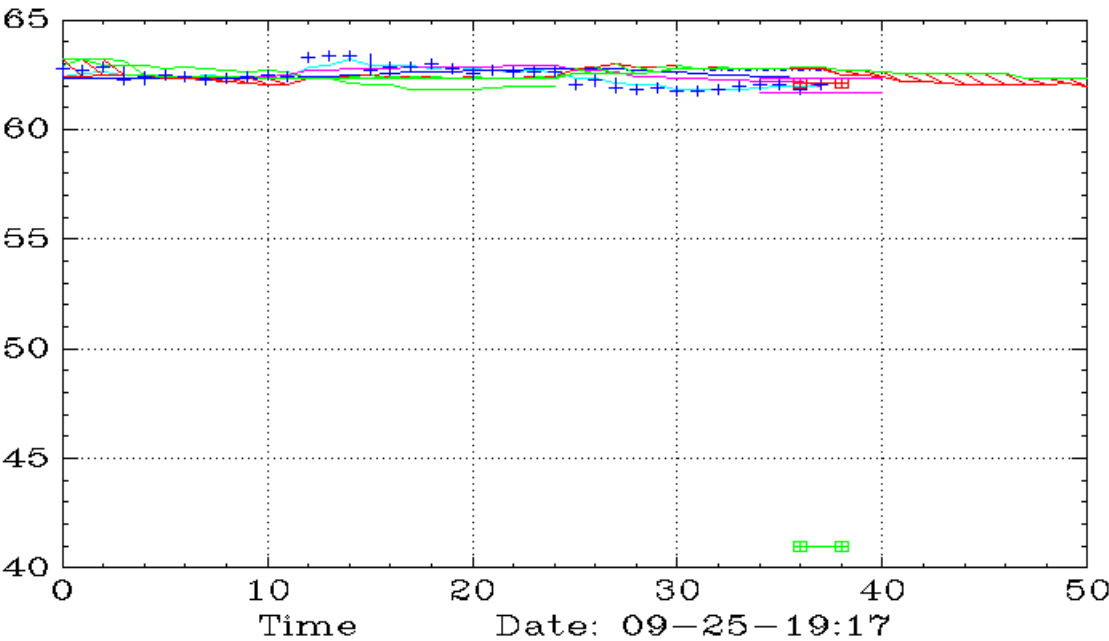
XLE (30,Ichimoku)
