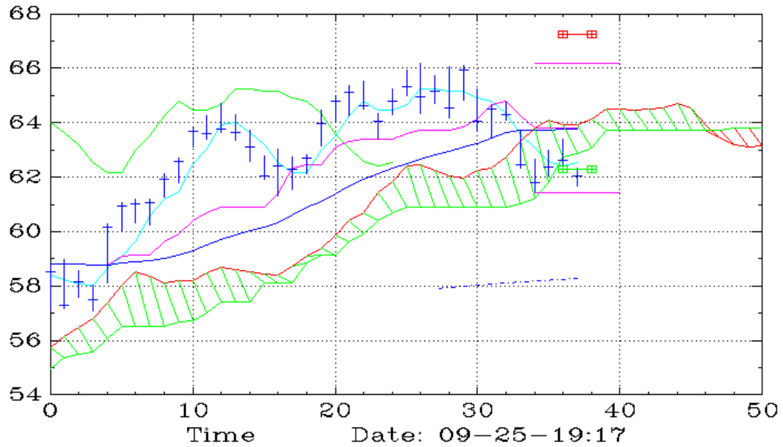
XLE (Daily,Ichimoku)
