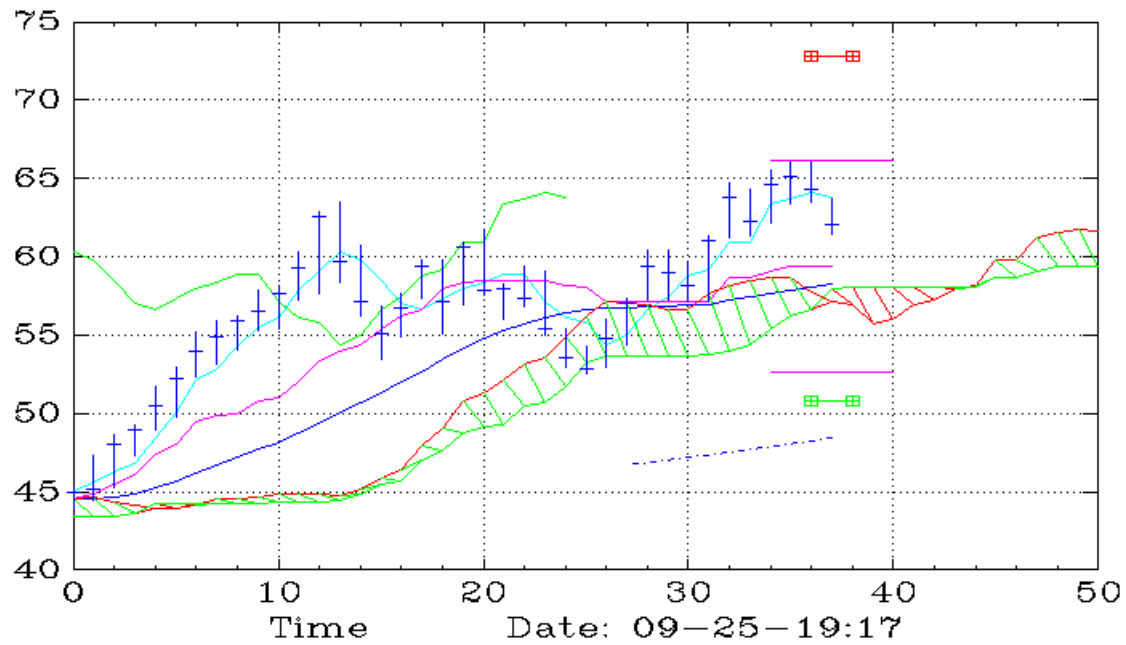
XLE (Weekly,Ichimoku)
