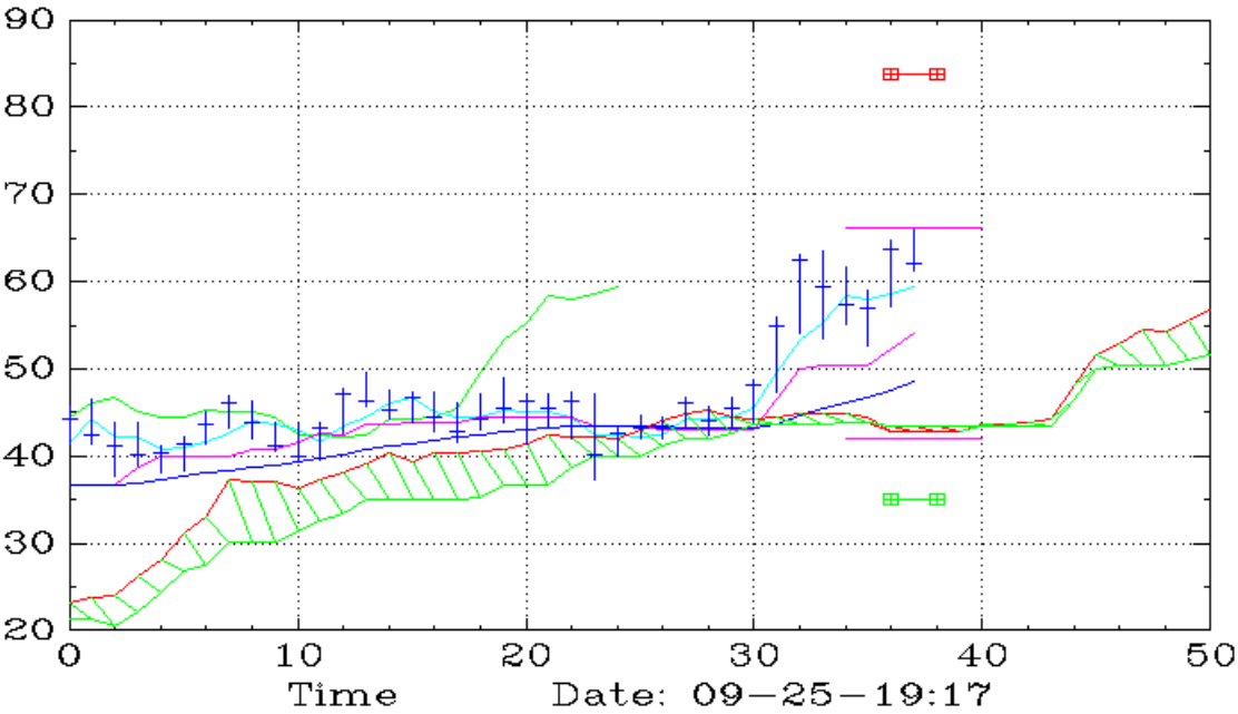
XLE (Monthly,Ichimoku)
