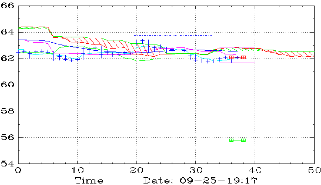
XLE (45,Ichimoku)
