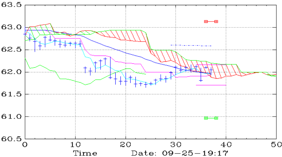
XLE (15,Ichimoku)
