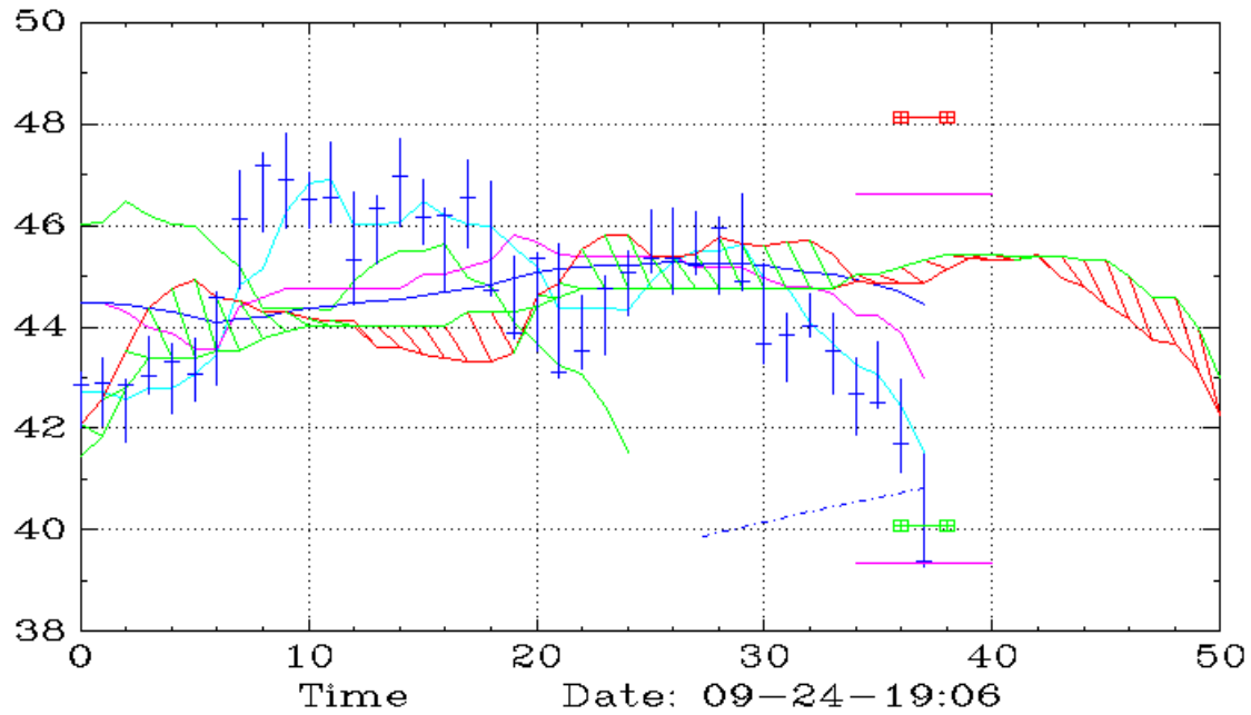
XLU (Weekly,Ichimoku)
