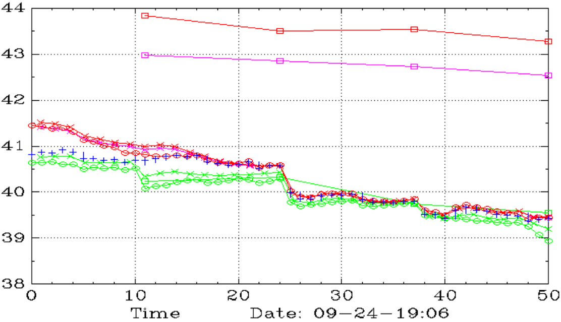
XLU (Daily,45,30)
