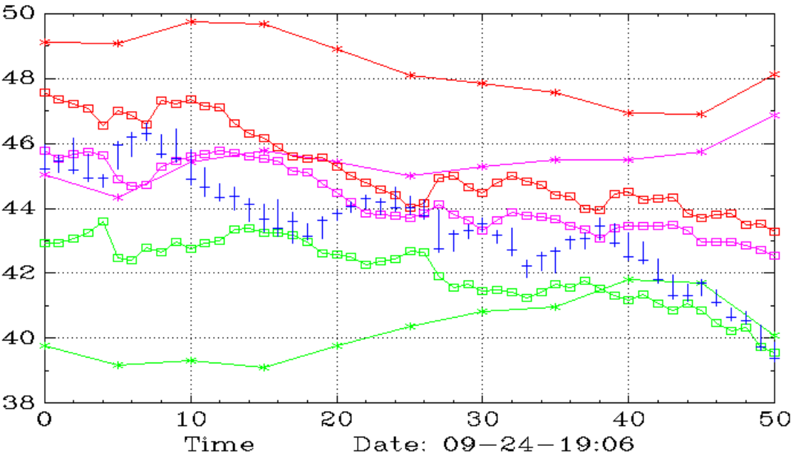
XLU (Weekly,Daily)
