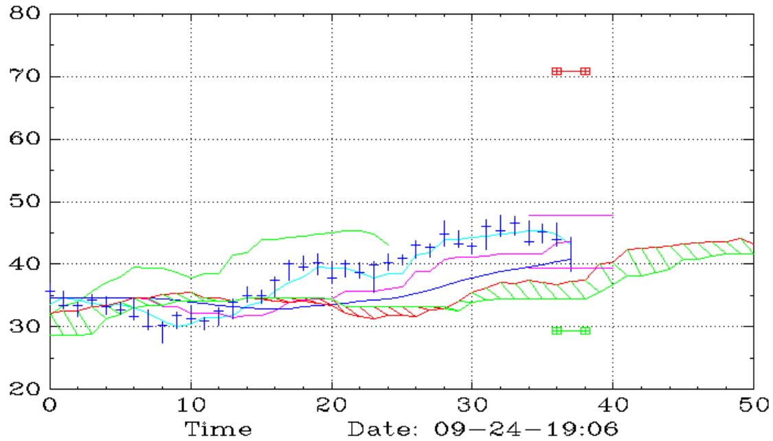
XLU (Monthly,Ichimoku)
