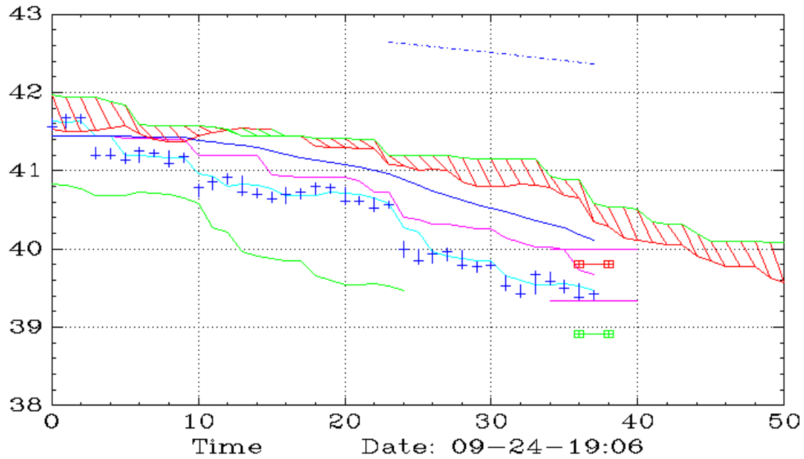
XLU (60,Ichimoku)
