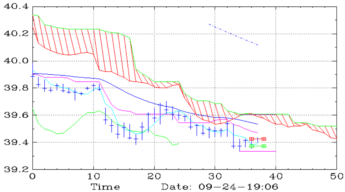
XLU (15,Ichimoku)
