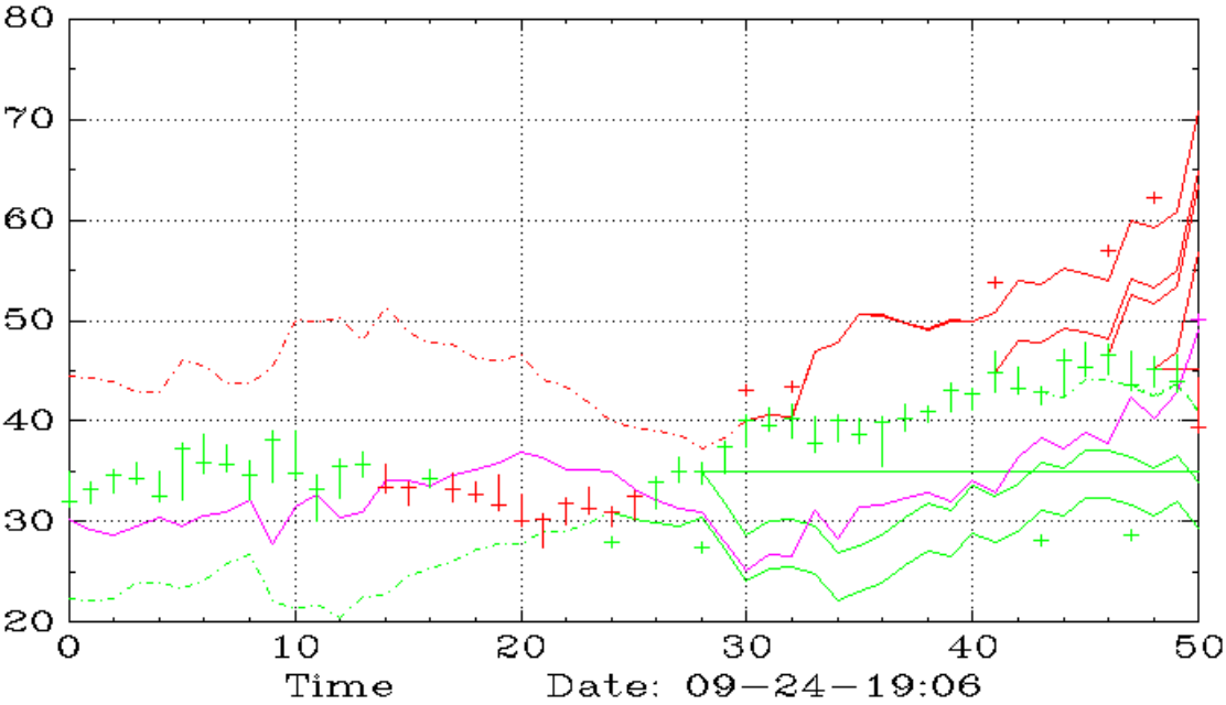
XLU (Monthly,SAR)
