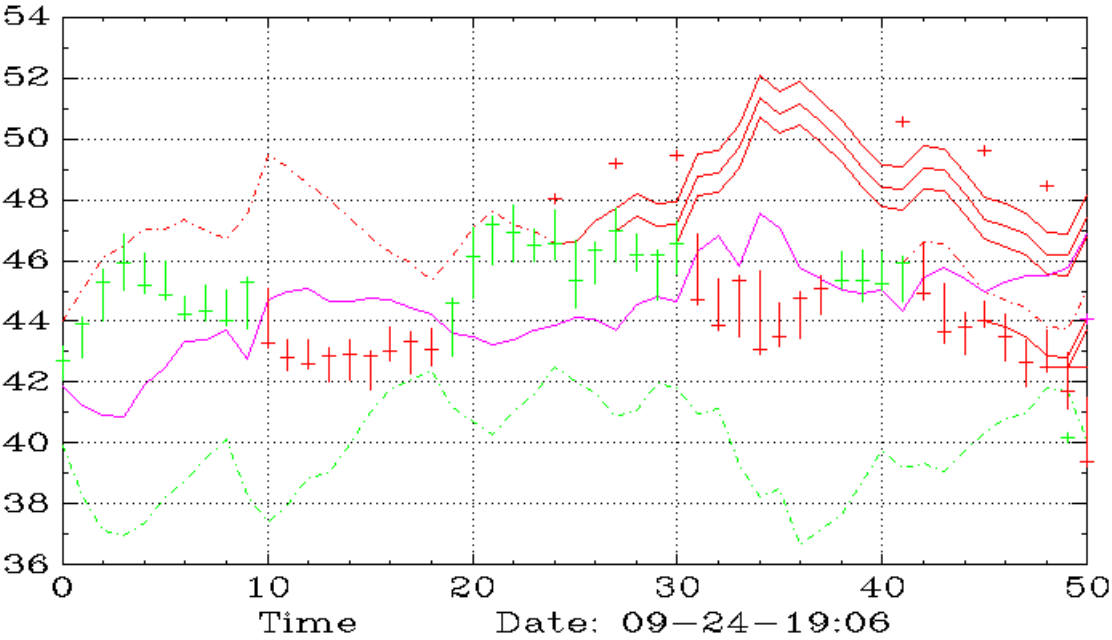
XLU (Weekly,SAR)
