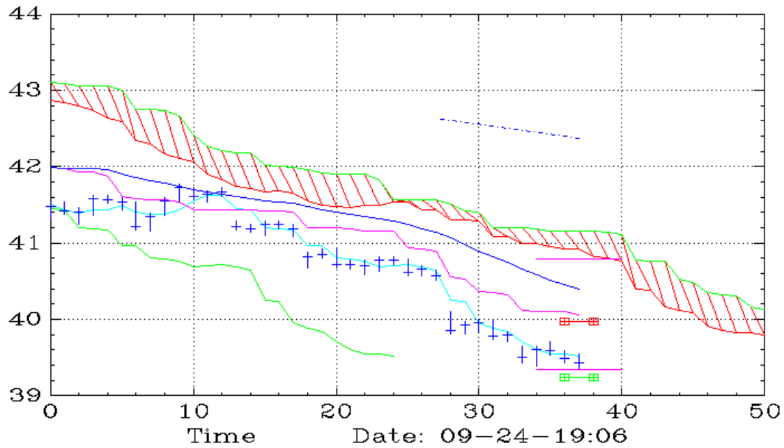
XLU (90,Ichimoku)
